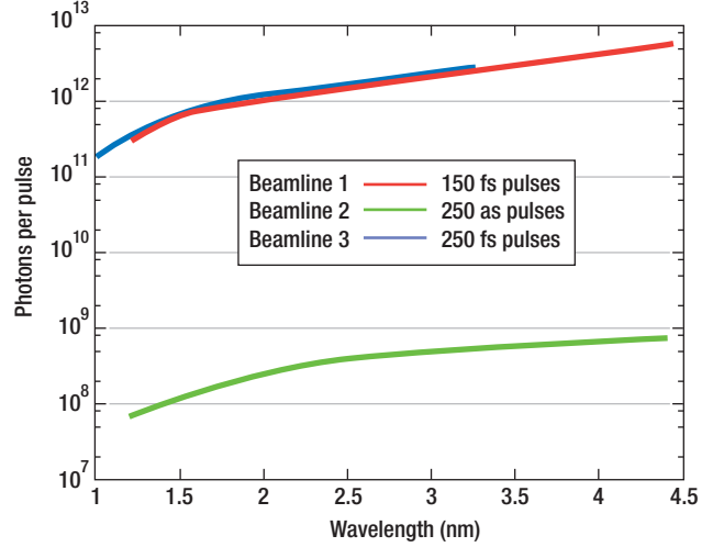
Figure 2: Beamline 1 is a seeded FEL shown here for 150 fs pulse duration; Beamline 2 is a 2-color attosecond beamline, here with 250 as pulses; Beamline 3 is a SASE FEL here with 250 fs pulses.
