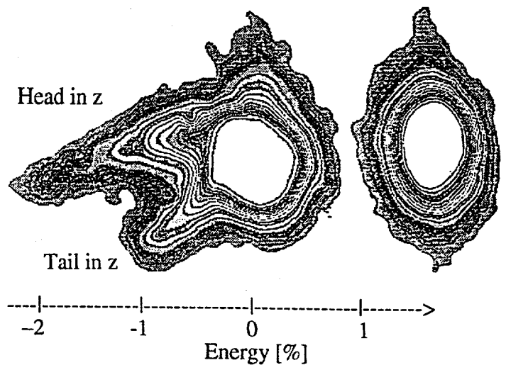
Figure 5: Beam Distributions at a Dispersive Point
