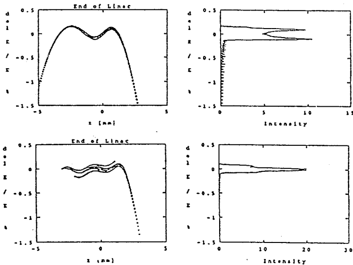
Figure 4: Energy versus z Distribution on the Linac RF and Energy Distribution
