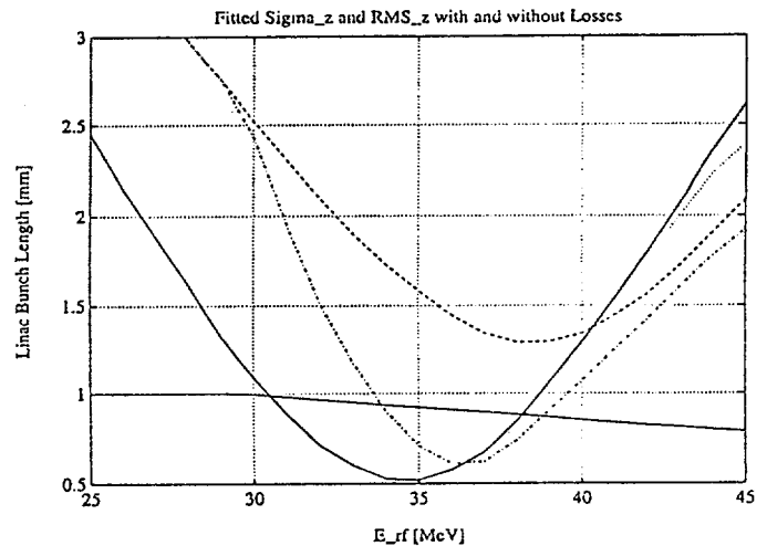
Figure 3: Bunch Length versus Compressor Amplitude
