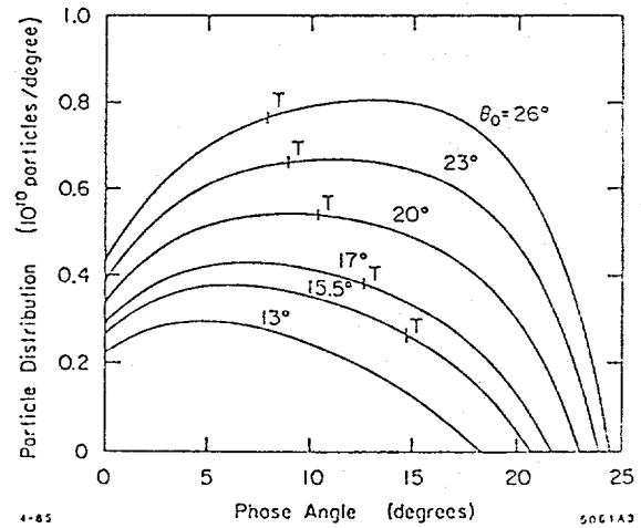
Figure 1: Linac Bunch Distributions [3]
