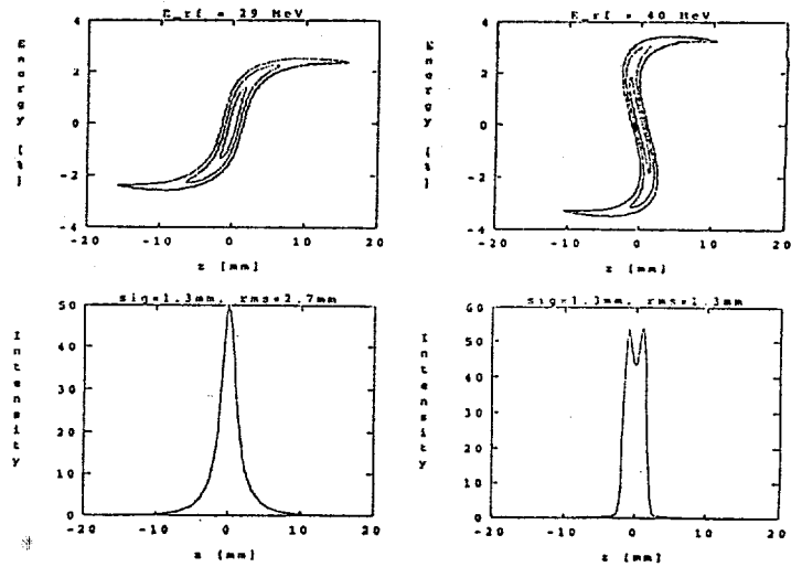
Figure 2: Under- and Over-Compression of the RTL Bunch Length
