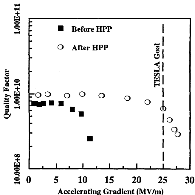
Fig. 3 Results of high power pulsed processing (HPP) of a 5 cell, 1.3 GHz superconducting cavity. Processing was performed with a peak field of 90 MV/m. 18
