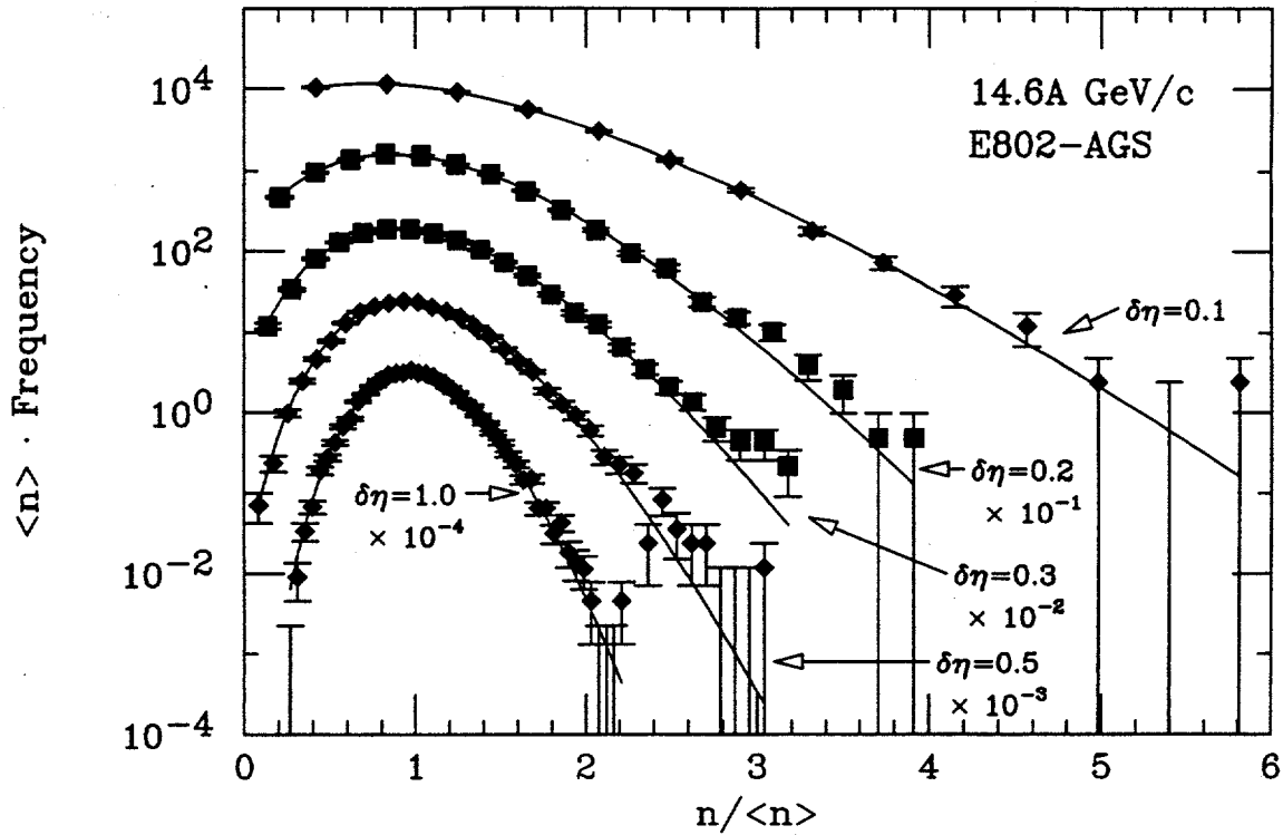
Figure 1: Multiplicity distributions for selected \delta\eta intervals, 0.1, 0.2, 0.3, 0.5, 1.0, as indicated. The data for each interval are plotted scaled in multiplicity by \langle n \rangle , the mean multiplicity in the interval. Each successive distribution has been normalized by the factor indicated, for clarity of presentation.
