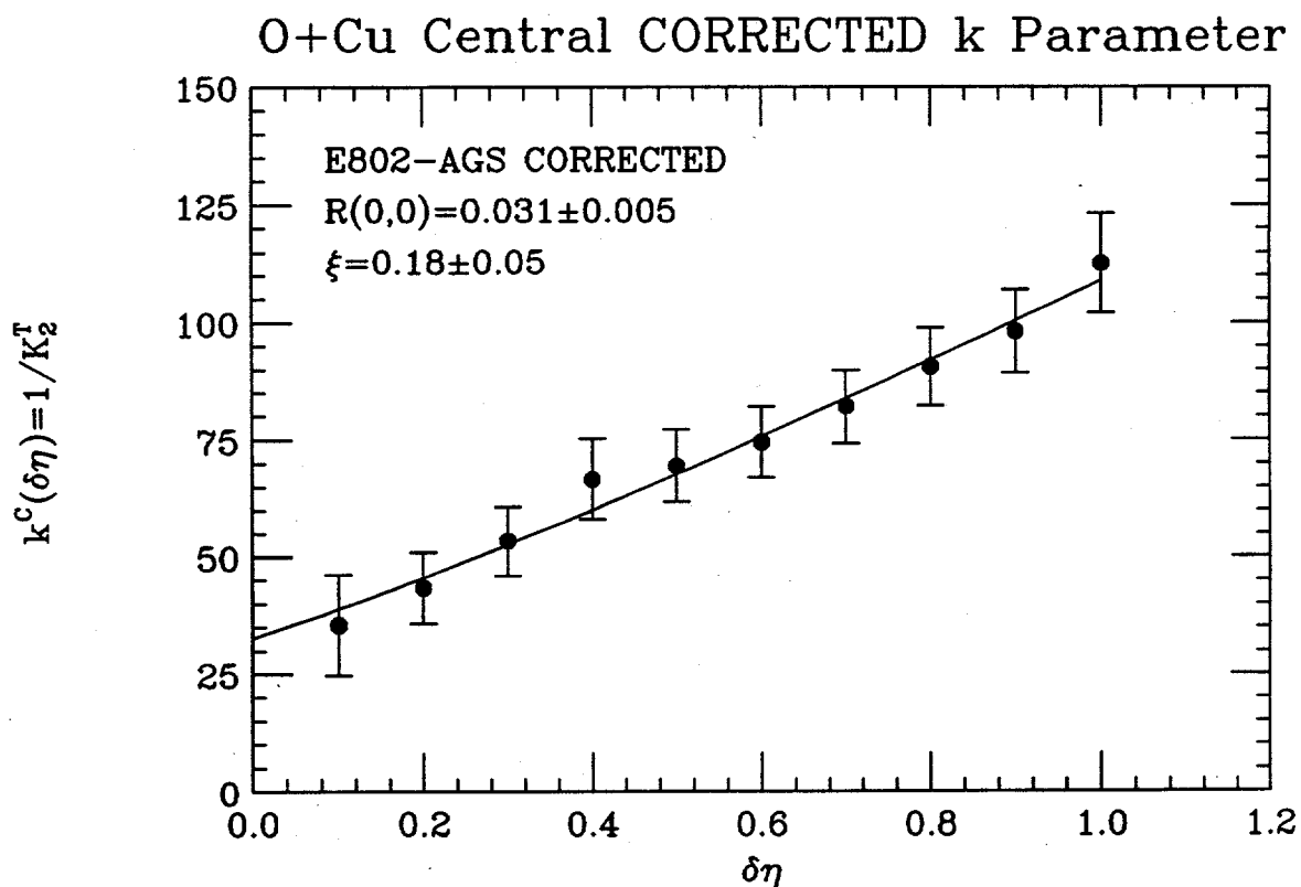
Figure 5: The k parameter from NBD fits to the data, corrected for instrumental effects, as explained in the text, presented as k^C(\delta\eta) \equiv 1/K_2^T(\delta\eta) as a function of the interval \delta\eta . The solid line is a fit to Eq. 10 with the parameters indicated.
