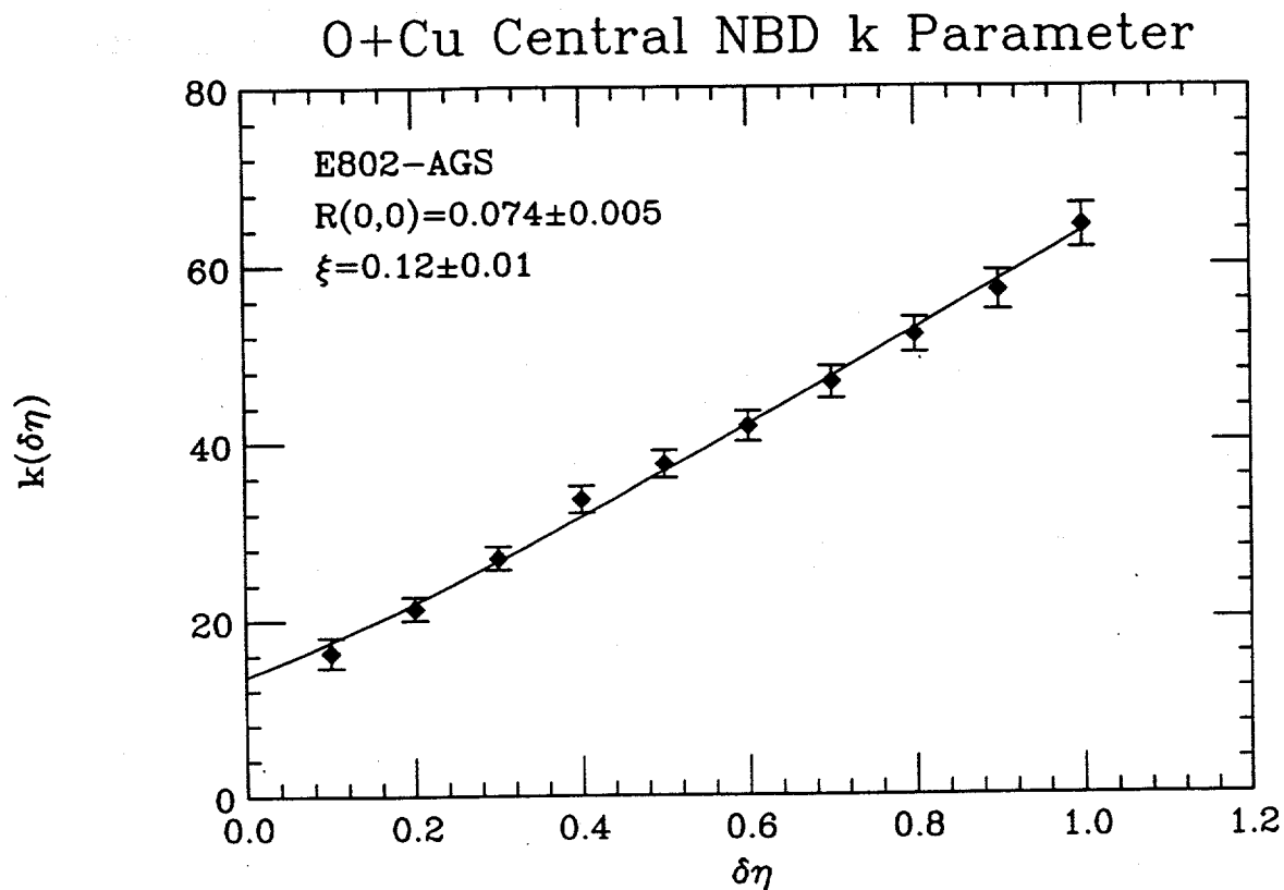
Figure 4: The NBD parameter k(\delta\eta) as a function of the interval \delta\eta (Fig. 2), together with a fit to Eq. 10 with the parameters indicated (solid line).
