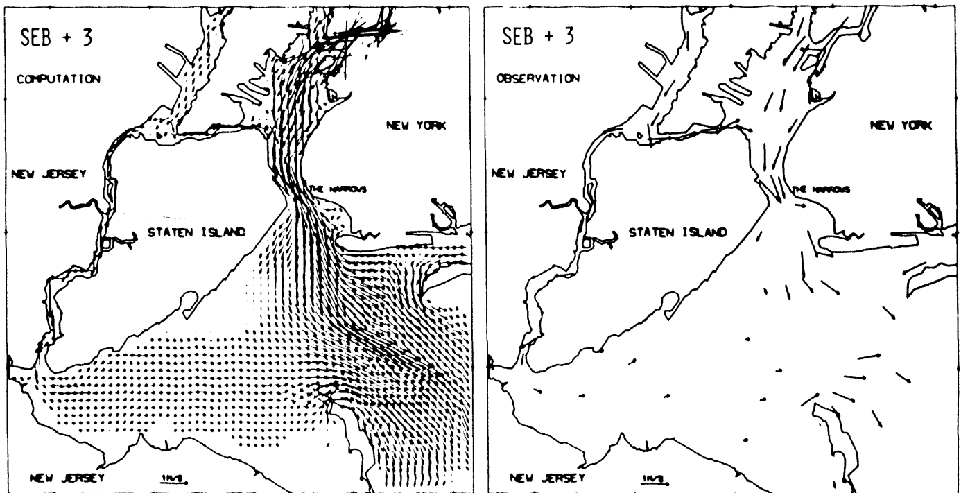
Computed and observed vertically averaged currents at the time of maximum ebb current at the Narrows.
