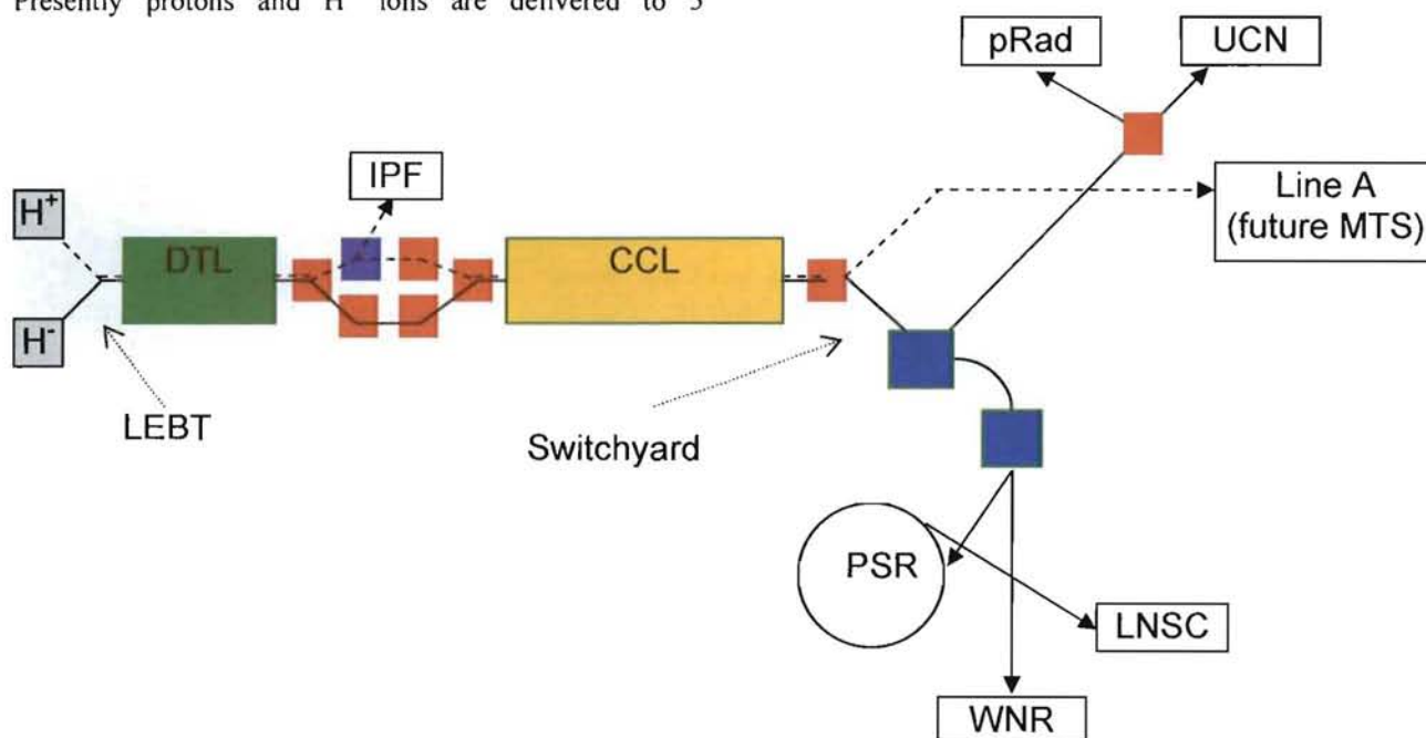
Figure 1: Schematic depiction of the LANSCE accelerator and experimental areas. Proton ( H^+ ) beam lines are shown as dashed lines and H^- beam lines are shown as solid lines. Blue squares depict pulsed magnets for switching beam delivery on a per macropulse basis. The experimental areas are: IPF: Isotope Production Facility; pRad: Proton Radiography; UCN: Ultra-Cold Neutrons; MTS: Materials Test Station (under development); LNSC: Lujan Neutron Scattering Center; WNR: Weapons Neutron Research. The beam switchyard, just downstream of the linac, directs beam to the various experimental areas.
