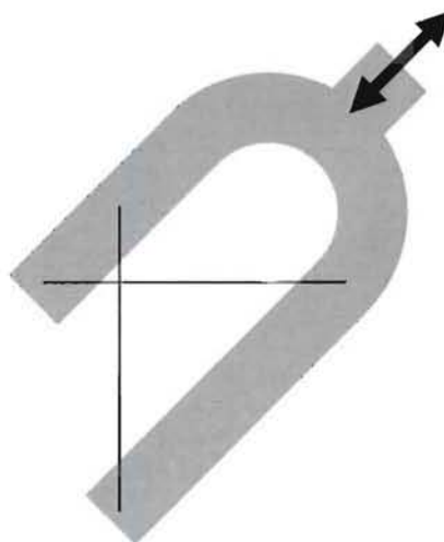
Figure 6 Wire locations on the actuator fork to eliminate cross-talk between the wires. The crossing point of the wires needs to be outside the beam-pipe aperture.
