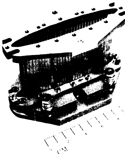
Figure 2. One of 48 flex bands in the storage ring. A flex band fits inside each bellows allowing expansion and contraction of the ring due to temperature changes while maintaining a smooth inside surface to prevent distortion of rf fields.
