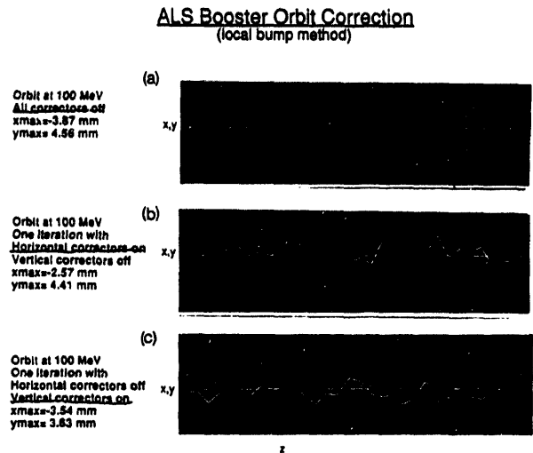
Figure 8. Correction of closed orbit in the booster: (a) uncorrected closed orbit; (b) closed orbit with horizontal correction; (c) closed orbit with vertical correction.
