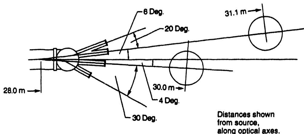
Figure 2. Floor layout of the experimental space at the end of Beamline 7.0.
