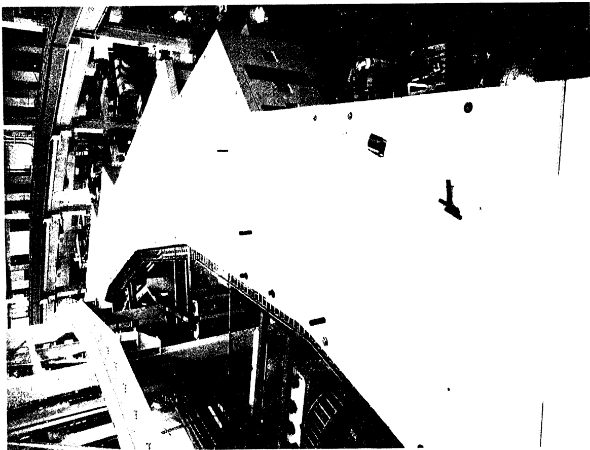
Figure 37. Storage ring enclosed by concrete shielding.
