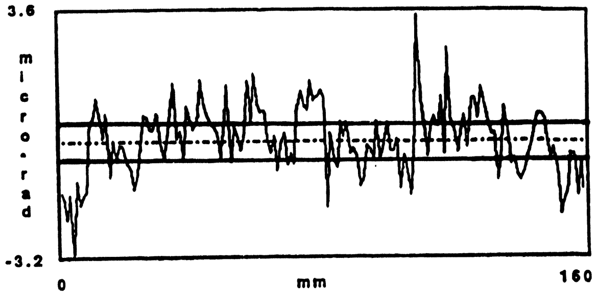
Figure 30. Results of figure measurements made by long trace profiler on a 18-cm-long, nickel-plated, spherical monochromator grating blank. The slope error of 1.0 \mu\text{rad rms} is due to the shape of the mirror and random errors in the measurement.
