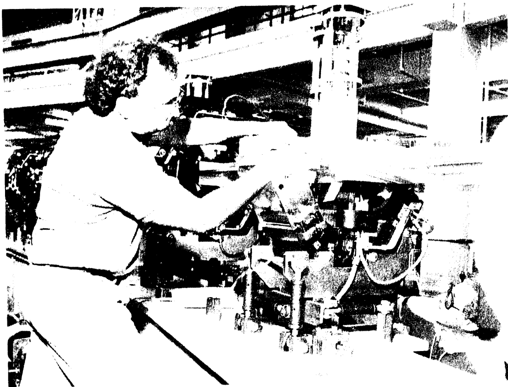
Figure 34. Sextupole magnets being installed onto one of the storage-ring girders.
