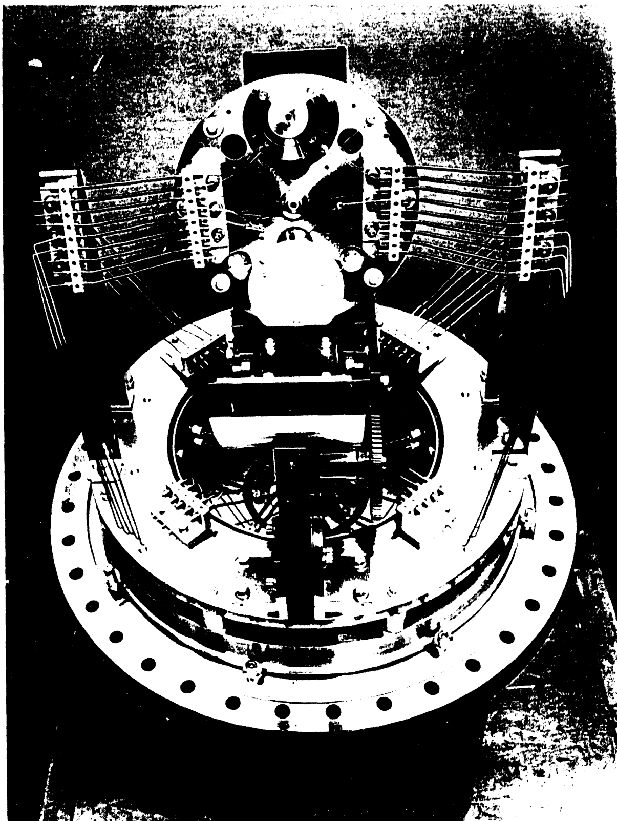
Figure 4. End station to be available to independent investigators for conducting condensed-matter, solid-state studies at the ALS.
