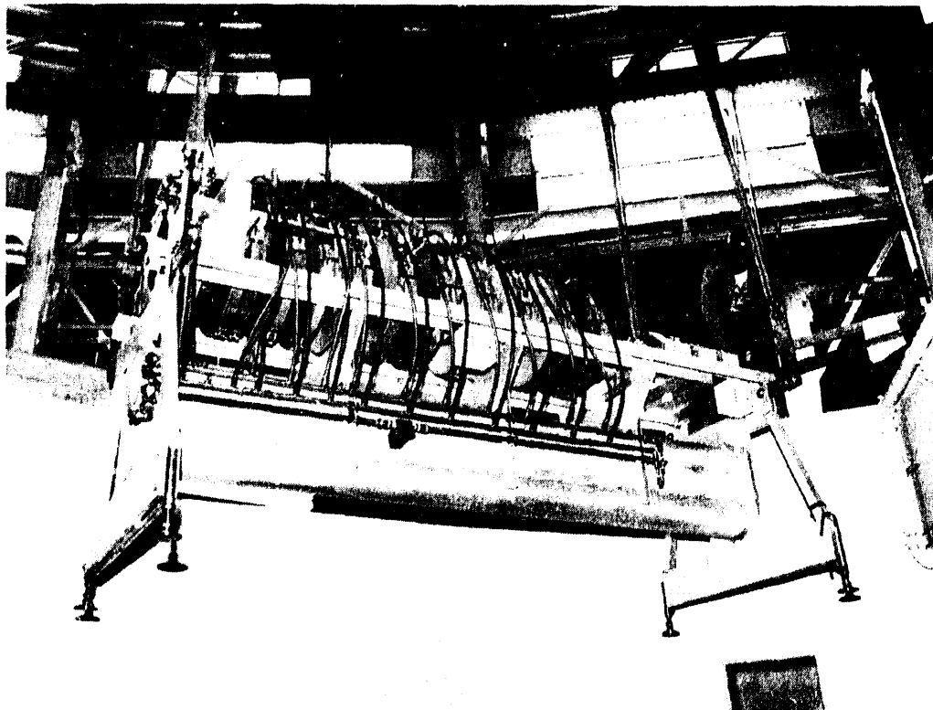
Figure 19. An accelerating section of the linac being lowered into its shielding enclosure.
