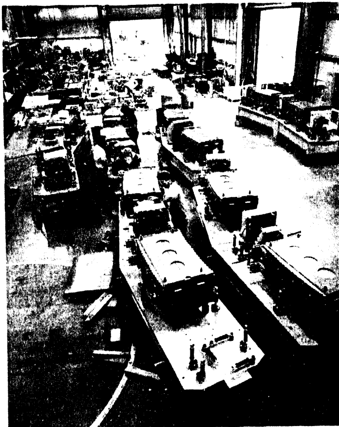
Figure 22. Shop for assembling magnets on booster girders.
