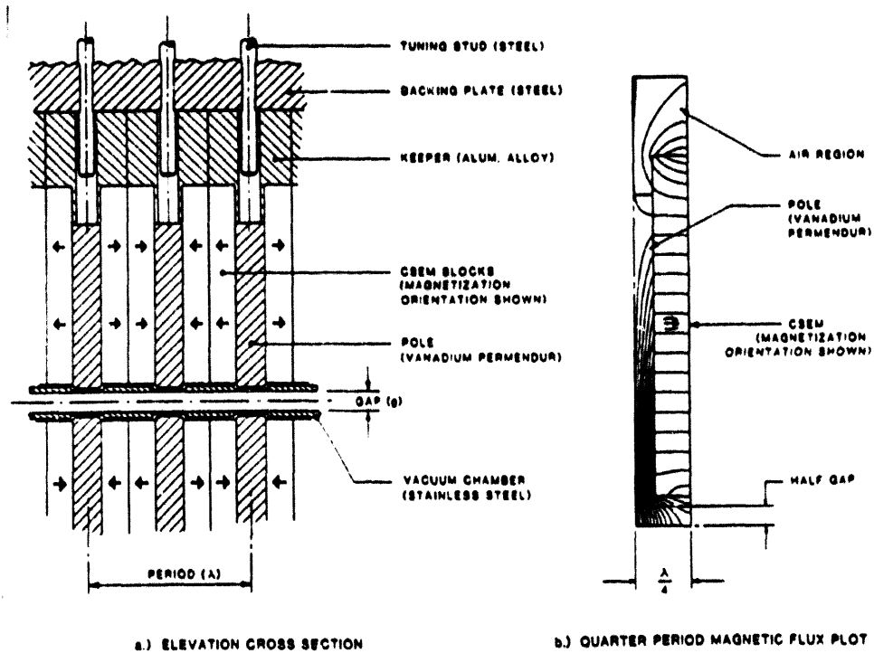
CSEM-STEEL HYBRID INSERTION DEVICE
