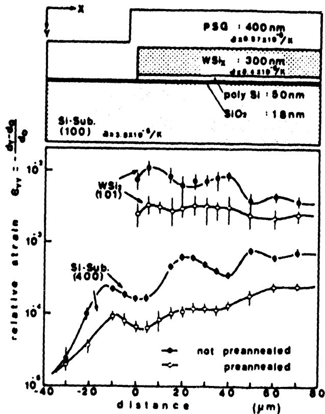
Strain Distribution in WSi 2 /polysilicon MOS capacitor. The "a"
