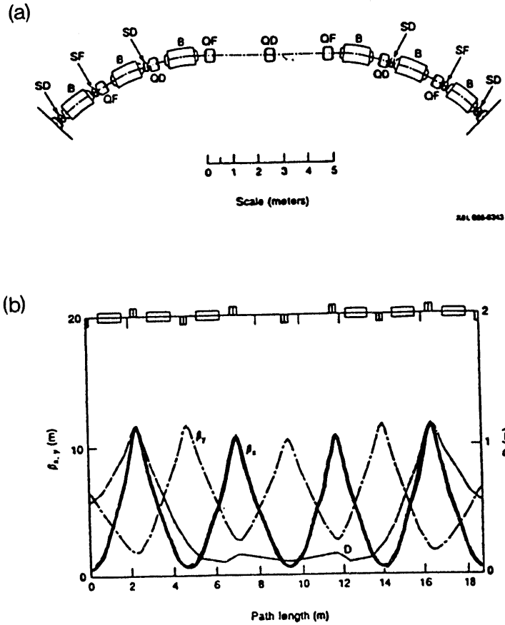
Figure 3. (a) Schematic of booster quadrant showing alternating focusing and defocusing magnets. (b) Amplitude functions derived from modelling.
