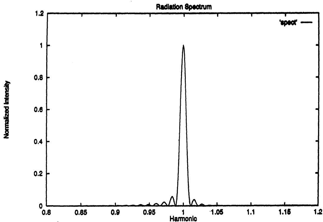
Figure 21. Computed synchrotron-radiation spectrum for first harmonic based on magnetic measurements indicates 99+% performance efficiency.
