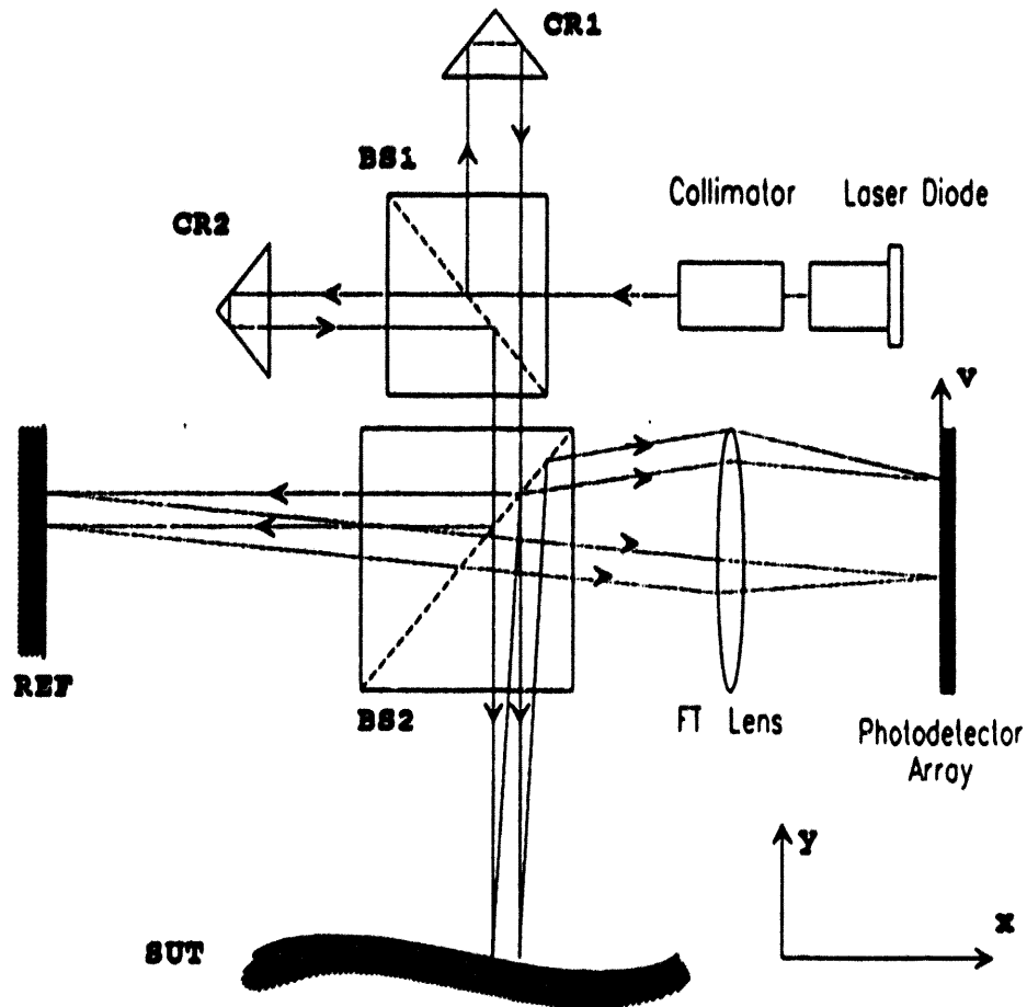
Figure 29. Schematic of long trace profiler used to measure surface figure of ALS optics.
