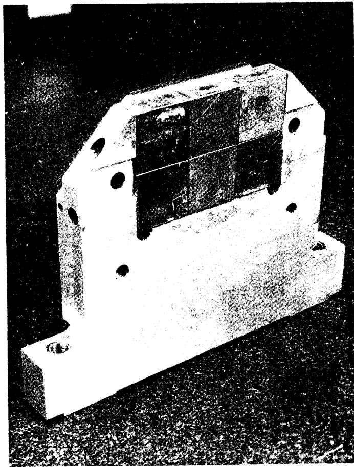
Figure 13. Pole assembly for ALS undulators consists of permanent-magnet blocks glued to steel poles and held together in an aluminum frame.
