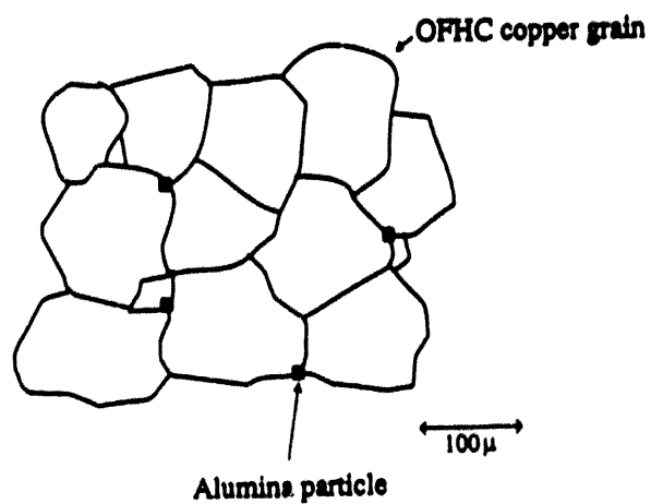
Figure 26. Structure of GlidCop™, a material used to make some ALS beamline optical components.
