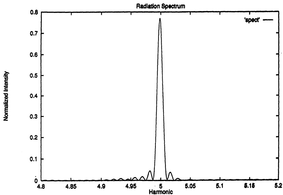
Figure 22. Computed synchrotron-radiation spectrum for fifth harmonic indicates almost 80% performance efficiency.
