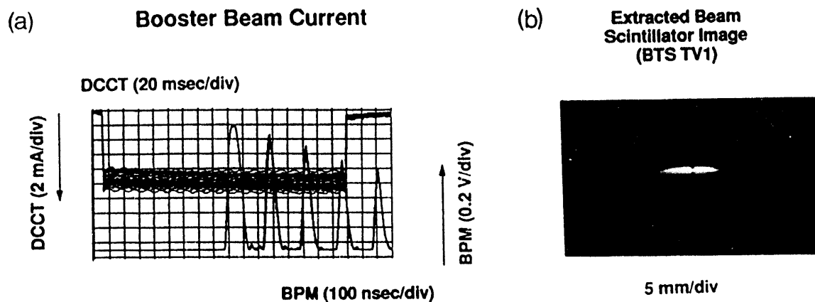
Figure 9. (a) Electron-beam current in the booster; (b) electron-beam cross section in the booster-to-storage-ring transport line.
