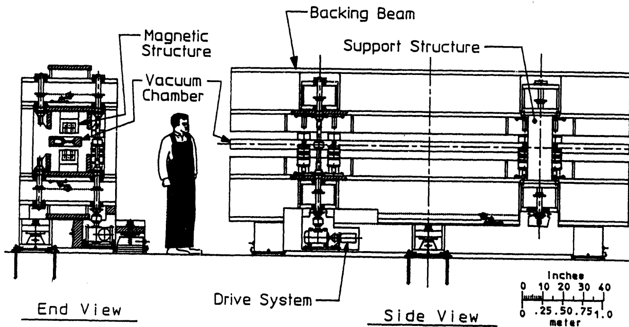
Figure 17. Diagram of undulator structure.
