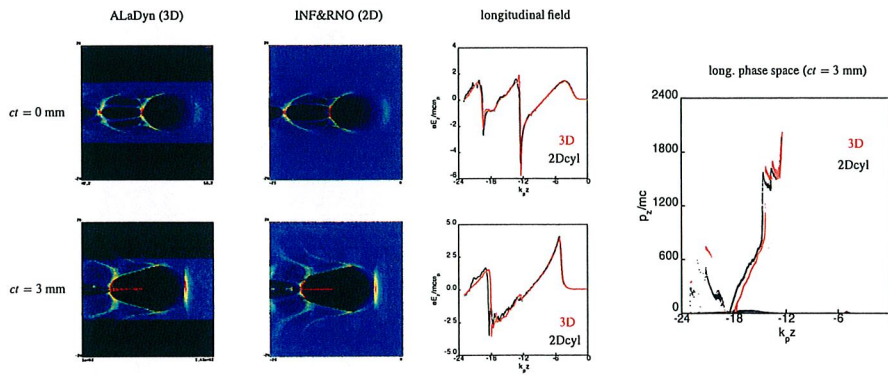
FIGURE 6. Comparison between a full LPA simulation performed with the 3D PIC code ALADyn and INF&RNO (see subsection "Test 5" for details).
