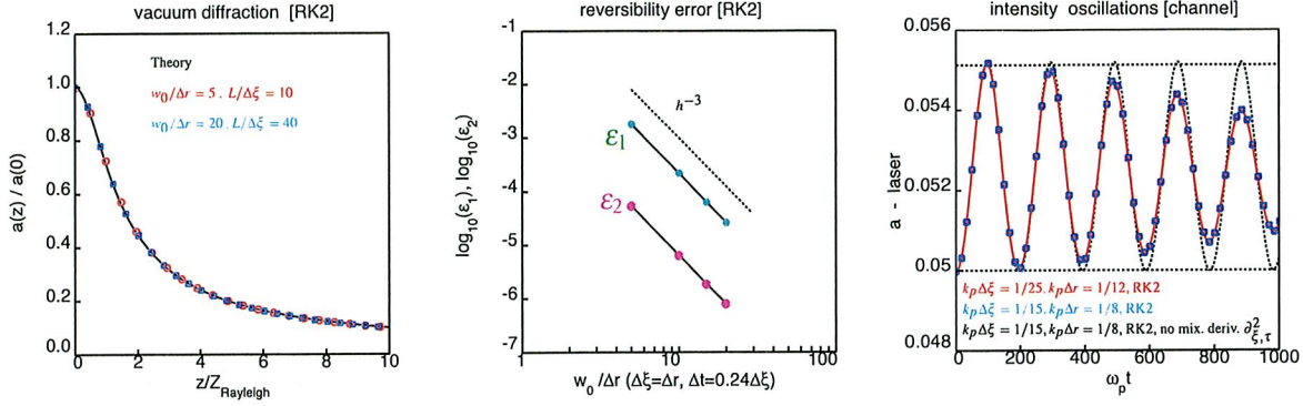
FIGURE 3. Left: vacuum diffraction of a focused laser pulse (see subsection "Test 1" for details). Center: time reversibility test for the vacuum diffracting pulse changing the resolution (see subsection "Test 1"). Right: mismatch oscillations of a low intensity pulse in a plasma channel (see subsection "Test 2" for details).
