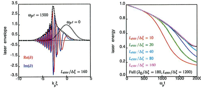
FIGURE 2. 1D fluid-envelope simulation: a_0 = 1.5, k_0/k_p = 20, k_p L = 2 . Left: black plots are the laser envelope profile at \omega_p t = 0 and \omega_p t = 1500 , the red/blue plots are the real/imaginary part of \hat{a} at \omega_p t = 1500 . Right: laser energy evolution deep into depletion as a function of the longitudinal resolution in the envelope (colored plots). The black plot is a full fluid simulation (no envelope approximation) at very high resolution (180 points/ \lambda_{\text{laser}} ) and can be considered an "exact" result.
