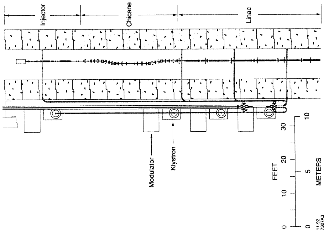
Figure 3. Plan view of the NLCTA injector, chicane, and linac.
