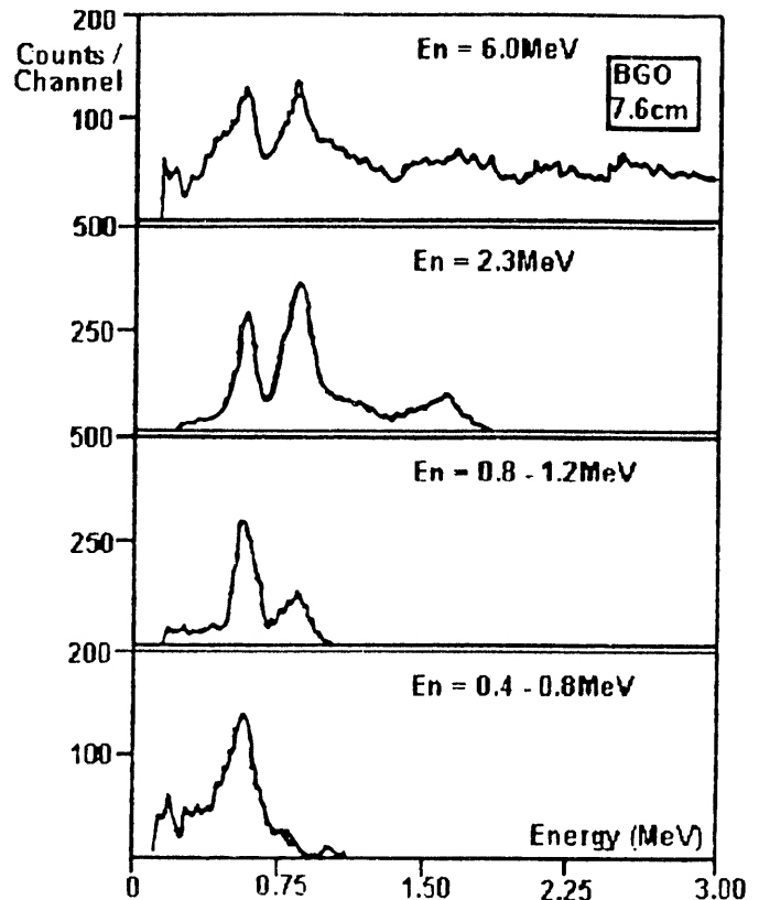
Fig. 2. Gamma ray spectra produced in BGO by high energy neutron irradiation (from Ref. 3).
