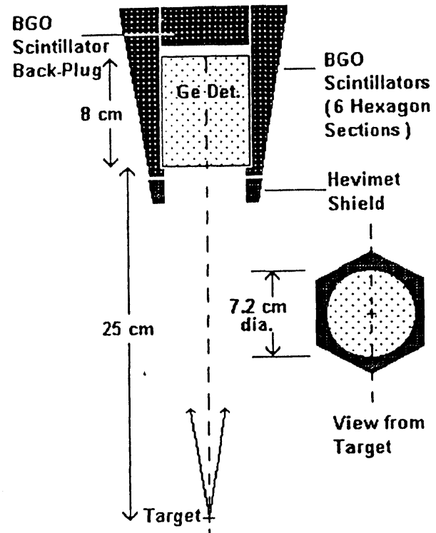
Fig. 1. Target/detector geometry for a single detector module in GAMMASPHERE. 110 modules surround the target.
