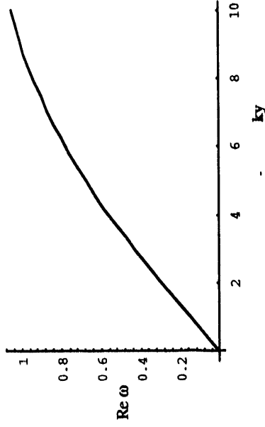
Fig. 5.1 The real part of the dispersion relation. This gives the frequency spectrum as a function of ky .
