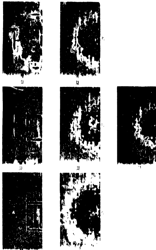
Fig. 4.9 Evolution of the spectrum with driving and damping (under the polarization drift nonlinearity only) subsequent to a impulse of energy localized to a rectangular annulus in k space. Time goes sequentially from left to right and down. The 0.0 mode is at the center bottom of each snap shot and the scale is from dark gray (near center) signifying the most energy through white to black signifying the least energy.
