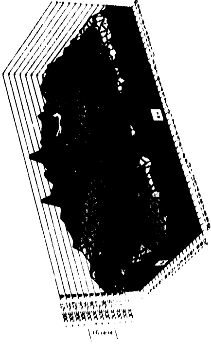
Fig. 4.7 Spectrum of turbulence driven at long wavelength and damped by a hyperviscosity at short wavelength with an inertial range in the intermediate modes. There is also damping at the smallest wavenumbers, representing the effect of ion-ion
