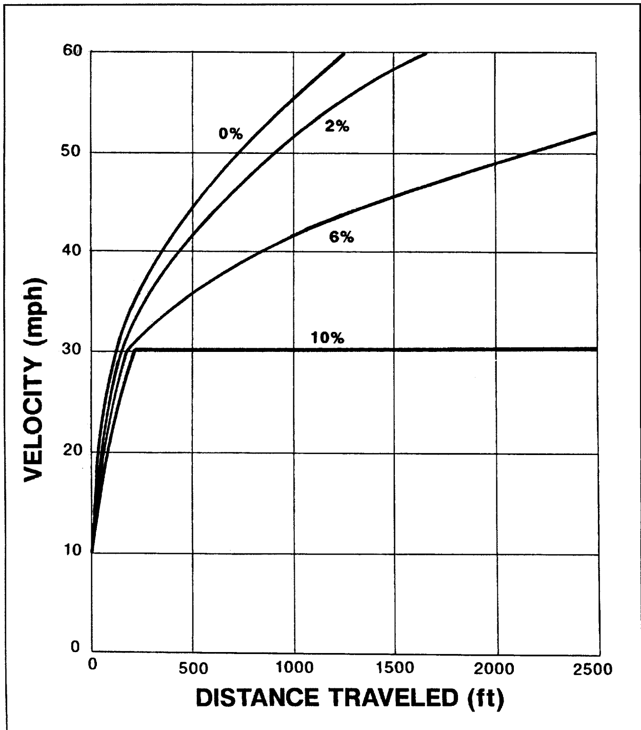
Figure 6.2 Vehicle velocity from dead start
