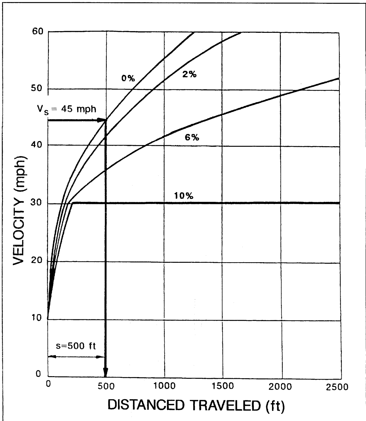
Figure 6.7 Example - Vehicle velocity from dead start
