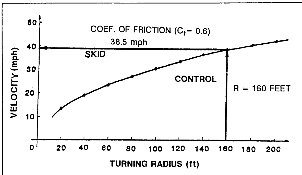
Figure 6.6 Example - Vehicle velocity on curves
