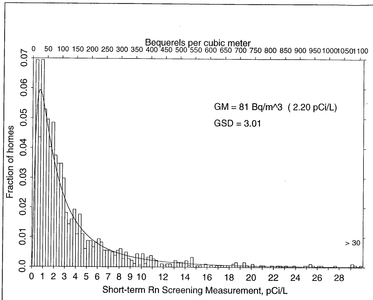
Fig. 1. The distribution of short-term radon screening measurements collected in the New Hampshire Radon Survey.
