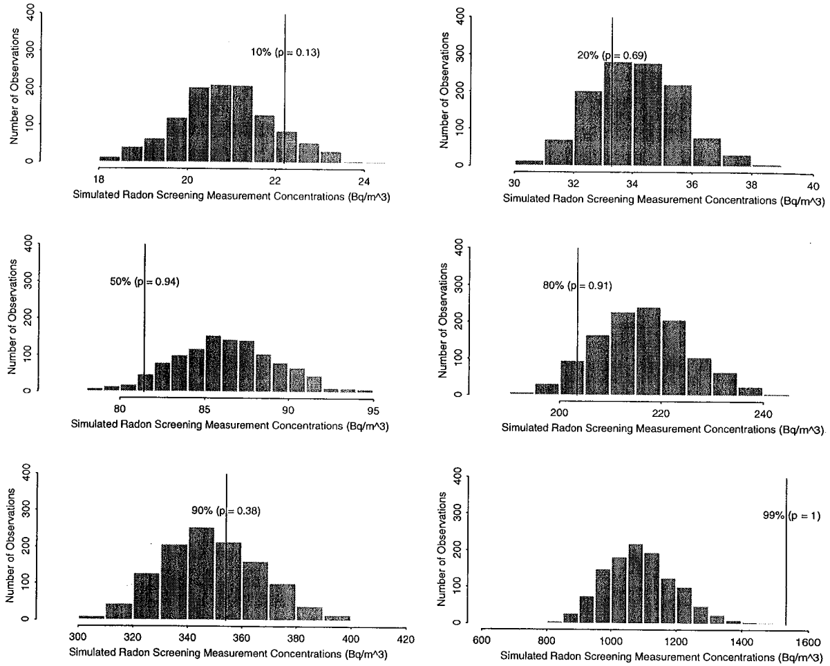
Fig. 7. Bayesian posterior predictive checks of 1200 simulations of Model 10. The predictive checks have been conducted at the 10th, 20th, 50th, 80th, 90th, and 99th percentiles. The superimposed line on each histogram of posterior distributions is the measurement at the percentile in question, from the New Hampshire Radon Survey. The p-value presented is a Bayesian p-value , as discussed in the text. For example, the first plot shows that the 10th-percentile measurement was about 22 Bq/m 3 (vertical line), and that simulated data from the posterior distribution had 10th-percentile values between about 19 and 22.5 Bq/m 3 most of the time (histogram), with the simulated 10th-percentile value exceeding the actual measurement about 11% of the time ( p=0.11 ).
