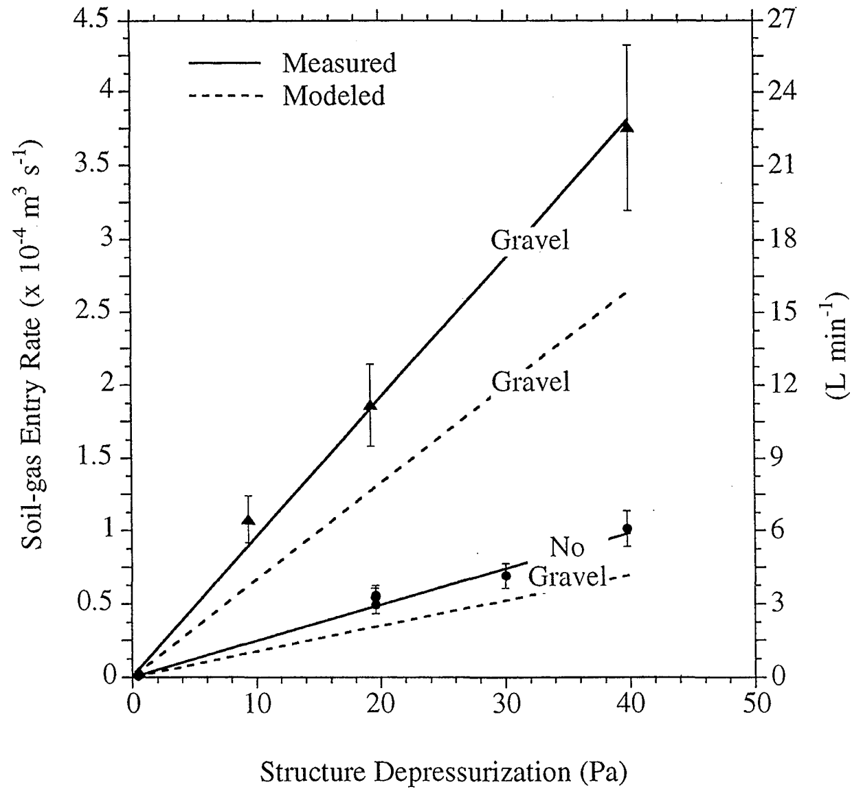
Fig. 2. A comparison of measured and modeled soil-gas entry rate into both structures as a function of structure depressurization. Lines through measured points are linear regressions weighted by uncertainties. The vertical bars represent measurement uncertainty.
