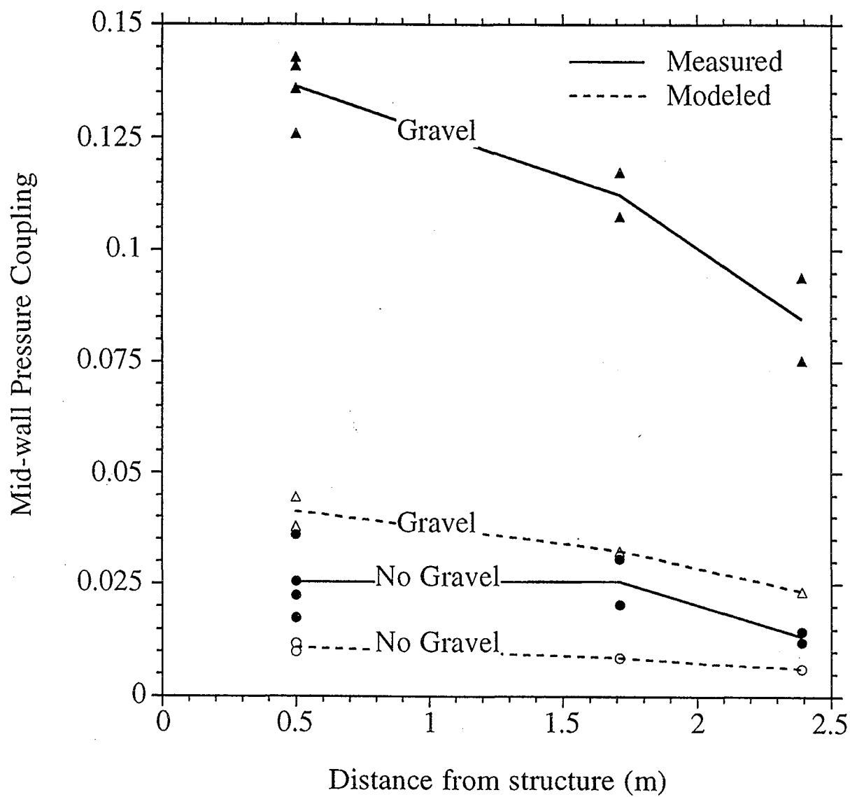
Fig. 5. A comparison of measured and modeled mid-wall (0.8 m below grade) pressure coupling around both structures with all six slots open. Lines, symbols, and uncertainties are the same as in Fig. 3.
