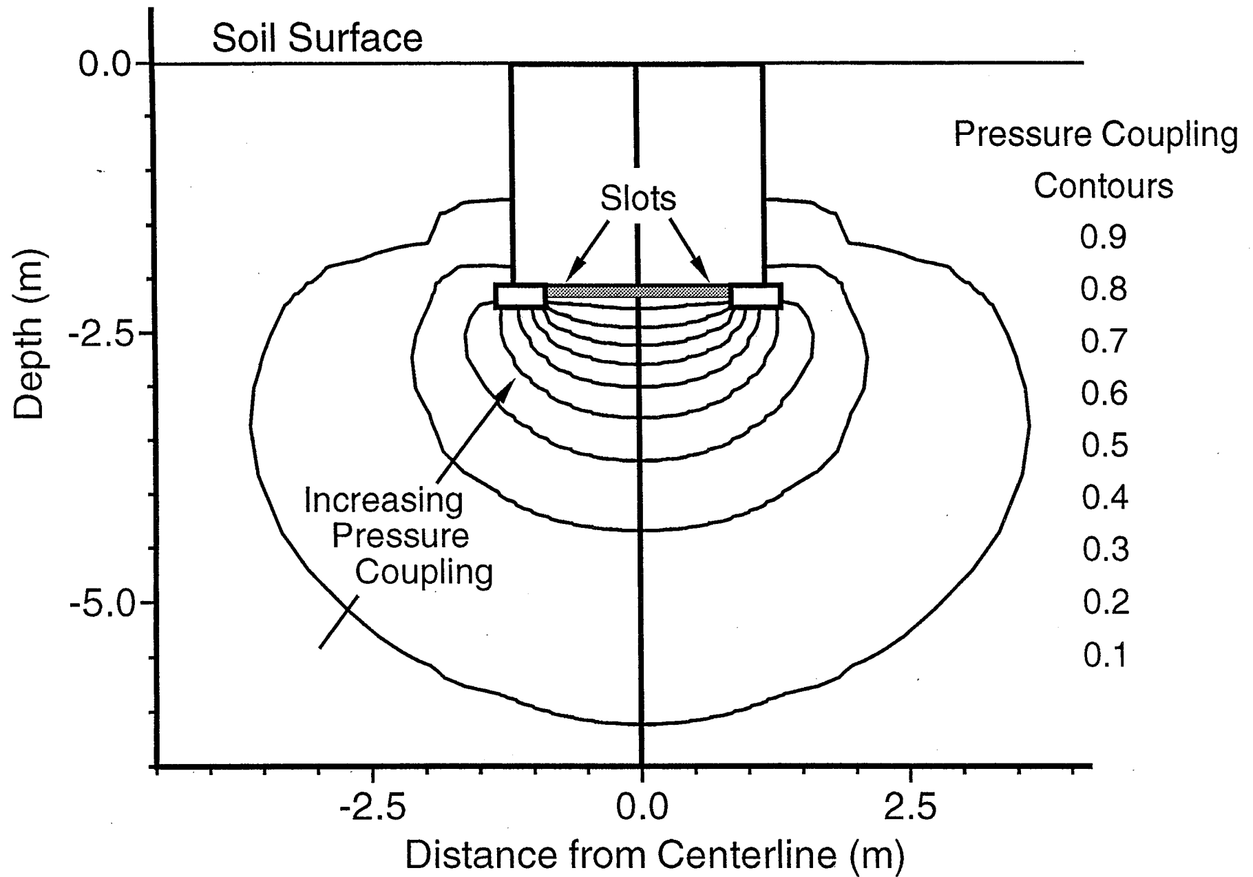
Fig. 6a. Model prediction of the pressure coupling field in the east-west cross-section around the gravel structure with all six-slots open. Lines are pressure coupling contours. The subslab gravel layer is represented by the shaded region underneath the structure floor. The cusp in the 0.1 pressure coupling contour near the structure wall occurs at the interface between the backfill and the undisturbed soil. The permeability changes by an order of magnitude at this interface (see Table 2). The line down center of the figure represents the model's plane of symmetry.
