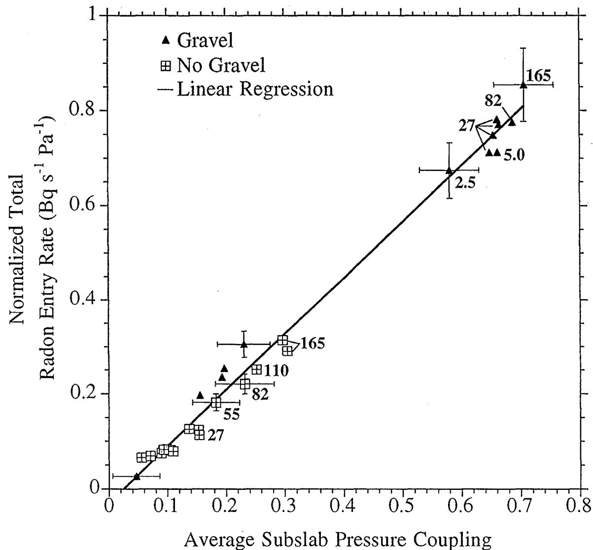
Fig. 8 Measured total advective radon entry rate into both structures normalized by structure depressurization as a function of average subslab pressure coupling. Numbers indicate open area in units of 10^{-4} \text{ m}^2 . Vertical bars indicate uncertainty of measured radon entry rate, a maximum of 12%; horizontal bars indicate uncertainty of average pressure coupling, a maximum of \pm 0.05 . Error bars omitted on some points for visual clarity.
