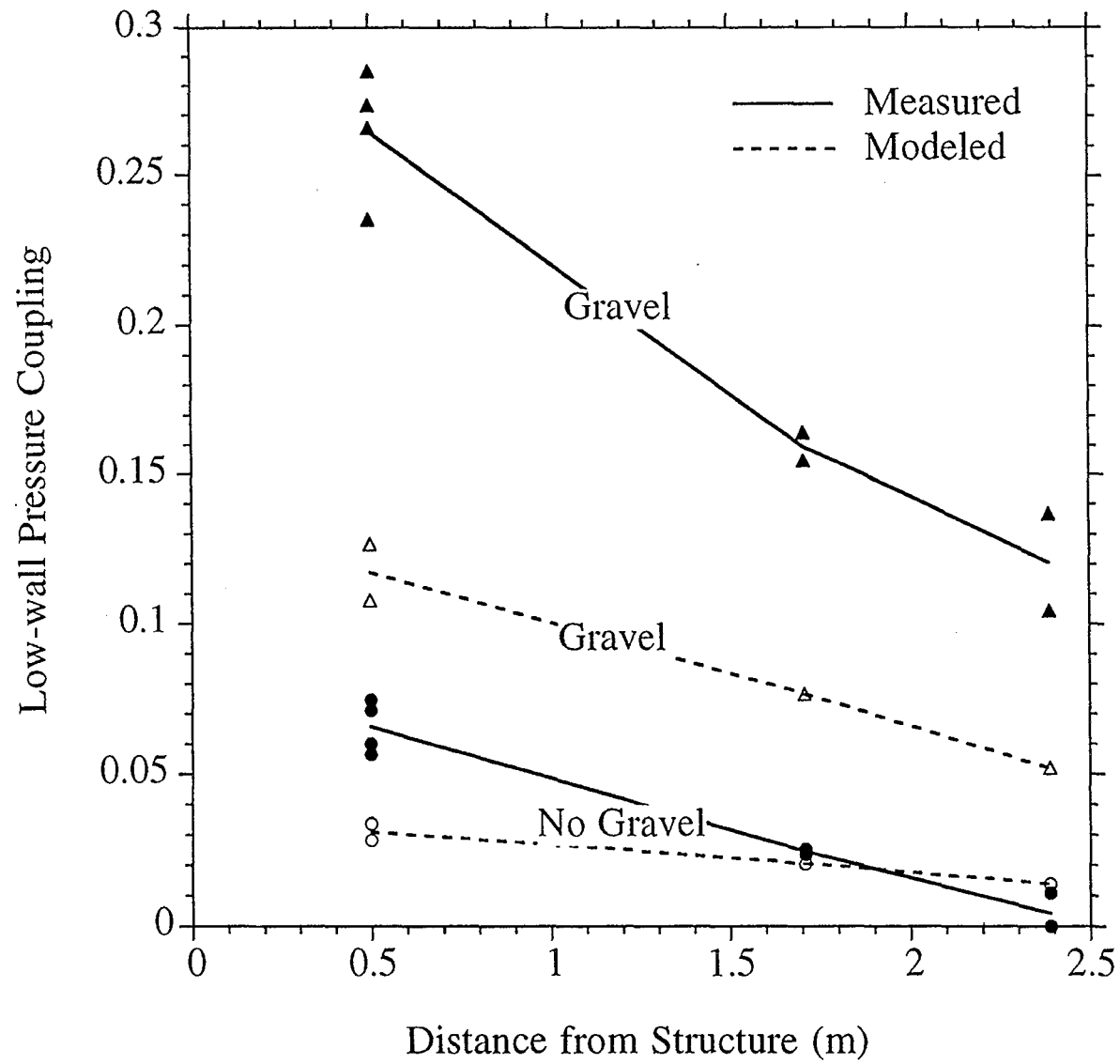
Fig. 4. A comparison of measured and modeled low-wall (1.6 m below grade) pressure coupling around both structures with all six slots open. Lines, symbols, and uncertainties are the same as in Fig. 3.
