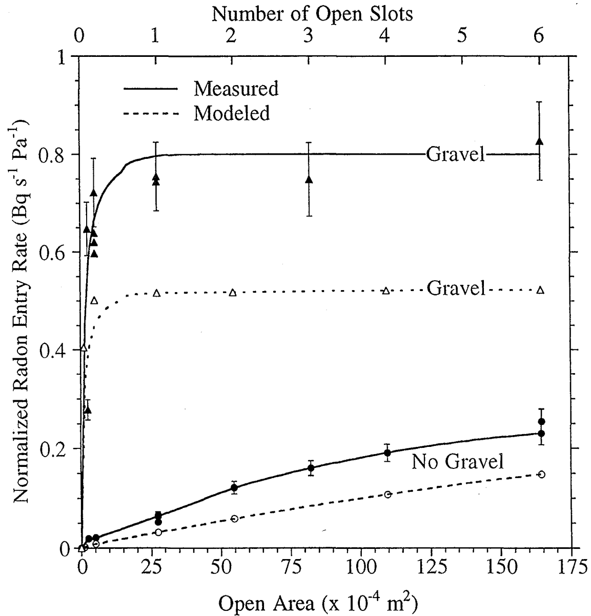
Fig. 7. A comparison of measured and modeled advective radon entry rate normalized by structure depressurization as a function of open area. Solid symbols indicated measured values; open symbols indicate modeled values. Lines are intended for visual guidance only. The vertical bars represent experimental uncertainty.
