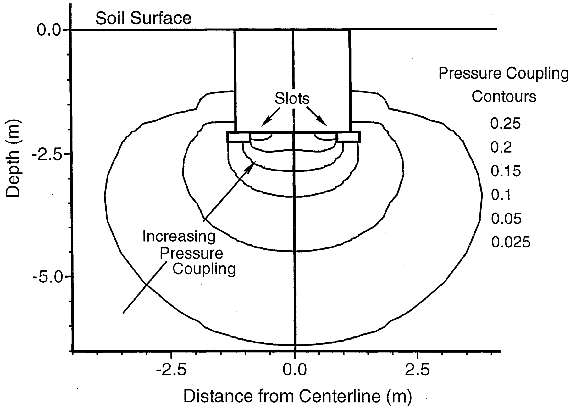
Fig. 6b. Model prediction of the pressure coupling field in the east-west cross-section around the no-gravel structure with all six-slots open. Lines are pressure coupling contours. The cusp in the 0.025 pressure coupling contour near the structure wall corresponds to the interface of the backfill and undisturbed soil. The permeability changes by an order of magnitude at this interface (see Table 2). The line down center of the figure represents the model's plane of symmetry.
