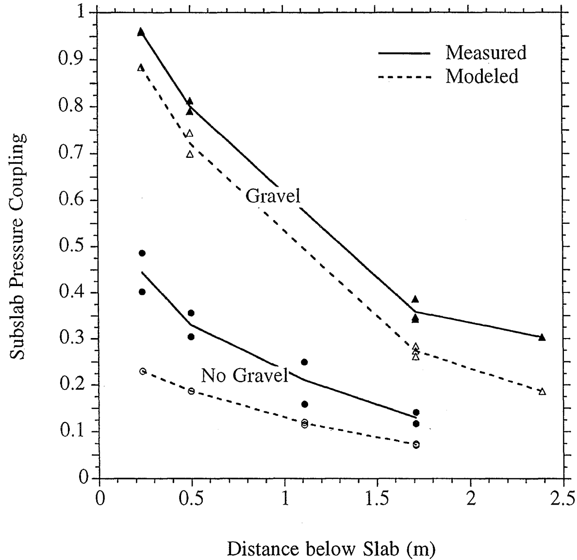
Fig. 3. A comparison of measured and modeled subslab pressure coupling underneath both structures with all six slots open. Lines connect average values for a each probe length and are intended for visual guidance only. Note there are no 1.11-m-long probes underneath the gravel structure, and no 2.39-m-long probes underneath the no-gravel structure. Measured values indicated by solid symbols; modeled values indicated by open symbols. The maximum uncertainty on the measurements is \pm 0.02 in the no-gravel structure, and \pm 0.03 in the gravel structure.
