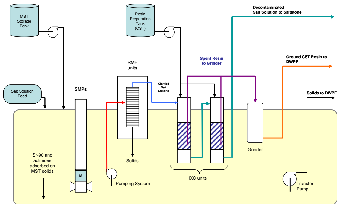
Figure 1. Simplified process diagram for SCIX.
