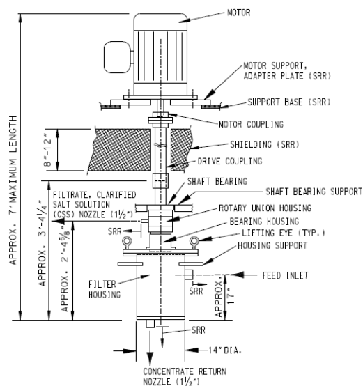
Figure 2. Conceptual design of the RMF Component.
