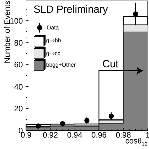
Figure 1: Angular distribution between vertex axes in jet 1 and jet 2 ( 0.9 < \cos \theta_{12} ) (points). The simulated distribution is shown as a histogram.
