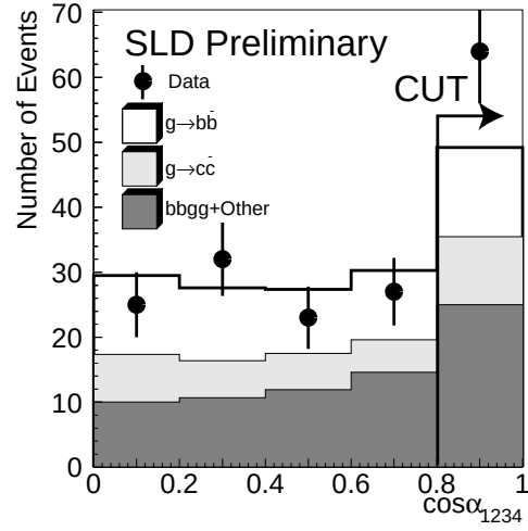
Figure 2: The distribution of the cosine of angle between the plane \Pi_{12} formed by jets 1 and 2 and the plane \Pi_{34} formed by jets 3 and 4, for data (points) and Monte Carlo simulation (histogram). We reject |\cos \alpha_{1234}| > 0.8
