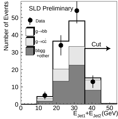
Figure 3: The distribution of the energy sum of jet 1 and jet 2.
