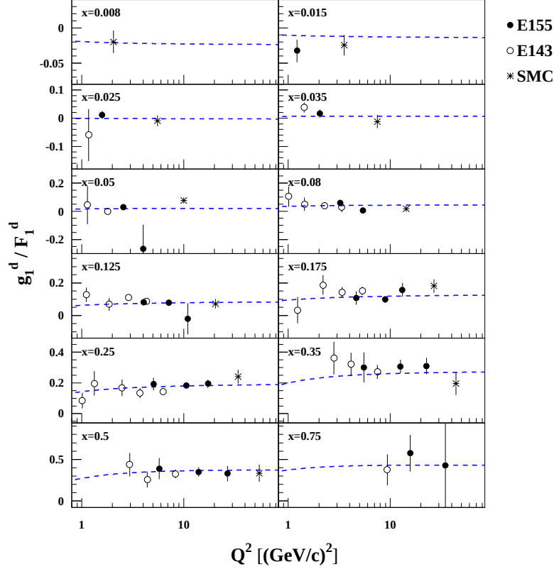
FIG. 3. g_1^d / F_1^d for E155 vs. other experiments. The multiple points in each bin for E155 are for the separate spectrometers. The dashed curves are from a functional fit to world data on g_1 / F_1 .
