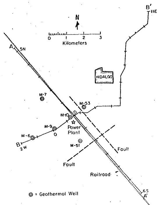
Fig. 1. Self-potential survey lines, Cerro Prieto geothermal field, Baja California, Mexico.
