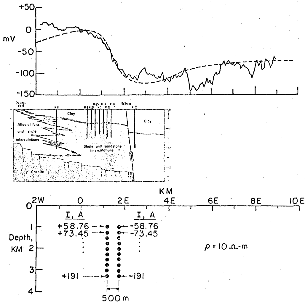
Fig. 3. Self-potential (projected onto a straight line), geologic cross-section (from Manon, et al., 1977), and electrical model for line B-B'. The dashed line on the self-potential profile is generated by the electrical model, which consists of a vertical sequence of current dipoles, each of magnitude (\pm 58.76 z) amps, where z is the depth of the dipole in km.
