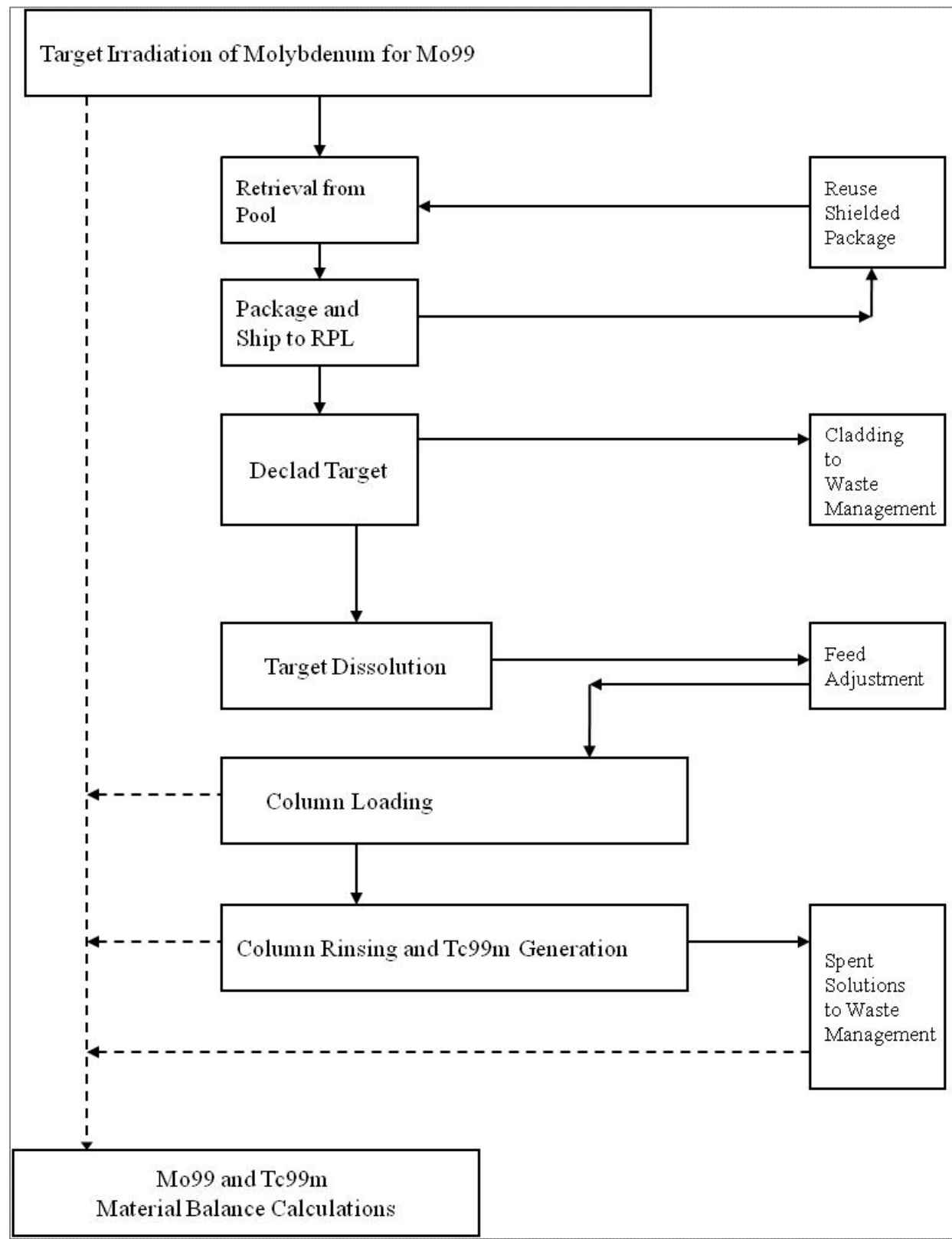
Figure A.6. Process Flow for Processing the Targets and Recovering the ^{99}\text{Tc} in a Hot Cell (Task 4).
