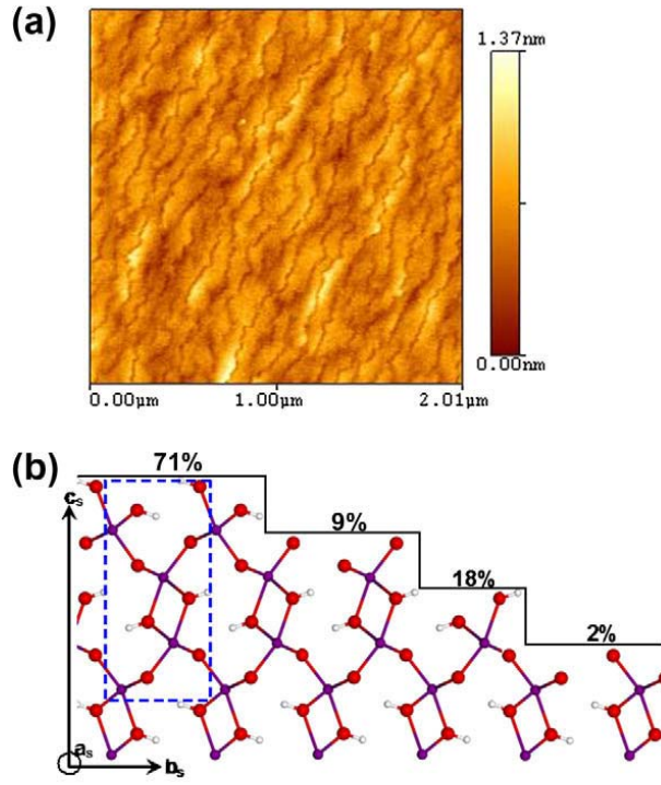
Fig. 3. (a) Step height distributions of goethite (100) surface: AFM image in height mode analysis shown over one 2\ \mu\text{m} \times 2\ \mu\text{m} area, but representative of many such areas. Step height analysis shows the presence of quarter, half, and three quarter step heights. Here a full step height corresponds to the size of the unit cell along the surface normal c_s = 9.9629\text{\AA} . (b) A schematic representation of the steps on the (1 0 0) surface of the goethite surface model. The blue dashed box shows the unit cell dimensions for a (0 1 1) face. The unequal fractions of different domains are determined from the CTR analysis. The best fit model consists of 71% of double hydroxyl layer 1, 9% double oxygen layer 4, 18% double hydroxyl layer 7 (an opposite handed layer 1) and 2% double oxygen layer 10 (an opposite handed layer 4) with the layer fractions determined with a 2% uncertainty.
