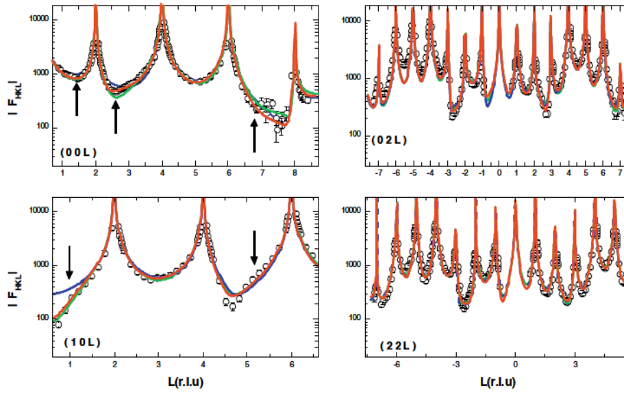
Fig. 4. Selected rods with experimental (circles) and theoretical structure factors ( F_{HKL} ) as a function of perpendicular momentum transfer ( L , in reciprocal lattice units) for the \alpha -FeOOH (100) surface. The blue solid lines are the calculated CTRs for the combined-domain relaxed fit model with double hydroxyl termination ( \text{OH}-\text{OH}-\text{Fe}-\text{O}-\text{O}-\text{Fe}-\text{R} ) with no water layers present. The green solid lines represent the fit model, with single-hydrated double hydroxyl termination ( (\text{H}_2\text{O})-\text{OH}-\text{OH}-\text{Fe}-\text{O}-\text{O}-\text{Fe}-\text{R} ). The red solid lines represent the best fit model, the double-hydrated double hydroxyl termination ( (\text{H}_2\text{O})-(\text{H}_2\text{O})-\text{OH}-\text{OH}-\text{Fe}-\text{O}-\text{O}-\text{Fe}-\text{R} ). The atoms in bold face represent the water layers. The arrows mark the reciprocal lattice positions where the fits have significant mismatch to the experimental data.
