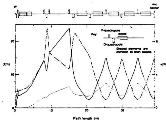
Figure 2. One quadrant of the low-energy ring.
