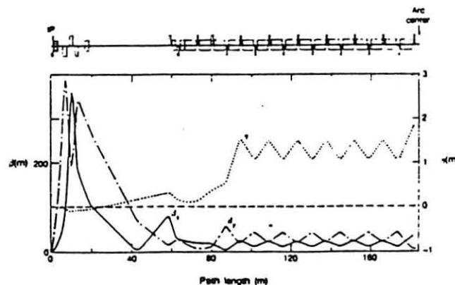
Figure 3. Half of the PEP sextant containing the B-Factory IR.
