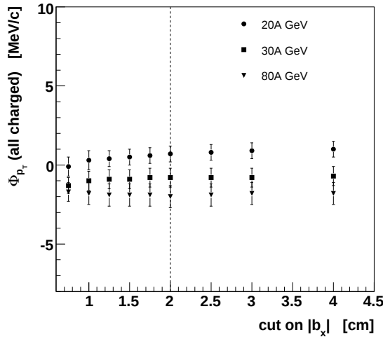
Figure 6: Dependence of \Phi_{p_T} on upper cut in the impact parameter |b_x| . For each point, the cut on |b_y| is equal to half the cut on |b_x| . Note: the values and their errors are correlated. The dashed line indicates the cut used in the analysis.
