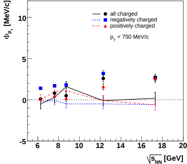
Figure 17: (Color online) \Phi_{p_T} as a function of energy for the 7.2% most central Pb+Pb interactions, with additional cut p_T < 750 MeV/c. Data (points) are corrected for limited two-track resolution. Lines show results of UrQMD calculations with the same kinematic and acceptance restrictions. Errors are statistical only.
