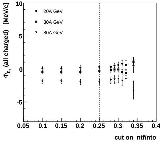
Figure 4: Dependence of \Phi_{p_T} on one of the event cuts ( ntf/nto ratio). Note: the values and their errors are correlated. The dashed line indicates the cut used in the analysis.
