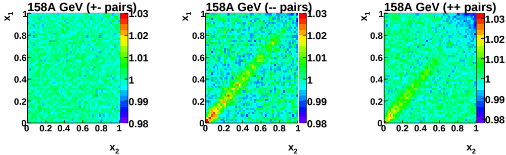
Figure 15: (Color) Two-particle correlation plots (x_1, x_2) using the cumulant p_T variable x . The bin contents are normalized by dividing with the average number of entries per bin. Plots are for central Pb+Pb collisions at 158A GeV for unlike-sign particles (+-), and for negatively and positively charged particles, separately. Note that the color scale can be slightly different for different panels.
