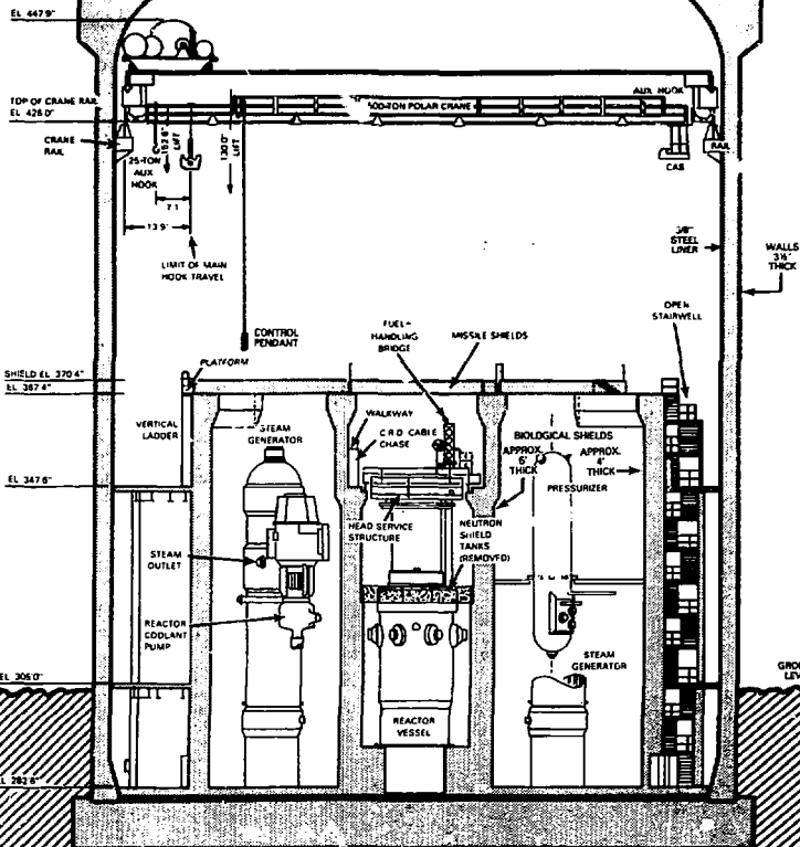
TMI-2 Reactor Building
