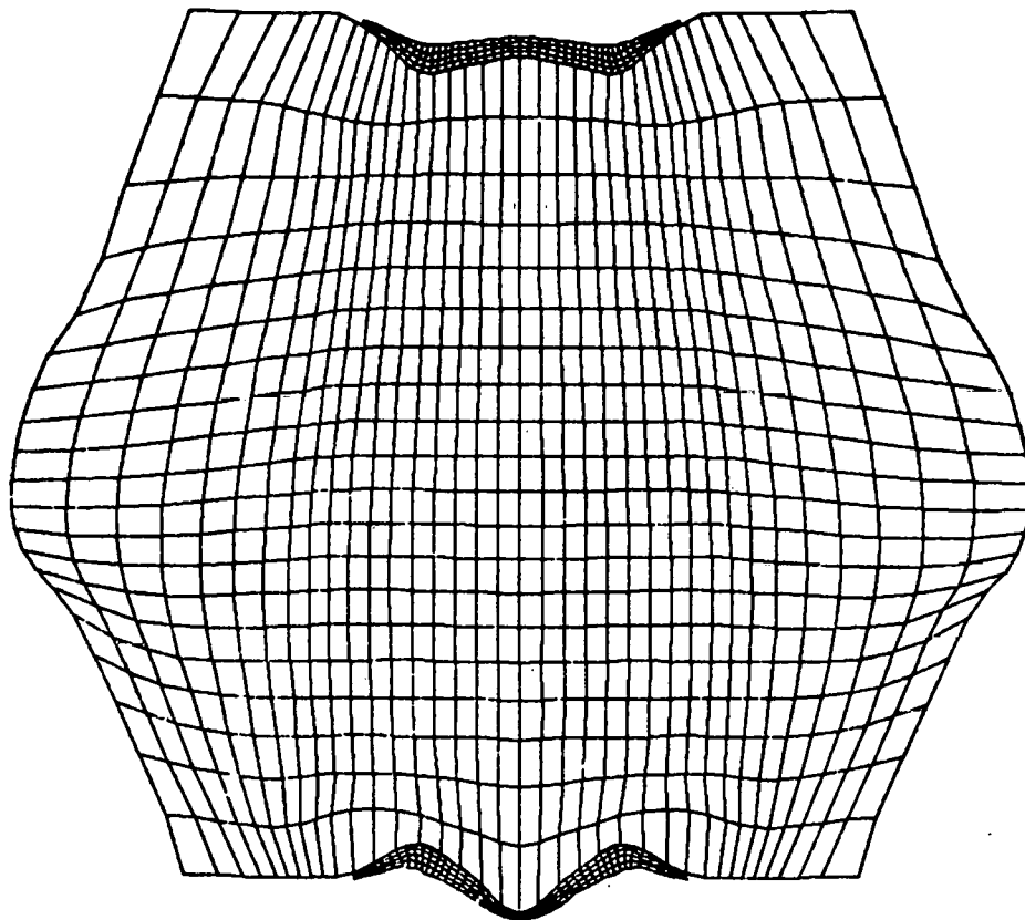
Fig. 22. Deformed shape at 50 \mu s.
