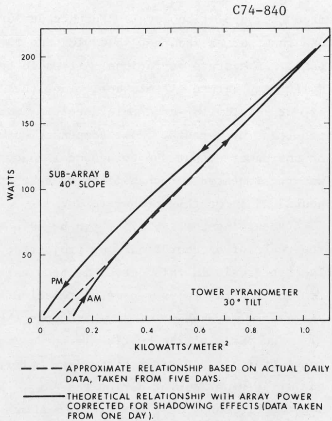
Fig. 2. Array output vs. insolation.
