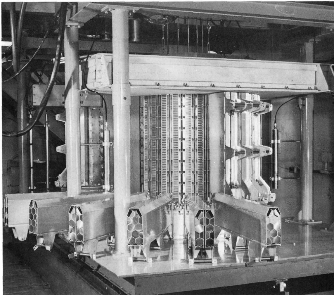
Fig. 5.21—RAG-1 folded-flow mockup for critical experiments, shown with six reflector sections dropped down
