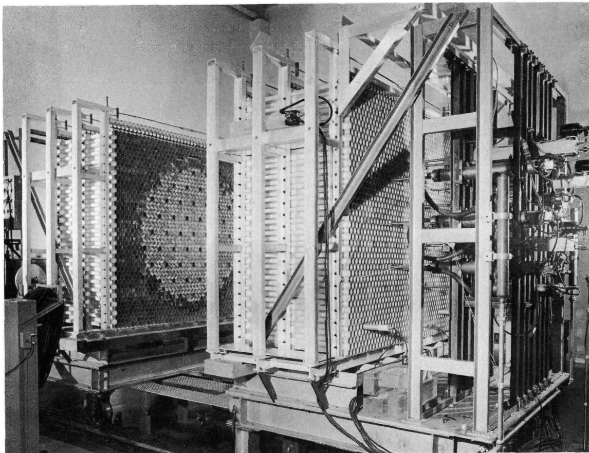
Fig. 5.8—MOP-I reactor
