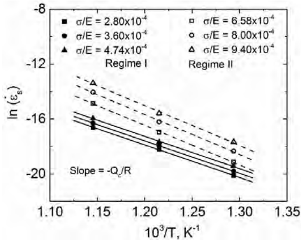
Figure 1.8. Arrhenius plots at different stresses (regimes I and II)
