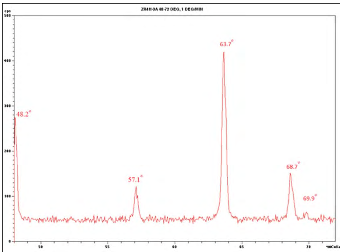
Fig. 4.13 Post Annealing Zircaloy-4: 48° – 72° in 2 \theta . Sample Zr4H-3A.
