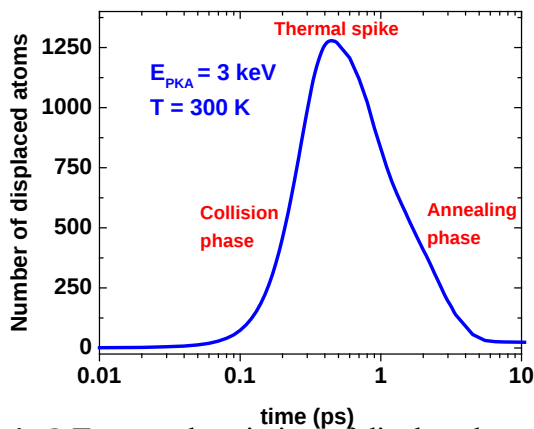
Fig.2 Temporal variation of displaced atoms
