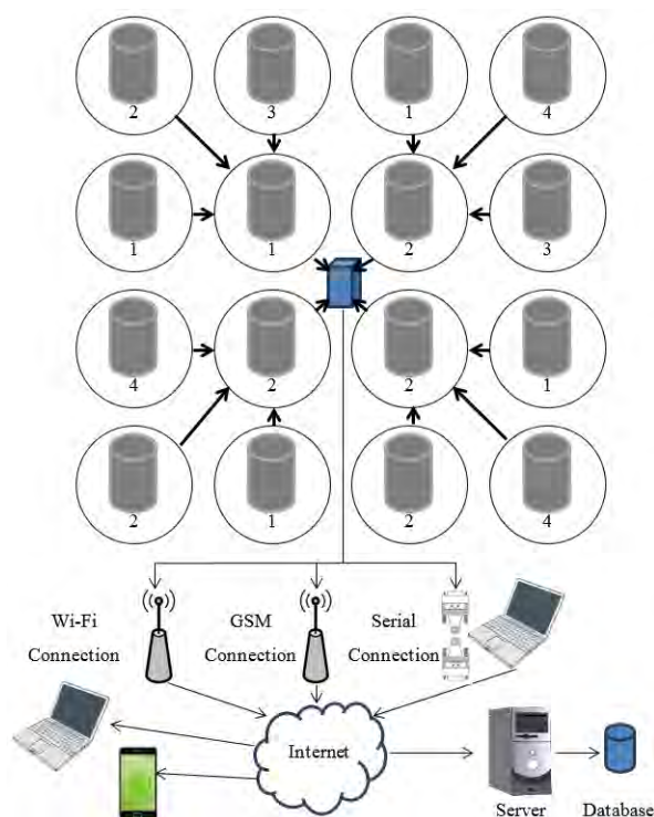
Figure 30. Example Sensor Network Configuration. This example network contains 16 SNF storage systems (grey cylinders) with a various number of nodes at each system. All of these nodes report to the central coordinator (blue box), which then manages the data by storing and/or transmitting it by various means to a server.
