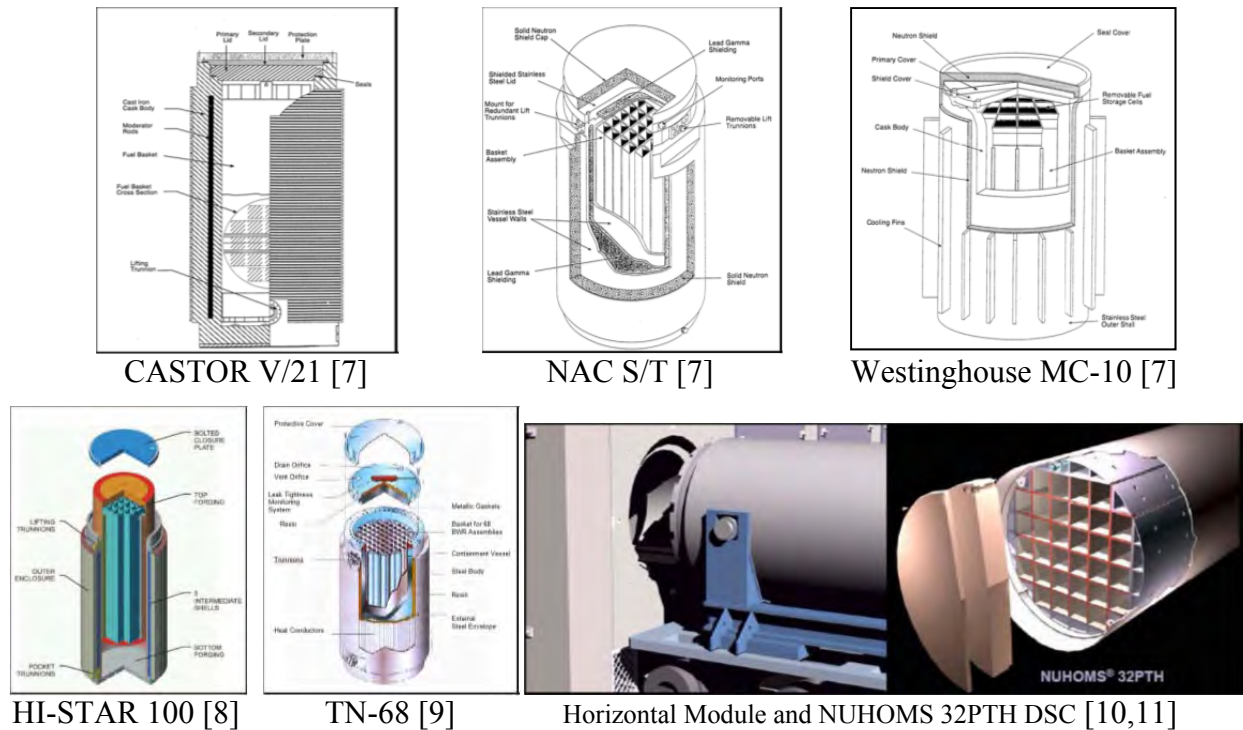
Figure 1.2. Schematics of selected dry storage canisters and systems (old systems).
