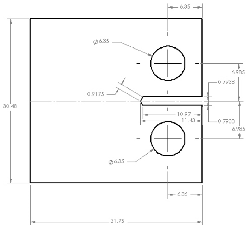
Figure 12 Dimensions of compact tension specimen. All dimensions are in mm.
