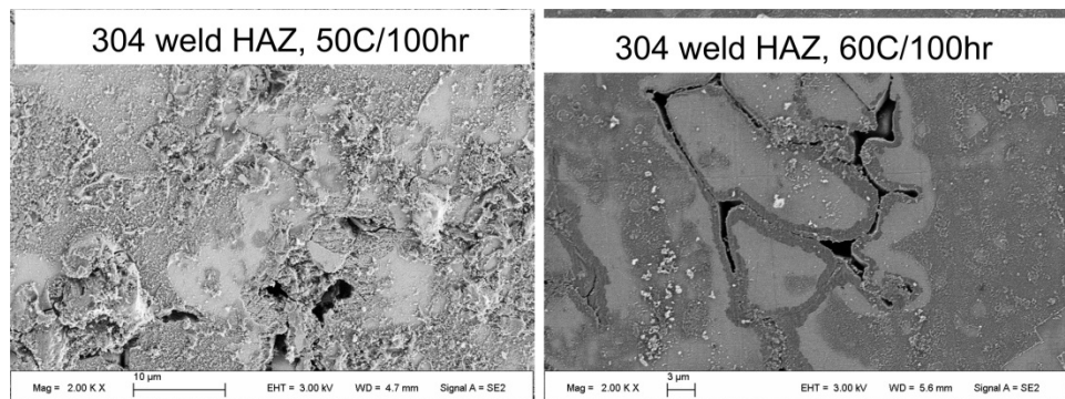
Figure 38. SEM images of heat affected zone of 304 weld material tested in 80% RH at 50°C and 60°C for 100hrs.
