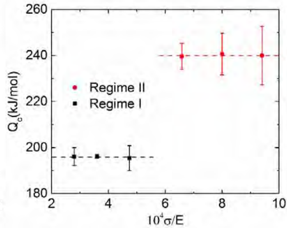
Figure 1.9. Creep activation energy as a function of applied stress in regimes I and II
