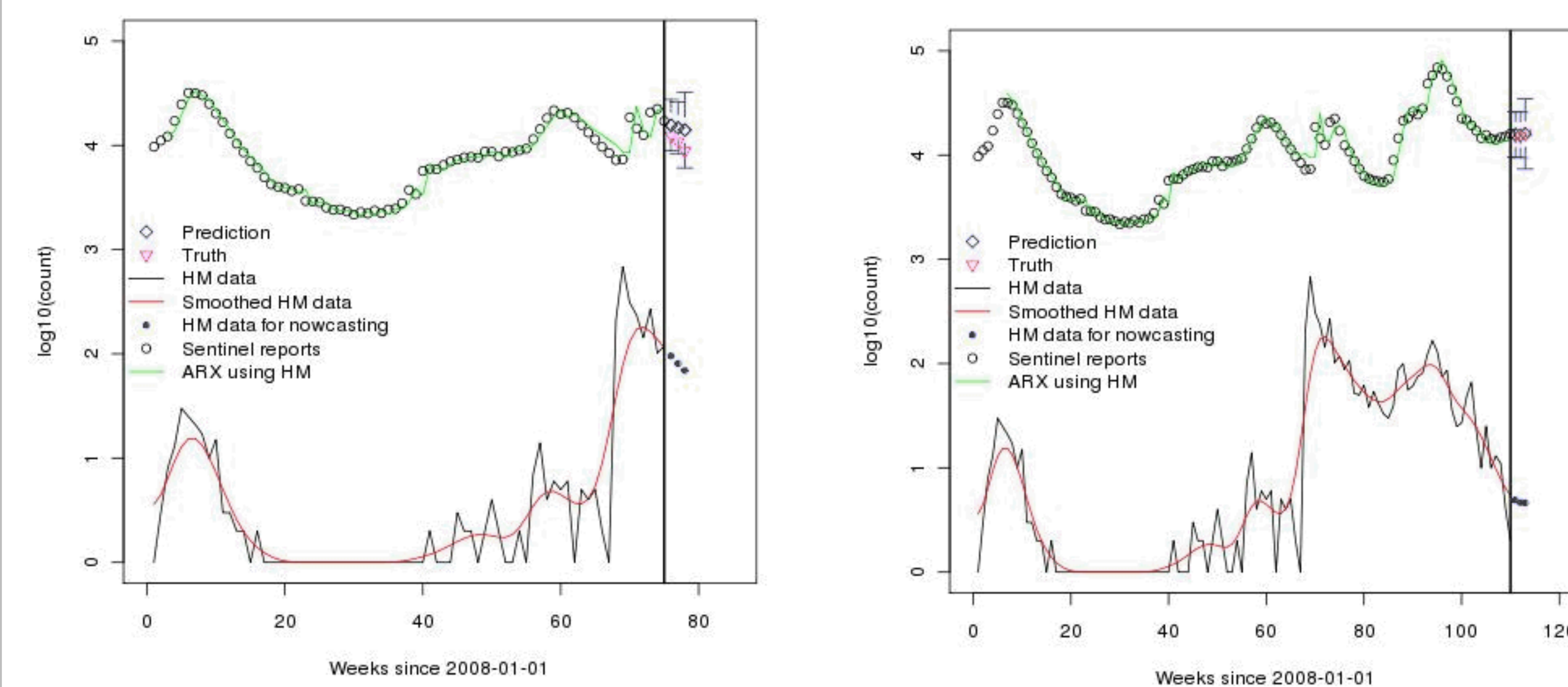
ARIMAX predictions versus ILINet data (training set: 75 weeks)
