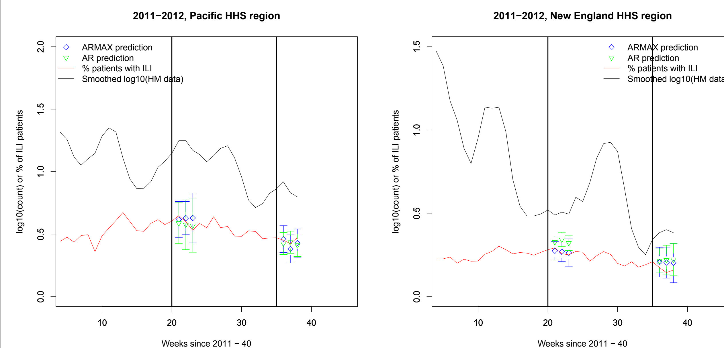
ARIMAX predictions for the pacific region (training set: 35 weeks)
