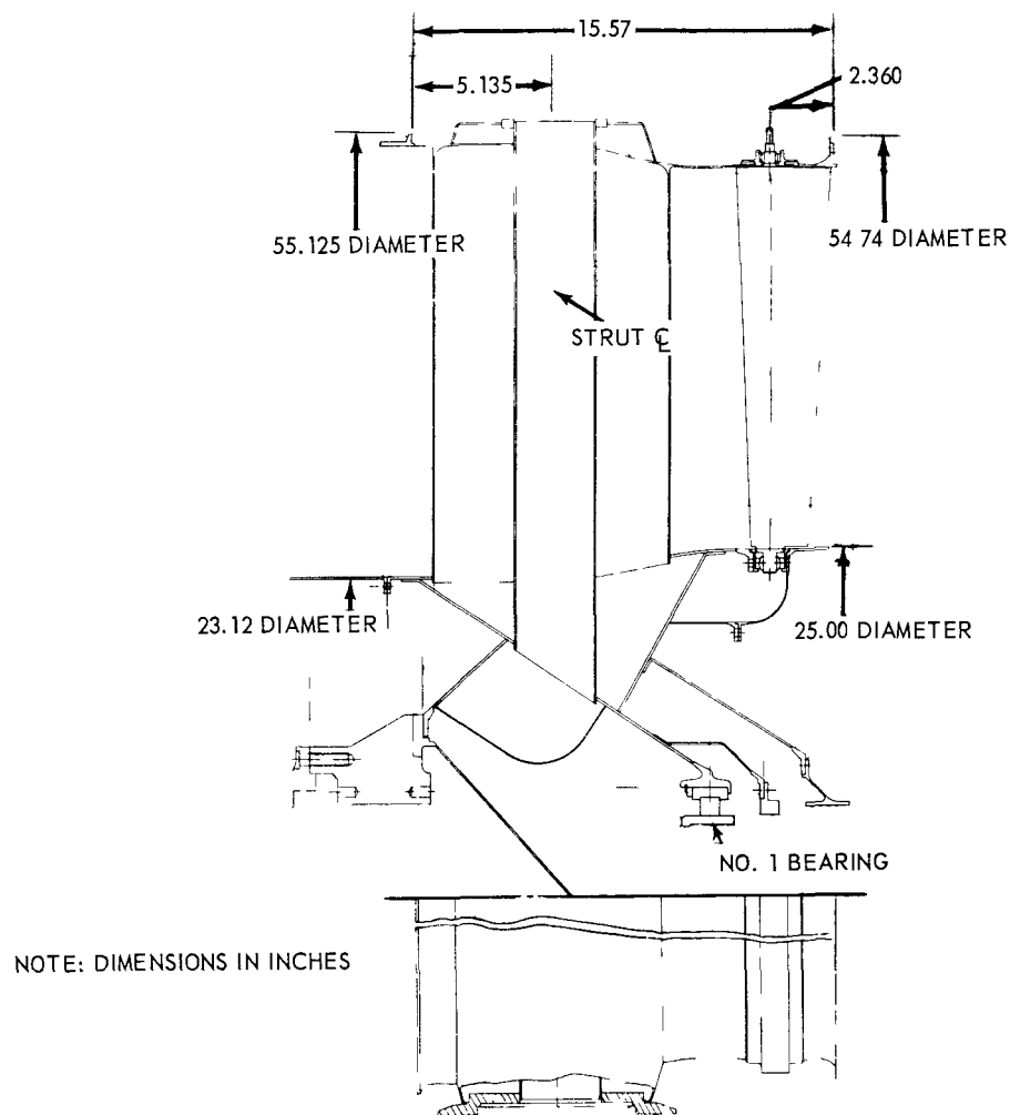
Fig. 6.2—Compressor front frame assembly
