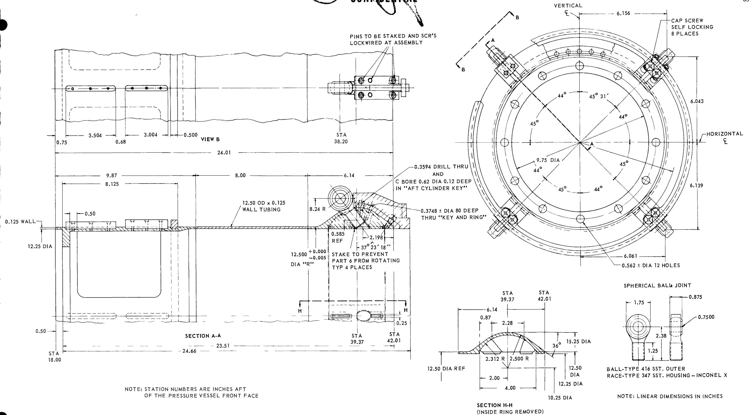
Fig. 5.30—Support structure cylinder (Dwg. 207R829)
