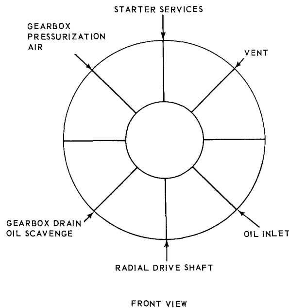
Fig. 6.3—Compressor front frame strut usage
