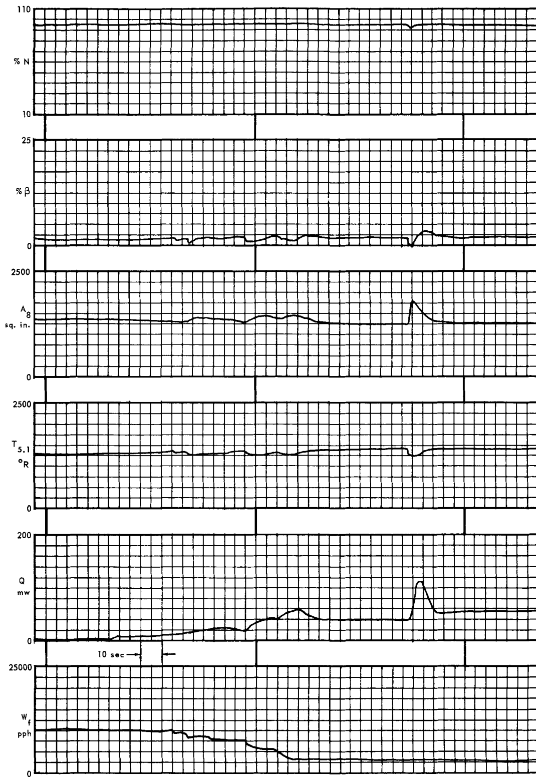
Fig. 7.37a—Analog computer study of power transfer CHO to NHO during ITS hot day conditions
