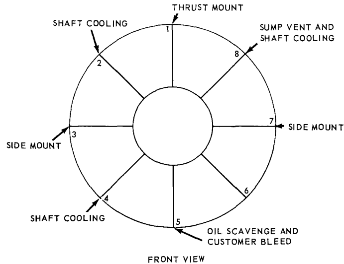
Fig. 6.10 – Compressor rear frame strut usage
