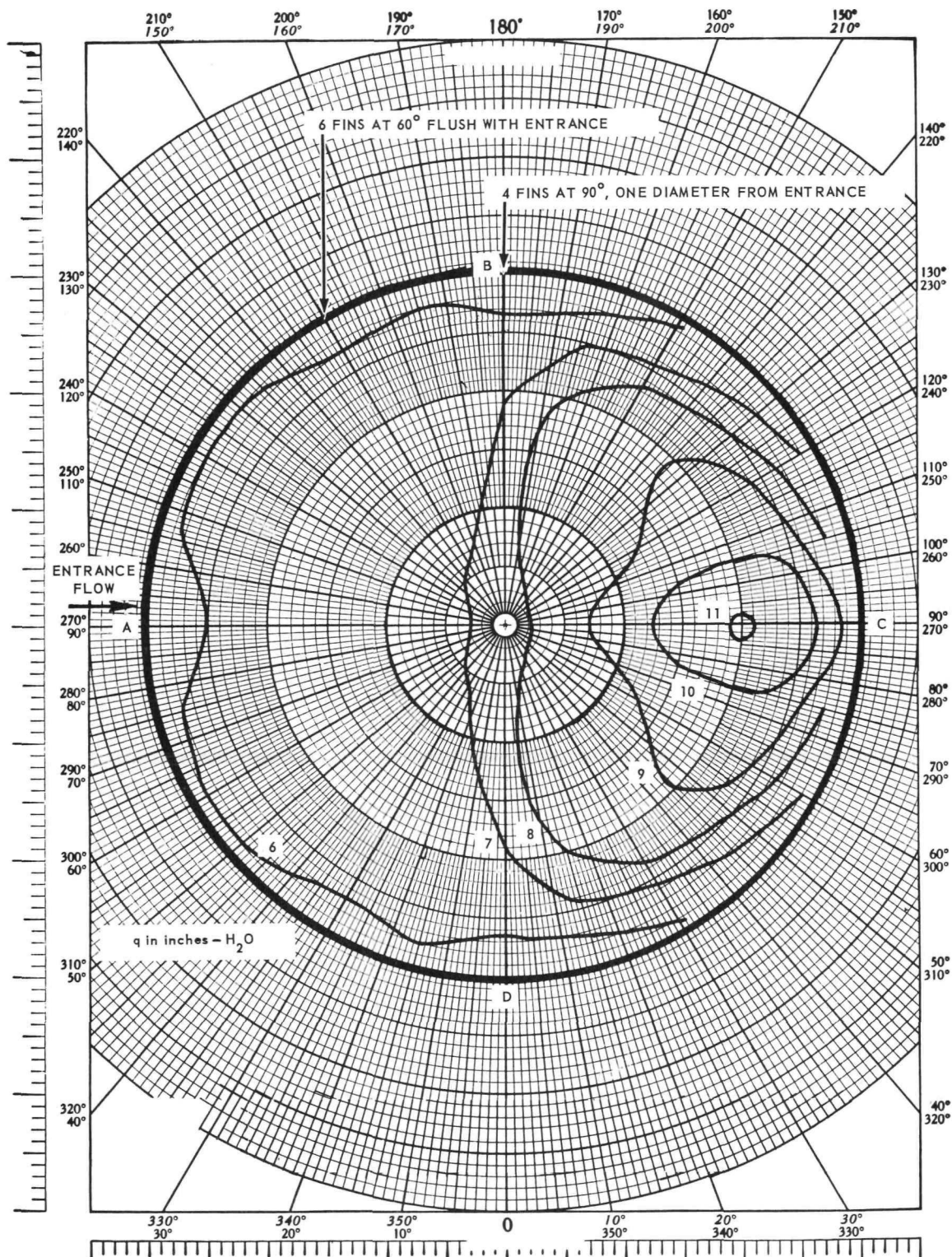
Fig. 3.10—ISO-Q plots from two-dimensional flow results for a tube-in-core location similar to that of tube A35 with nose and fin inserts
