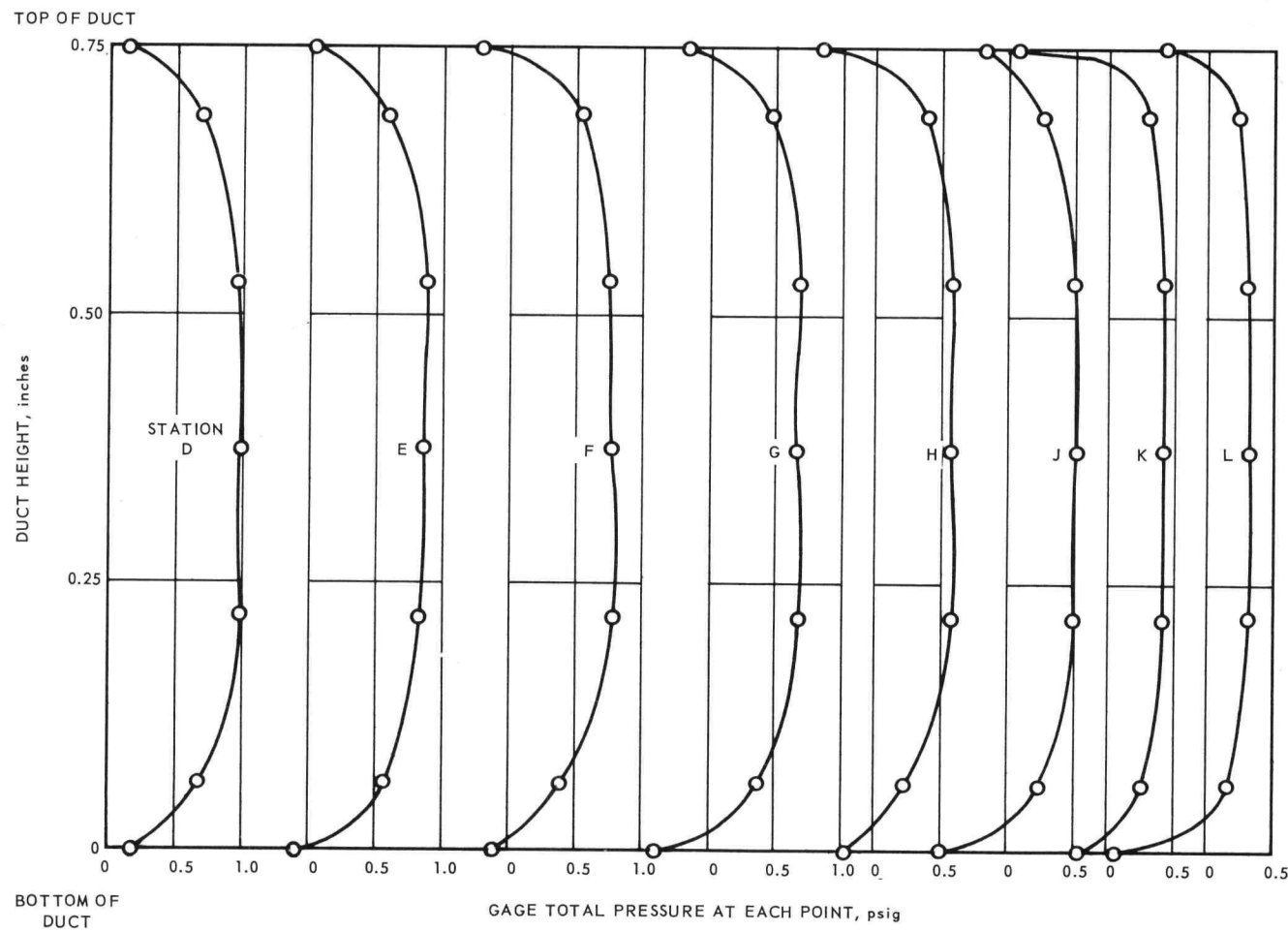
Fig. 3.24 - Front serpentine duct - gage total pressure profiles
