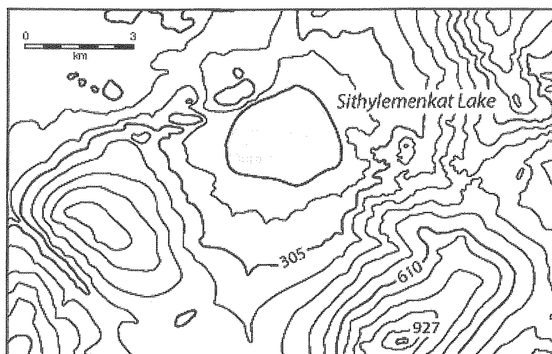
Fig. 6. Sithylemenkat Lake (66.117°N, 151.383°W) at the bottom of a bowl-shaped topographic depression in central Alaska. Contour interval is 30.5 m (100 ft) and the level of the lake is at 219 m (720 ft)
