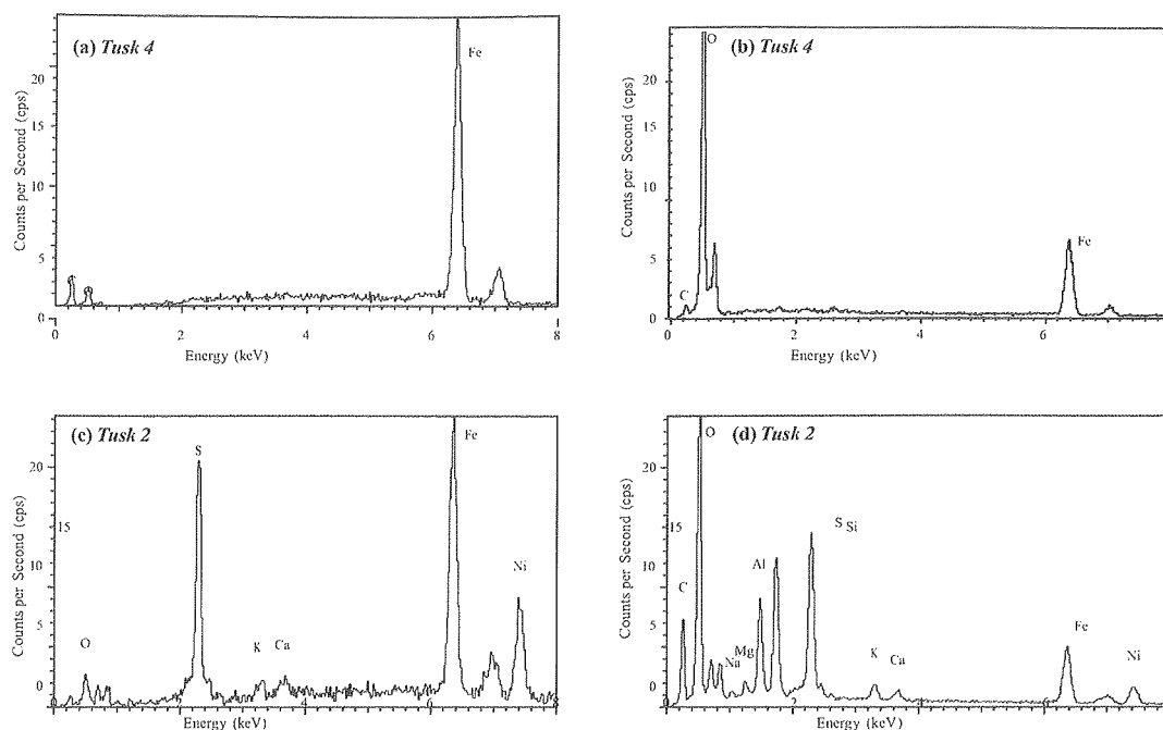
Fig. 3. X-ray fluorescence (XRF) spectra showing the compositional variability within and between particles from two different tusks. Compositions range between native Fe (a), FeO (b), FeNiS (c, d). Silicate compositions in d are probably due to contamination from host sediments during burial
