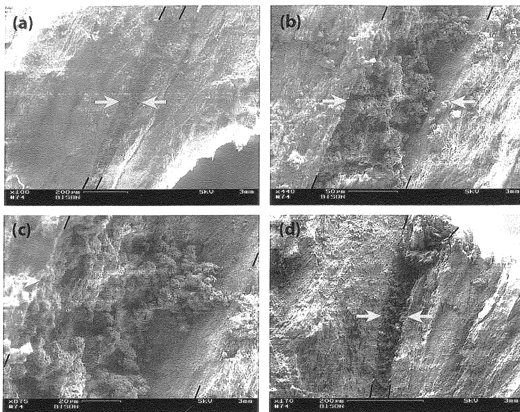
Fig. 5. Scanning electron microscope (SEM) images of a cross section of the bison skull. The particles appear to have formed straight channels (a-c) where particle shards penetrated the bone. Clusters of iron particles at greatest enlargement (c) are seen inside the channel. A second channel is also shown (d). Black line segments and arrows indicate channel walls
