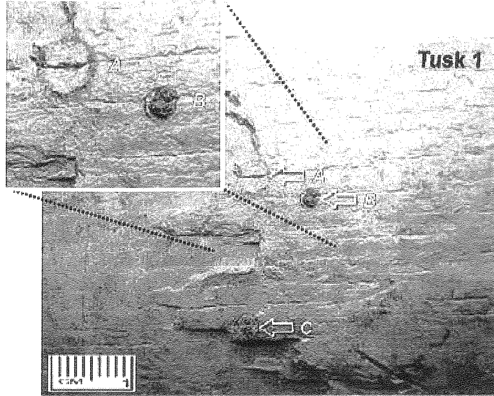
Fig. 1. Close-up photograph and enlargement of metallic particles embedded in tusk 1. Several features can be seen associated with these particles; raised rim (A), "burn" ring (B, C), and bulged center (B)
