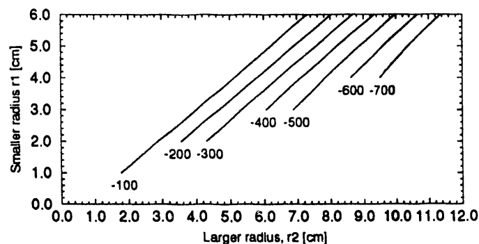
Figure 1: Contours of constant Z/n [i \mu\Omega] , for a RHIC aperture transition with a five-to-one flare.
