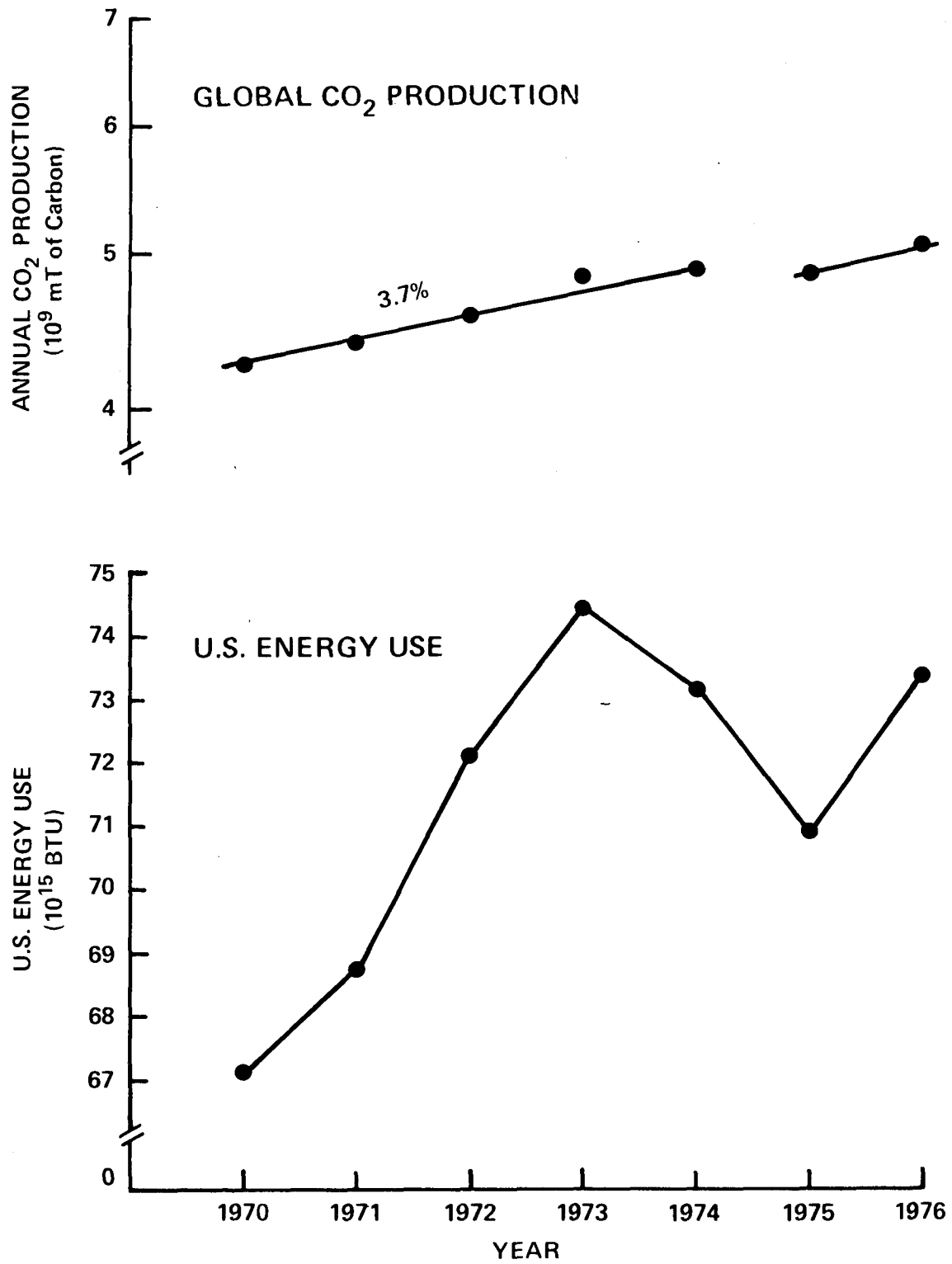
Figure 3: Global CO 2 Production, and U.S. Energy Use, 1970-1976
