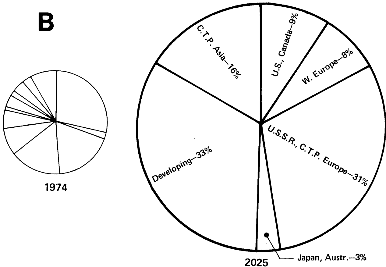
Figure 7: Global CO 2 Production by World Segments.
