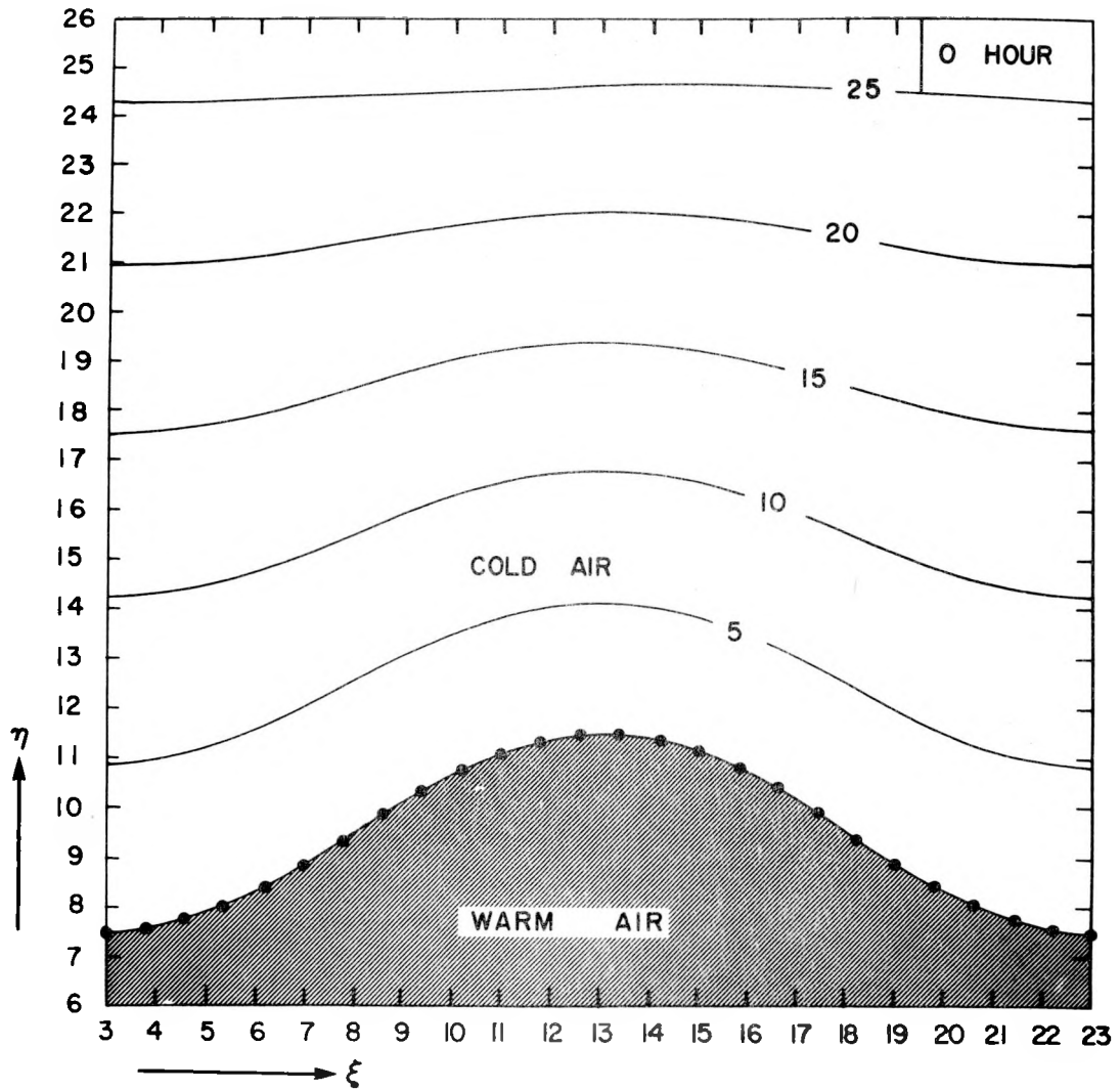
Fig. 8a. Height contour pattern of cold air for Case B at t = 0 , similar to Fig. 6a.
