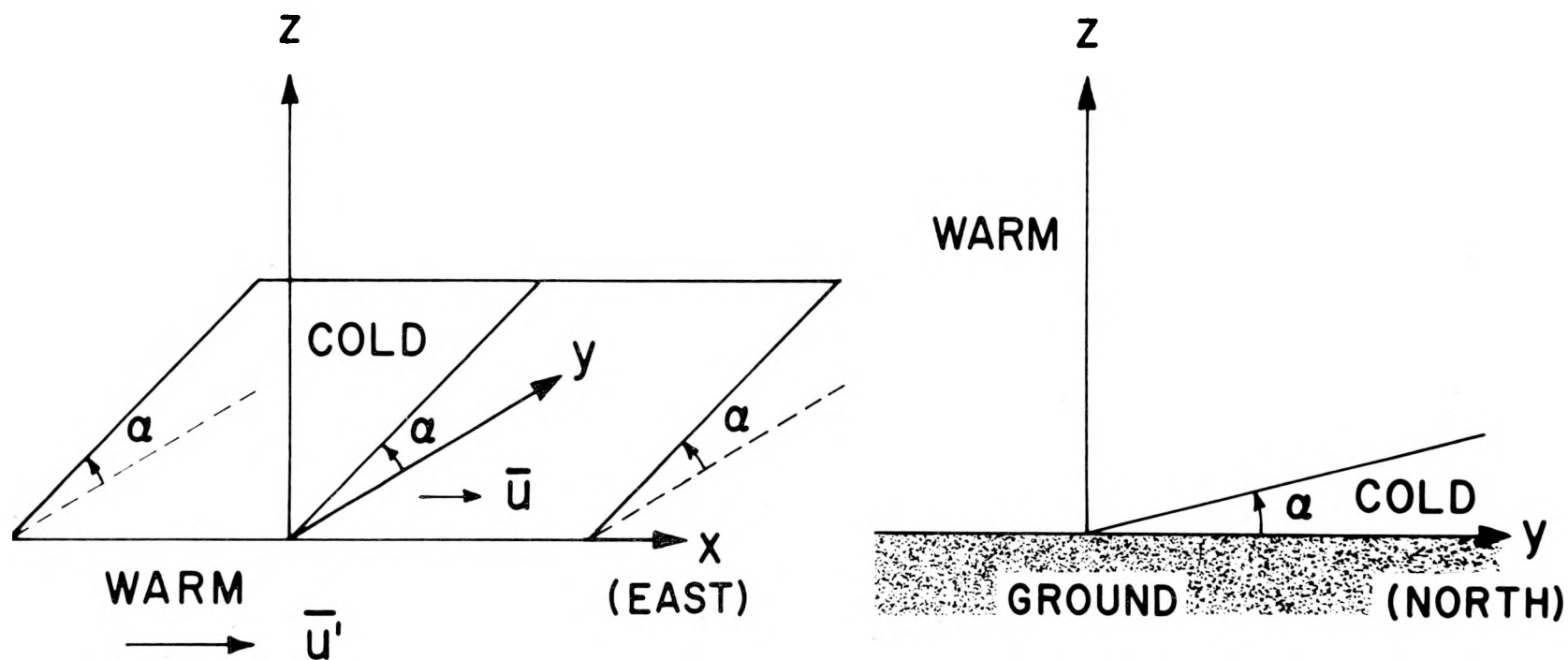
Fig. 1a. A stationary front.
