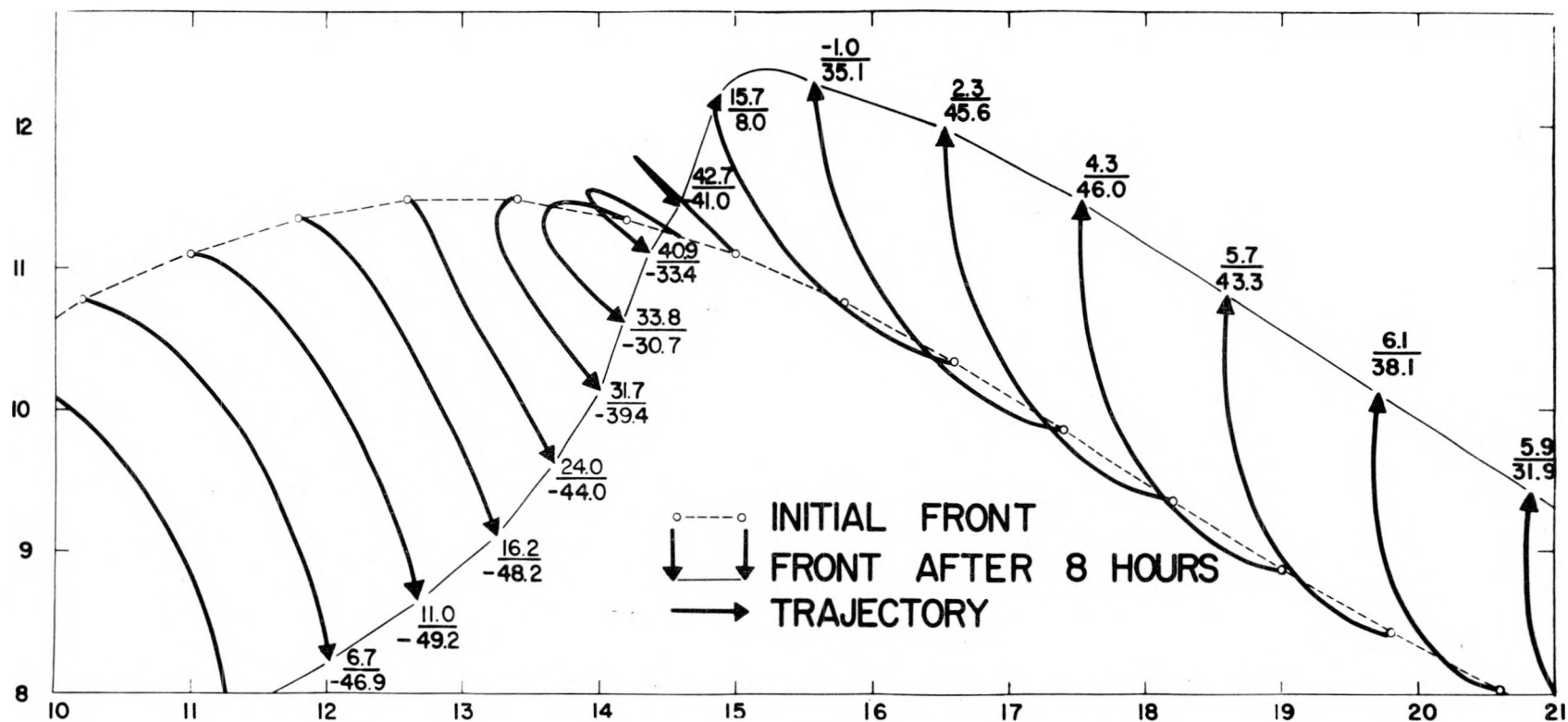
Fig. 7. Trajectories of front points (portion) during the period of 8 hours for Case A.
