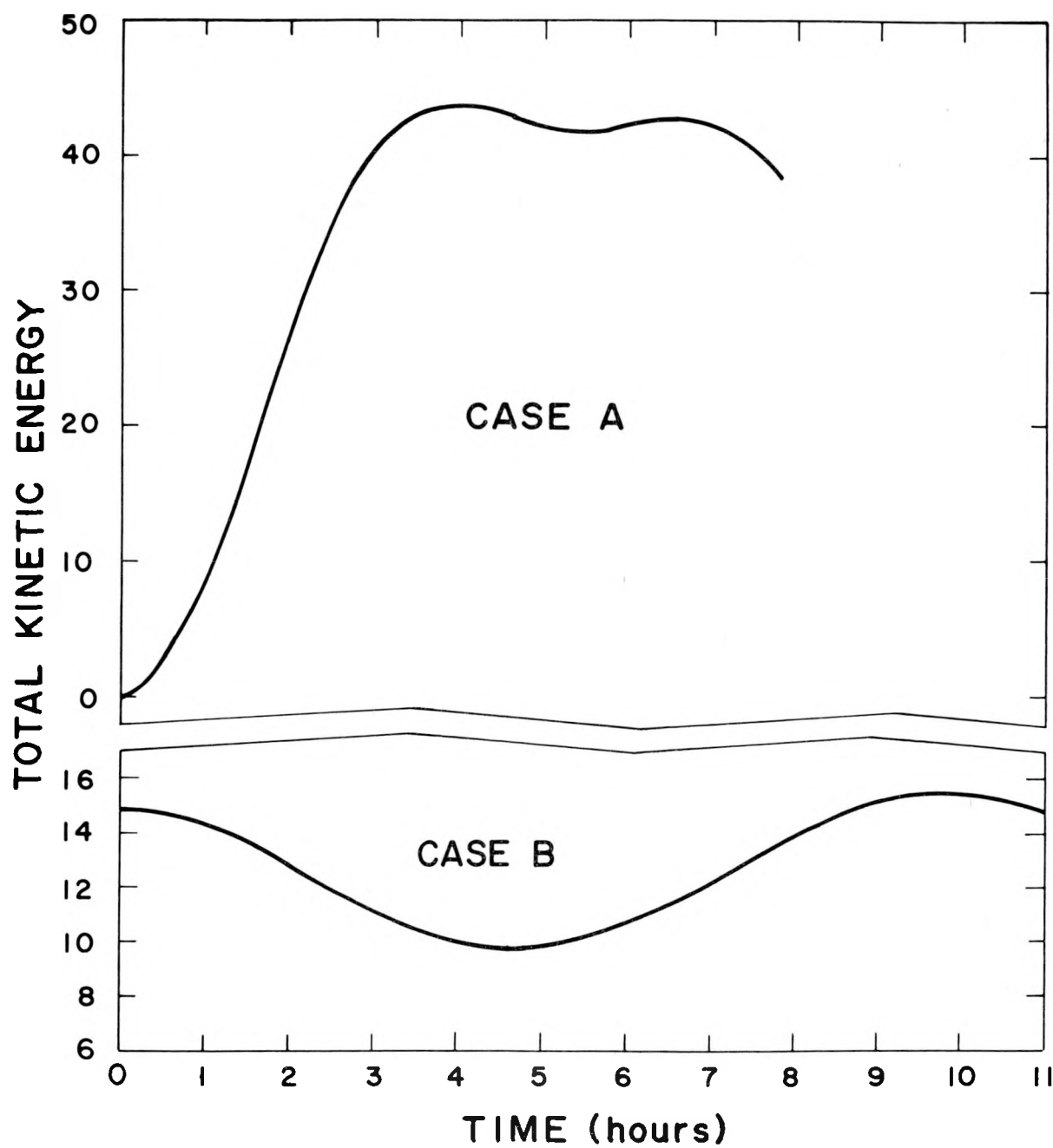
Fig. 10. Total kinetic energy as a function of time. The scale of ordinate is \rho(\Delta s/\Delta t)^2 \times 10^{-2} .
