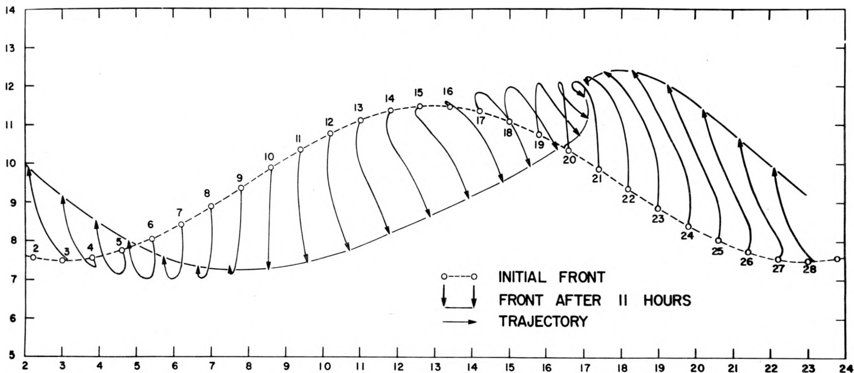
Fig. 9. Trajectories of front points during the period of 11 hours for Case B. Numerals beside each front point are the identification numbers.
