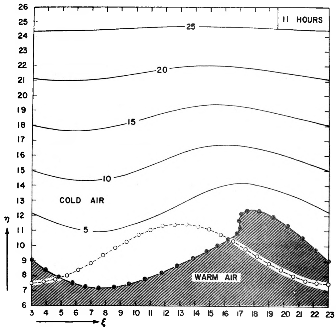
Fig. 8b. Height contour pattern of cold air for Case B at t = 11 hours, similar to Fig. 6b.
