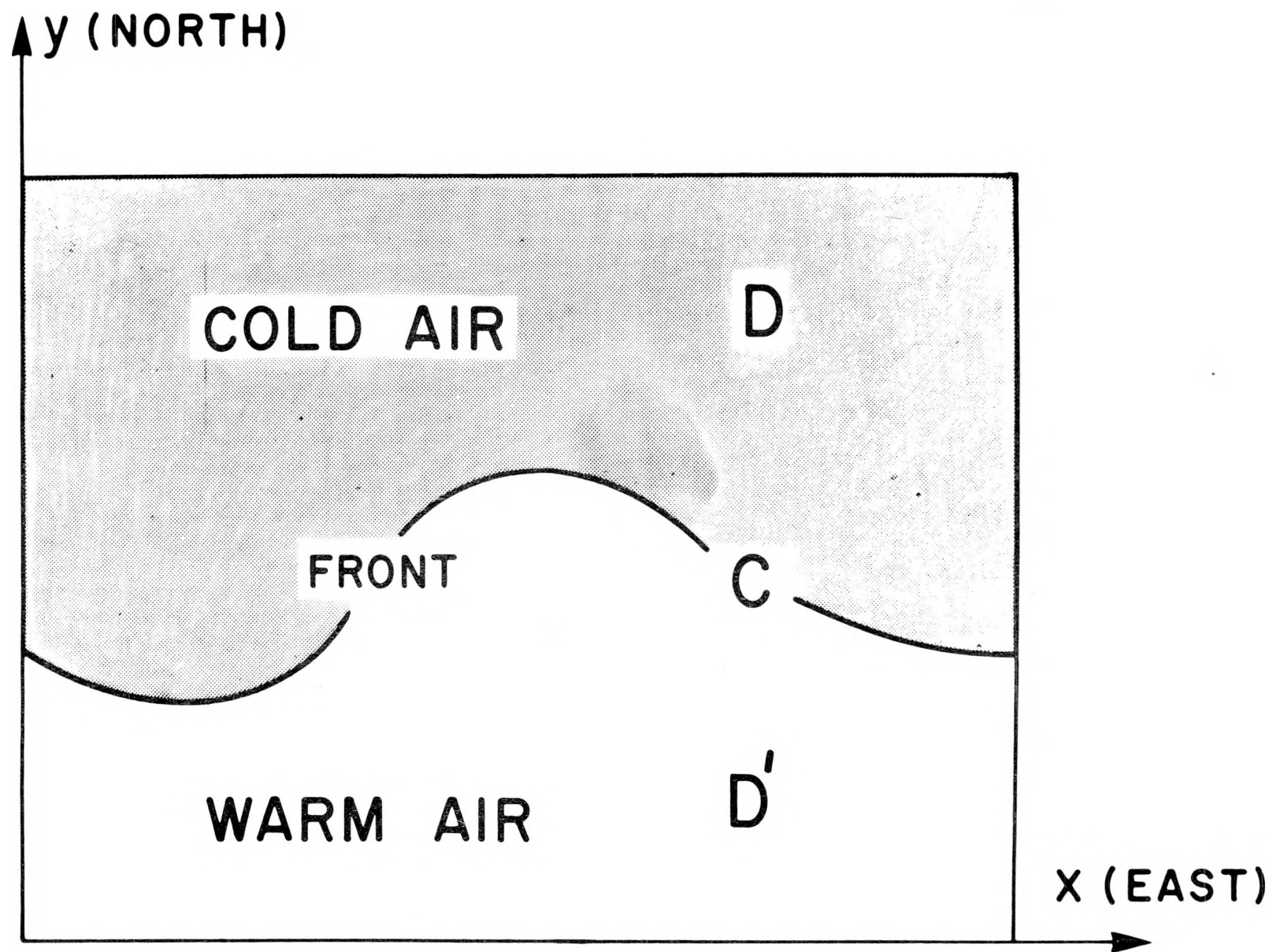
Fig. 3. The rectangular domain of numerical integration.
