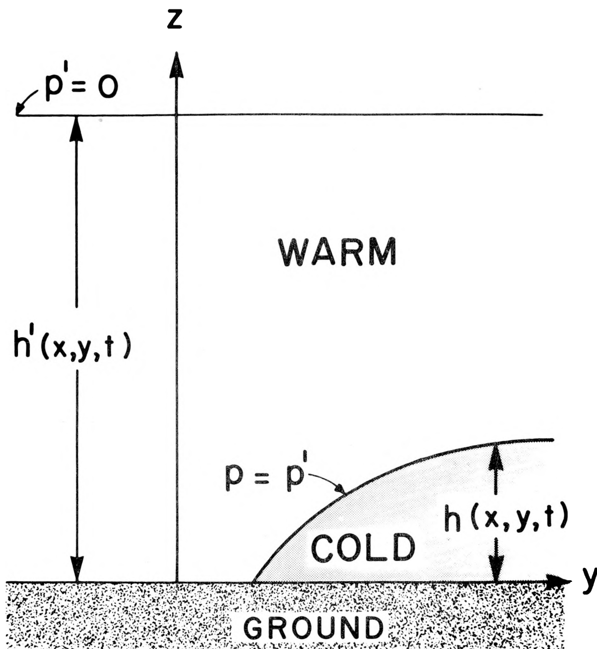
Fig. 1b. Vertical cross-section of the two layers.
