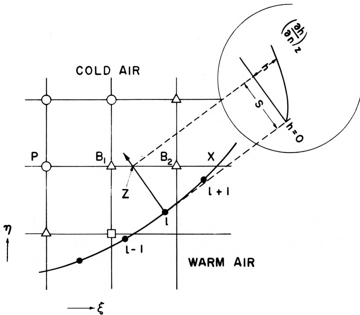
Fig. 5. Evaluation of V_h at the frontal boundary.
