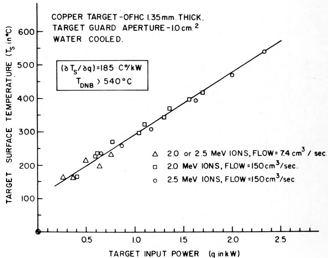
Figure 4. Correlation of target surface temperature data as a linear function of target input power for 1.0 square centimeter beam area.
