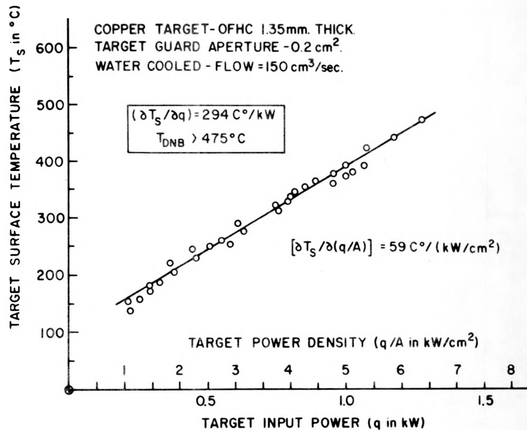
Figure 5. Correlation of target surface temperature data as a linear function of target input power for 0.2 square centimeter beam area.
