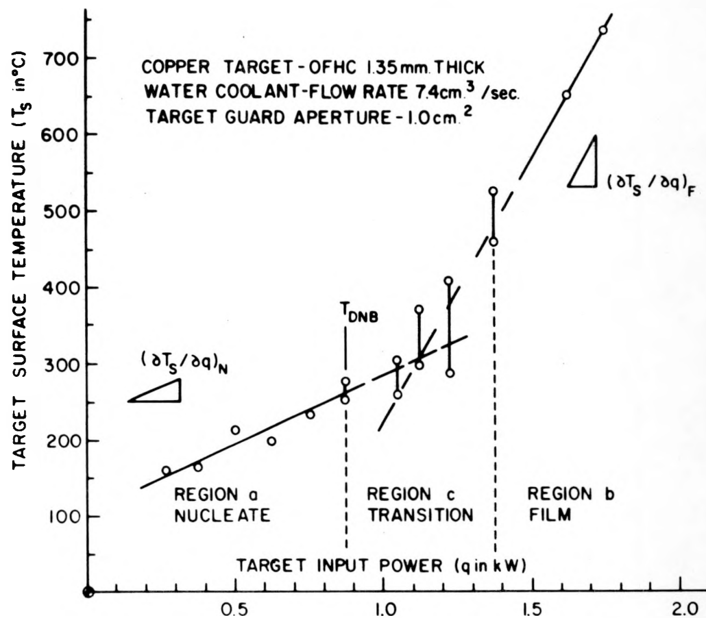
Figure 3. Boiling Regimes. Shown by target surface temperature as a function of target input power at reduced coolant flow rate.
