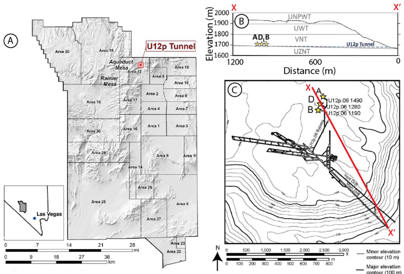
Fig. 1. Map and cross-section views of the testbed within the study area. (a) Location of the Nevada National Security Site, Aqueduct Mesa (red box) which houses U12p Tunnel (P-Tunnel). (b) Cross section of Aqueduct Mesa from X – X' in (c) . The layers correspond to the following lithologies: upper nonwelded to partially welded tuff (UNPWT), upper welded tuff (UWT), vitric nonwelded tuff (VNT), and upper zeolitic nonwelded tuff (UZNT). (c) Topographic contours of Aqueduct Mesa and P-Tunnel Complex. Yellow stars represent the locations of the Physics Experiment 1 (PE1) chemical explosion experiments (PE1-A, -B, and -D). Figure modified from 10 , U.S. Department of Energy technical report prepared by Lawrence Livermore National Laboratory under Contract DE-AC52-07NA27344. Original map created using digital elevation model data within the Generic Mapping Tools (GMT) software 14 .
