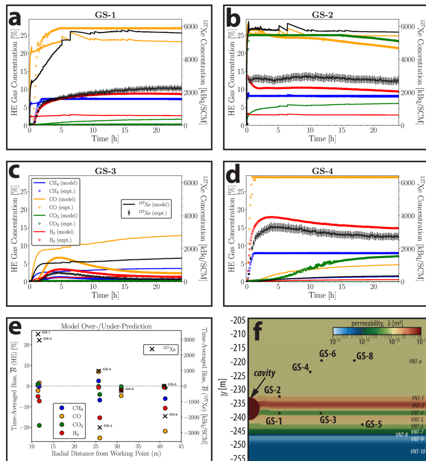
Fig. 3. Composite plot of simulated gas concentrations using permeability values from pre-shot and experimental gas concentrations at proximal boreholes: (a) GS-1, (b) GS-2, (c) GS-3, (d) GS-4; (e) bias (over-/under-prediction; Equation 9) plotted as a function of total distance from the working point and (f) zoomed-in section of model domain showing GS borehole locations. Note that for (a-e) HE byproducts concentrations/bias are represented by circles corresponding to the left y-axis [%] scale, whereas ^{127}\text{Xe} is represented by black “x” markers corresponding to the right y-axis [kBq/SCM] scale. Boreholes GS-6 and 8 are not shown because simulated concentrations are orders of magnitude lower than observed. Borehole GS-5 is not shown because breakthrough concentrations reported by both the experiment and model were negligible.
