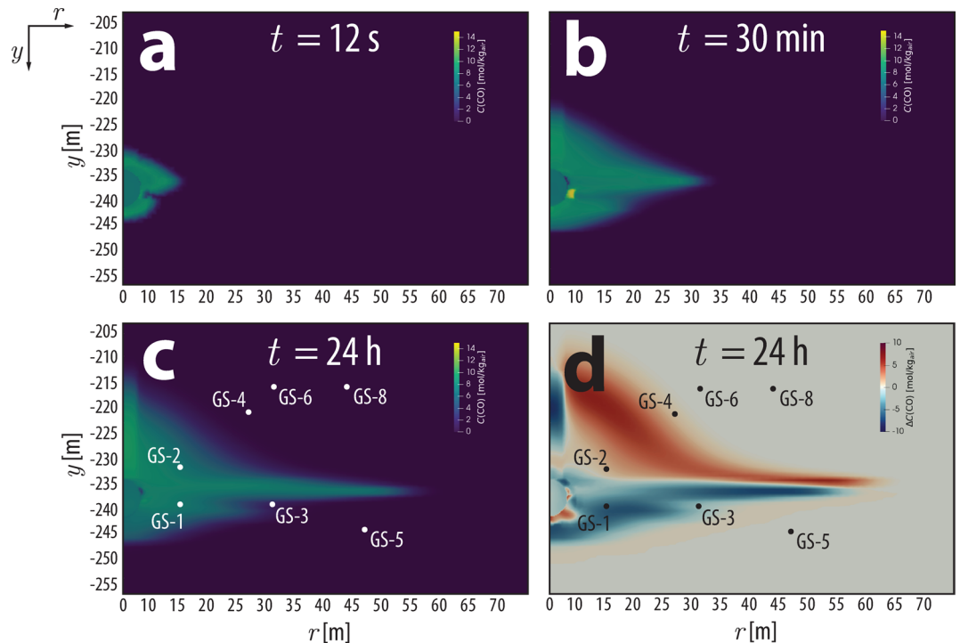
Fig. 4. Time slices of modeled CO gas transport plumes at: (a) 12 s, (b) 30 min, (c) 24 h, and (d) a comparison ( \Delta C_{\text{model}} ) of the CO gas plumes by calculating the difference between simulated results using the pre-shot and post-shot calibrated permeabilities, \Delta C_{\text{model}} = C_{\text{post}}(t) - C_{\text{pre}}(t) .
