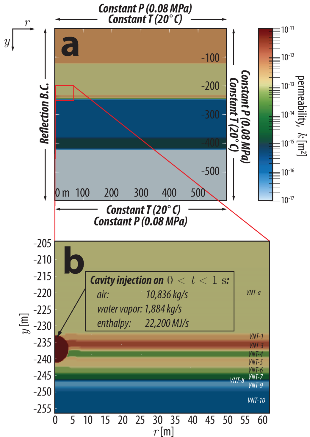
Fig. 2. Schematic of the hydrogeologic framework of the model and boundary conditions for (a) the full extent of the model domain, and (b) inset zoomed into region surrounding the cavity. The injection source terms are distributed uniformly throughout the cavity volume. VNT units in (b) correspond to those in Table 1.
