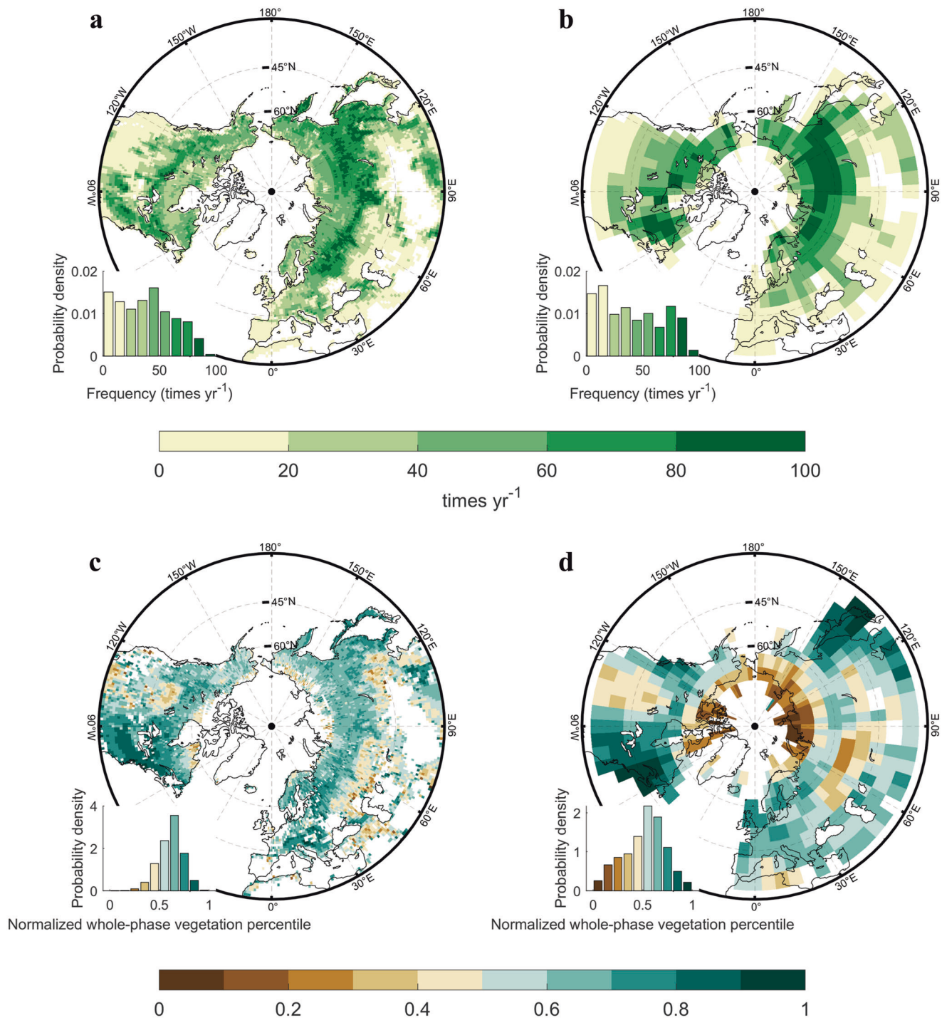
Fig. 1 | Spatial distribution and characteristics of flash flourishing growth events. Ensemble-mean frequency (times yr -1 ) of flash-flourishing events derived from (a) satellite-based observations (CSIF, PKU GIMMS NDVI, MODIS EVI, kNDVI and MODIS LAI) and (b) 18 TRENDY v12 S3 scenario GPP model outputs. Frequencies were
