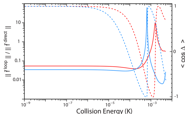
Fig. 6 The solid red and blue curves plot the ratios of the modulus of the looping ( \tilde{f}_{\text{loop}} ) and direct ( \tilde{f}_{\text{direct}} ) scattering amplitudes averaged over the scattering angle as a function of collision energy. The dashed red and blue curves plot the averaged \cos \Delta where \Delta is the phase difference between the two scattering amplitudes. The modulus ratios are specified on the log scale on the left vertical axis and the \cos \Delta values are specified on the linear scale on the right vertical axis. These results are for zero total angular momentum ( J = 0 ) and the red and blue colors correspond to even and odd exchange symmetry, respectively.
