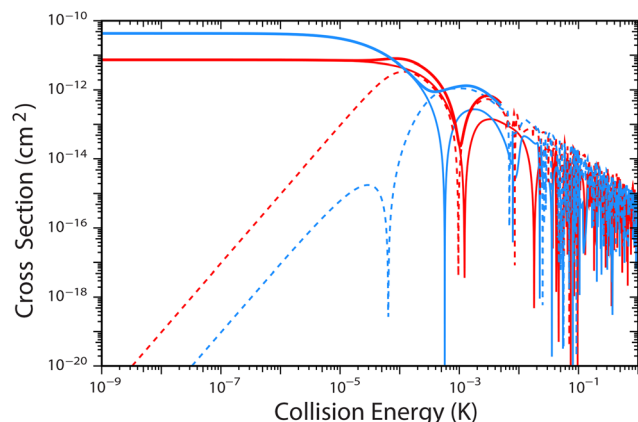
Fig. 4 Elastic cross sections for Rb + KRb ( \nu = 0, j = 0 ) \rightarrow Rb + KRb ( \nu = 0, j = 0 ) are plotted as a function of collision energy. These cross sections are computed on the single adiabatic ground electronic state PES of KRb 2 . The red and blue curves correspond to the even and odd exchange symmetry of the identical Rb nuclei, respectively. The thin solid red and blue curves are computed with total angular momentum J = 0 whereas the dashed red and blue curves correspond to J = 1^- . The thick solid red and blue curves are the total elastic cross sections summed over J = 0 and J = 1^- .
