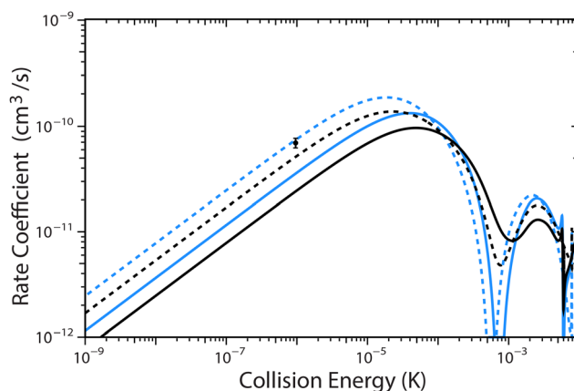
Fig. 7 The total elastic rate coefficients for \text{Rb} + \text{KRb} ( v = 0, j = 0 \rightarrow \text{Rb} + \text{KRb} ( v = 0, j = 0 )) are plotted as a function of collision energy for zero total angular momentum ( J = 0 ). The dashed curves correspond to the calculations on the single adiabatic ground electronic state PES and the solid curves correspond to the 2 \times 2 diabatic calculations. The experimentally measured rate coefficient is the solid black dot with error bars. The black curves include weighted contributions from both the even and odd cross sections that treats all of the nuclear spin states of the two identical Rb nuclei. The blue curves include only the odd cross section and correspond to a single symmetric nuclear spin state (no weights).
