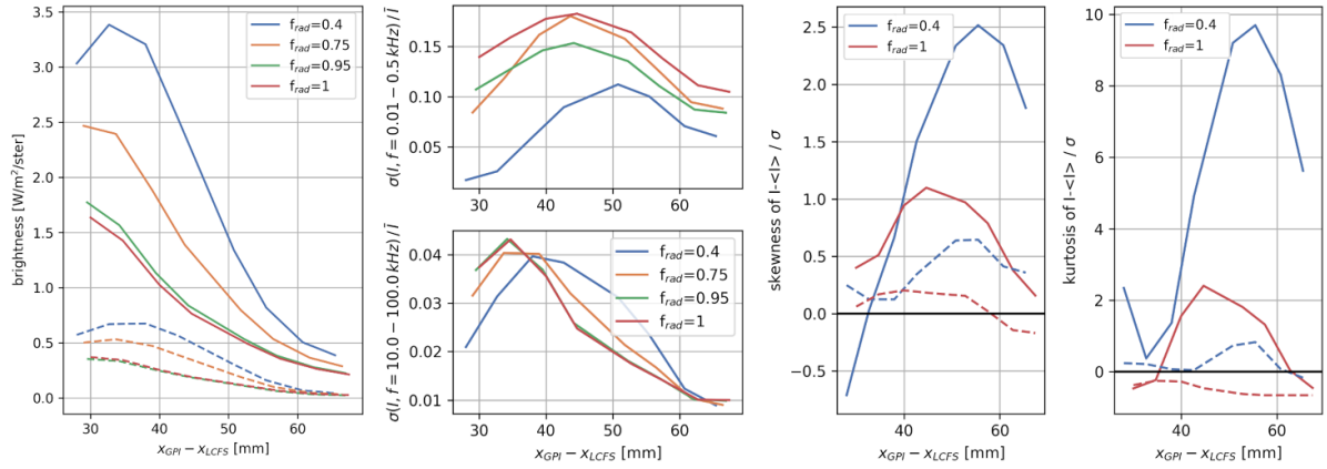
Figure 7. Radial profiles of GPI light emission during the 4 puffs in discharge 20230214.055. Left: Average radial emission profiles (solid) and standard deviation (i.e. fluctuations, dashed). Center: Mean-normalized radial fluctuation profiles in the low (10–500 Hz) and high (10–100 kHz) range. Right: Radial profiles of skewness and excess kurtosis, at two separate poloidal positions (solid: top, dashed: bottom of FOV).
