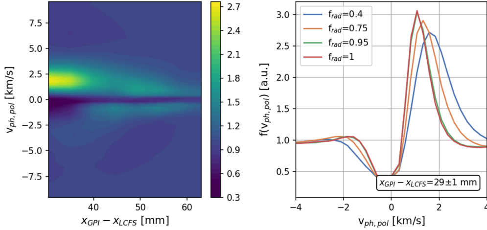
Figure 8. Radial profiles of poloidal phase velocities in discharge 20230214.055 Left: Probability distribution f(v_{ph}) for the first puff at 1.6 s. Right: Cuts of f(v_{ph}) at the innermost radial position for all four puffs.
