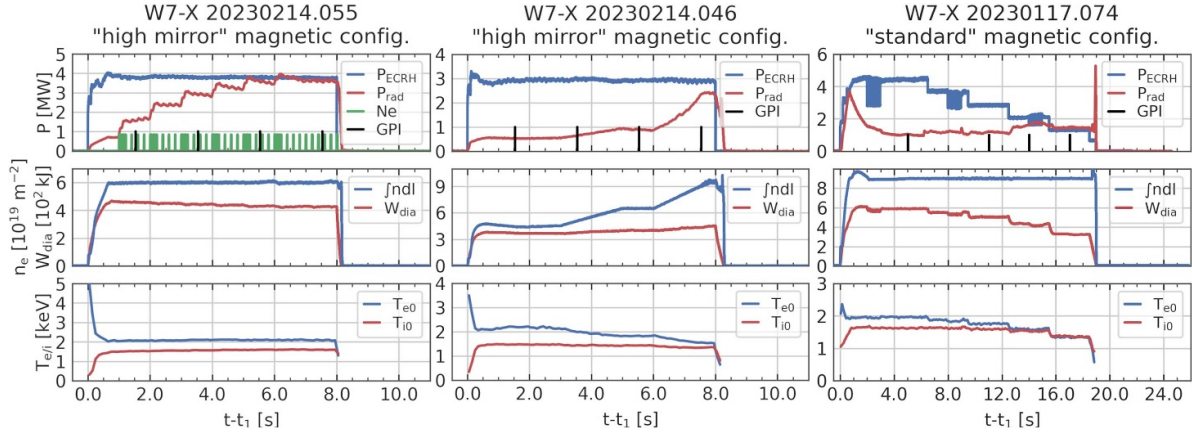
Figure 1. Summary time traces of plasma parameters during three discharges going into detachment. Left: Neon impurity seeding into a steady-state plasma at constant heating power and density into complete detachment around 6 s. Center: Feedback-controlled density ramp (hydrogen puffing) reaching detachment ( f_{rad} \approx 0.8 ). Right: Power step-down at constant density into complete detachment at 16 s.
