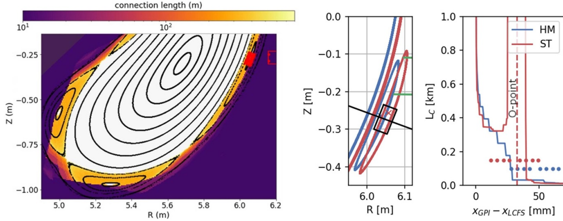
Figure 4. Left: Flux surfaces of the core plasma and magnetic islands at the toroidal angle of GPI over the color-coded magnetic connection length, together with the nozzle position and FOV for the ‘standard’ magnetic configuration. Right: Zoomed GPI FOV together with the last closed flux surface and island position ( x ) in the ‘standard’ (ST, red) and ‘high mirror’ (HM, blue) magnetic configurations with the reciprocating probe paths for the ST configuration (green). Connection length profiles along the image coordinate x_{GPI} , O-point position (dashed) and GPI detector column positions (dots).
