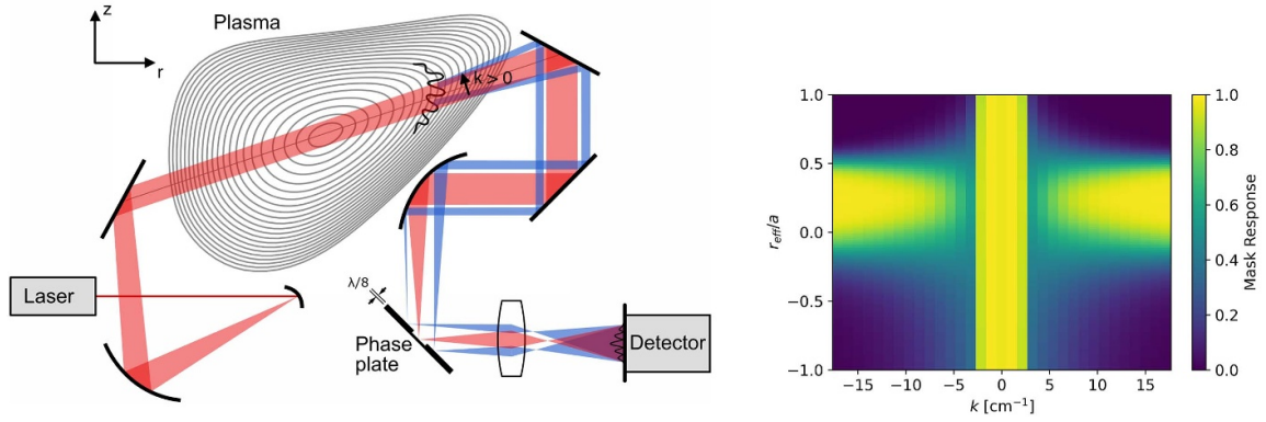
Figure 3. Left: Schematic of the PCI diagnostic including flux surface shapes at its toroidal location. Positive wavenumbers are defined as shown by the k > 0 arrow perpendicular to the line of sight. Right: Radial localization by the spatial selection mask of the PCI system for the angle setting and ‘high mirror’ magnetic configuration used in section 4.1.
