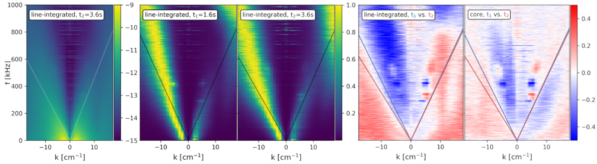
Figure 6. Frequency-wavenumber spectra S(k, f) of density fluctuations measured by PCI in discharge 20230214.055 at the times of two GPI gas puffs, t_1 = 1.6 s and t_2 = 3.6 s. From left to right: (logarithmic) amplitude spectrum S_{int}(k, f, t_2) ; frequency-normalized ('conditional') spectra \bar{S}_{int}(k, f, t_1) and \bar{S}_{int}(k, f, t_2) ; amplitude spectrum differences S_{int}(k, f, t_2) - S_{int}(k, f, t_1) and S_{core}(k, f, t_2) - S_{core}(k, f, t_1) for both PCI detectors.
