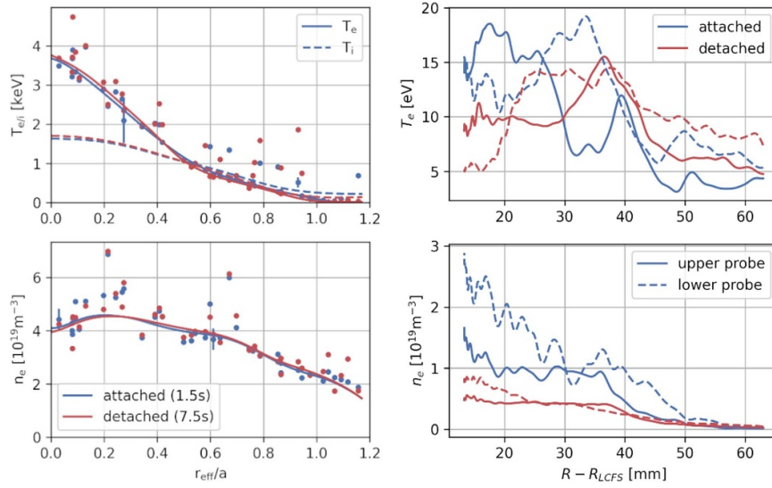
Figure 2. Left: Core kinetic plasma profiles for two time points in discharge 20230214.055, with T_e and n_e as measured by Thomson scattering (points), corresponding fits (solid lines) and T_i (dashed lines) as inverted from XICS data. Error bars are shown for selected representative points. Right: SOL profiles of T_e and n_e measured by reciprocating probes in discharge 20230323.054 at two time points and two vertical positions (solid and dashed lines) described in section 3.
