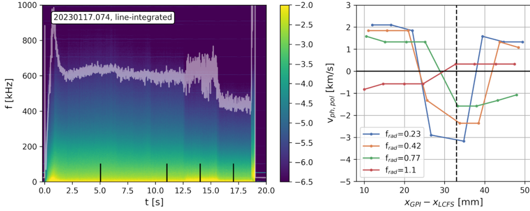
Figure 10. Left: PCI frequency spectrogram and total fluctuation amplitude (white line) from the power step-down experiment 20230117.074. Right: Radial profiles of poloidal velocity from GPI data in the SOL during the same discharge, with the island O-point marked by a dashed line.
