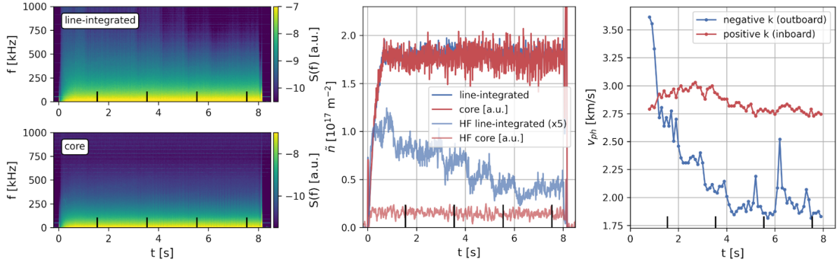
Figure 5. Density fluctuation properties as measured by PCI in discharge 20230214.055. Left: Frequency spectrograms from both detectors (line-integrated and masked for core fluctuations only) with time points of GPI measurements marked (black bars). Center: Total fluctuation amplitudes from both detectors (solid), absolutely calibrated for the line-integrated case, and (scaled-up) high-frequency components above 600 kHz (semi-transparent). Right: Time evolution of dominant fluctuation phase velocities with positive (inboard) and negative (outboard) wavenumbers.
