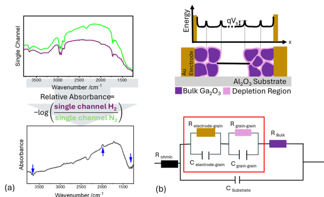
Fig. 2 (a) Schematic of the calculation used to calculate the relative absorbance spectra. (b) Schematic representation of the Ga 2 O 3 depletion layer and the corresponding equivalent circuit.
