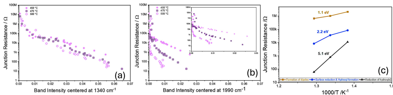
Fig. 7 (a) IR band intensity centred at 1340\text{ cm}^{-1} (associated with surface reduction) is plotted against the inter-junction resistance. (b) IR band intensity centred at 1990\text{ cm}^{-1} (associated with surface hydrides) is plotted against the inter-junction resistance. (Inset) Enlarged view of band intensity at 1990\text{ cm}^{-1} vs. inter-junction resistance. (c) Arrhenius plots of the inter-junction resistance in three different concentration regions.
