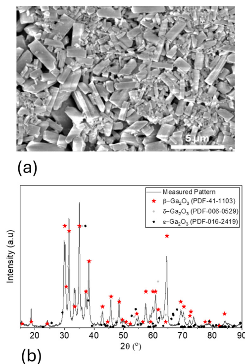
Fig. 3 (a) SEM image of the Ga 2 O 3 sensitive layer surface is shown. (b) Pattern match analysis of β-Ga 2 O 3 .
