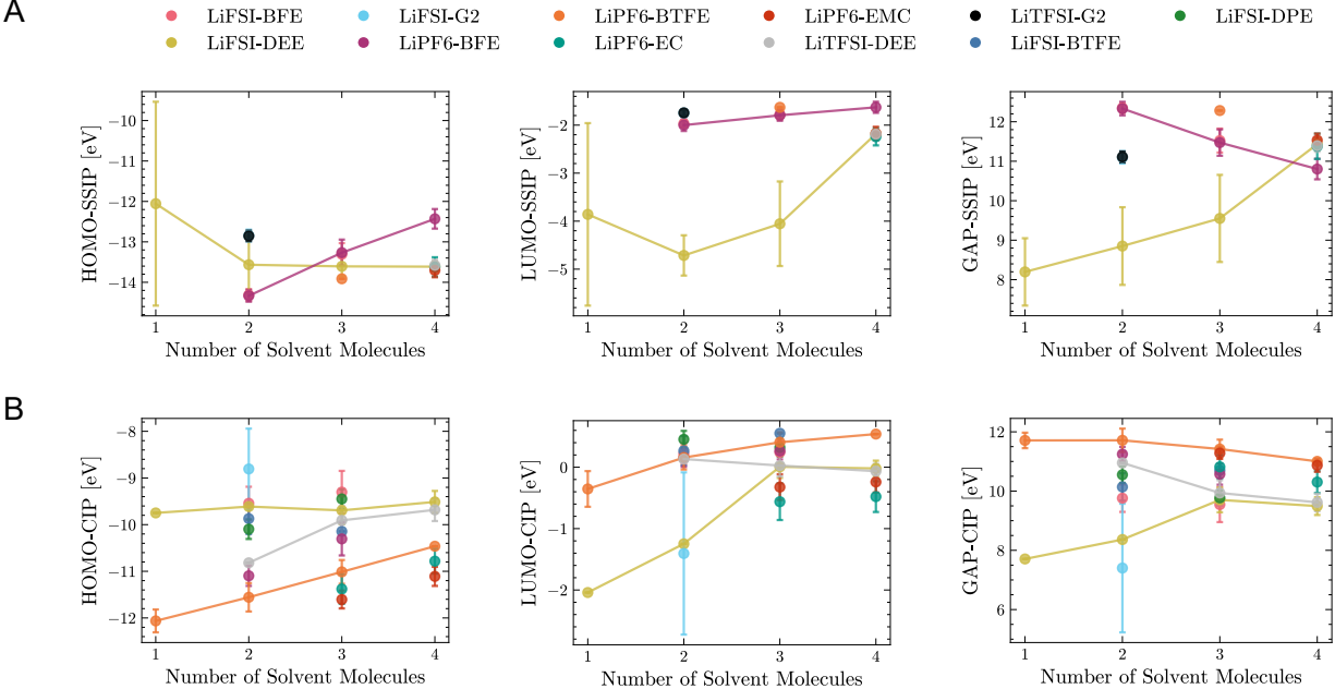
Figure 4: Desolvation analysis. (A) HOMO, LUMO, and HOMO-LUMO gap as a function of number of solvents in the primary solvation shell for freely solvated Li-ions. Lines are drawn for the systems most sensitive to desolvation (LiFSI-DEE, LiPF 6 -BFE) for highlighting purposes. (B) HOMO, LUMO, and HOMO-LUMO gap as a function of number of solvents in the primary solvation shell for CIPs. Again, lines are drawn for the systems most sensitive to desolvation in the CIP configuration, which include LiFSI-DEE, LiPF 6 -BTFE and LiTFSI-DEE.
