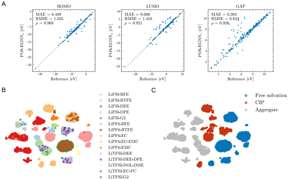
Figure 2: Robustness analysis of ML model prediction. (A) Parity plots comparing the predicted HOMO, LUMO energies, and the HOMO-LUMO gap across the OMol25 Li-ion battery electrolyte test set for the small model. (B, C) t-SNE projection of Li-ion node embeddings color-coded by chemical composition (B) or solvation structure (C).
