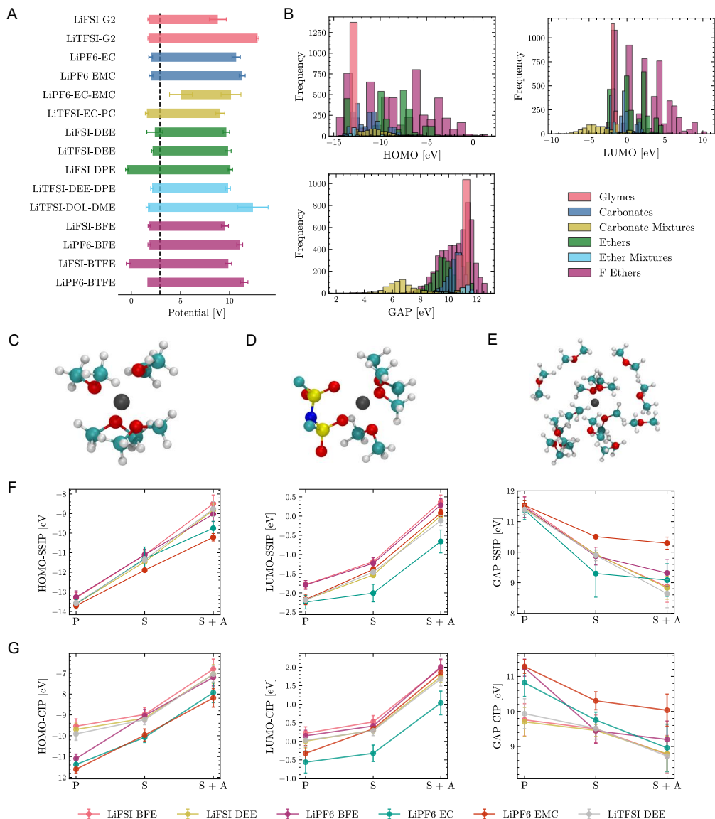
Figure 3: Correlation analyses. (A) Electrochemical stability windows of relevant Li-ion battery electrolytes. Colored bars denote the potential ranges over which the electrolyte is predicted to be stable, with the left and right edges corresponding to the cathodic and anodic limits, respectively. The vertical dashed black line marks the reference lithium metal Fermi energy at -2.91 eV, while the error bars reflect variations in the predicted HOMO and LUMO levels of solvated species arising from different coordination environments. (B) Histograms of HOMO, LUMO, and HOMO-LUMO gap for solvation structures color-coded by solvent class. (C) Representative snapshots of freely solvated Li-ion in DEE, extracted from MD simulation. (D) Representative snapshot of CIP configuration (Li-FSI in DEE). (E) Representative snapshot of secondary solvation shell of Li-ion in DEE. (F, G) Variations in HOMO, LUMO, and HOMO-LUMO gap as a function of the solvation shell size and composition, where P refers freely solvated Li-ion (primary solvation), S denotes secondary solvation environment and S + A represents secondary solvation with an anion species included.
