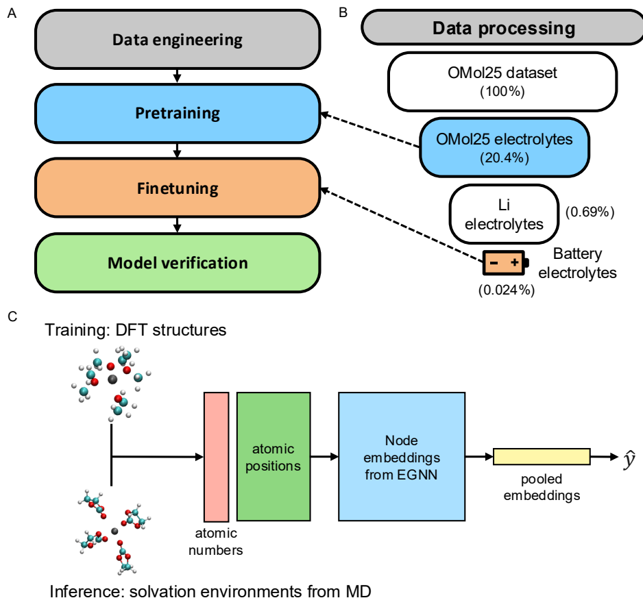
Figure 1: ML training protocol. (A) Overview of workflow from data engineering to model training and verification. (B) Data processing. (C) Model training and inference.
