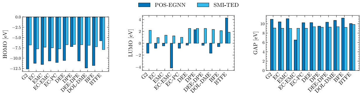
Figure 5: Comparison of mean predictions obtained from the POSEGNN model and the SMI-TED model
