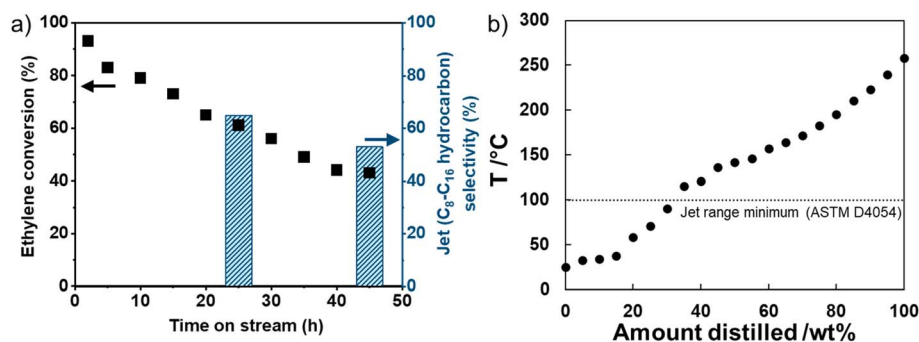
Fig. 5 (a) Ethylene conversion (black square) and jet ( C_8 - C_{16} olefins) selectivity (blue bar) obtained during mixed olefin oligomerization ( T = 250 °C; P = 21 bar; WHSV = 0.7\text{ h}^{-1} ) and (b) simulated distillation (ASTM D2887) of isoparaffin products of olefin oligomerization and hydrotreating (samples corresponding to 25 h demonstrated in Fig. 3a was used herein for analysis).
