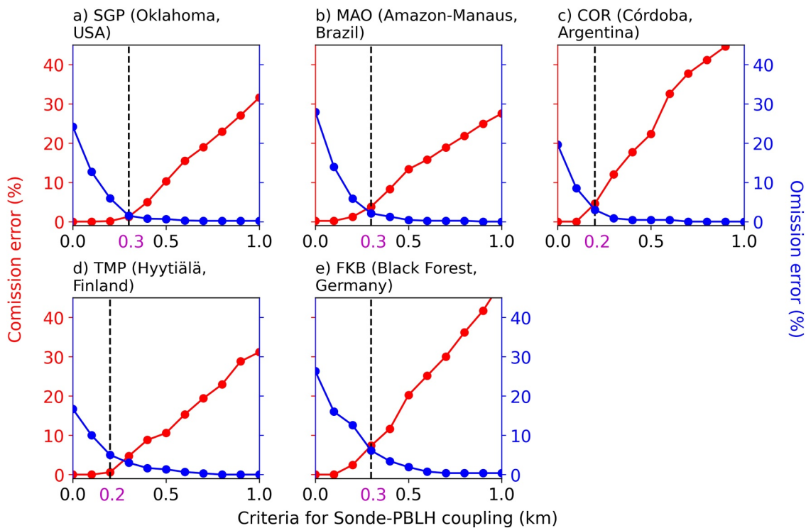
Figure 1. The commission and omission errors as a function of the coupling thresholds used at the five ARM sites. The dashed line indicates where the commission and omission errors are crossover of the same magnitude. The number in magenta is the coupling threshold.
