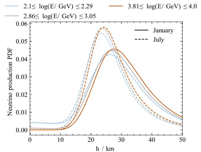
Fig. 2 Neutrino production profiles for January 1st (solid) and July 1st (dashed) for the neutrino sample from the IceCube Neutrino Observatory, integrated over the zenith range from 90^\circ to 110^\circ calculated using MCEq with the NRLMSISE-00 atmospheric model. The profiles in this figure are displayed for the first, fifth and highest energy bin
