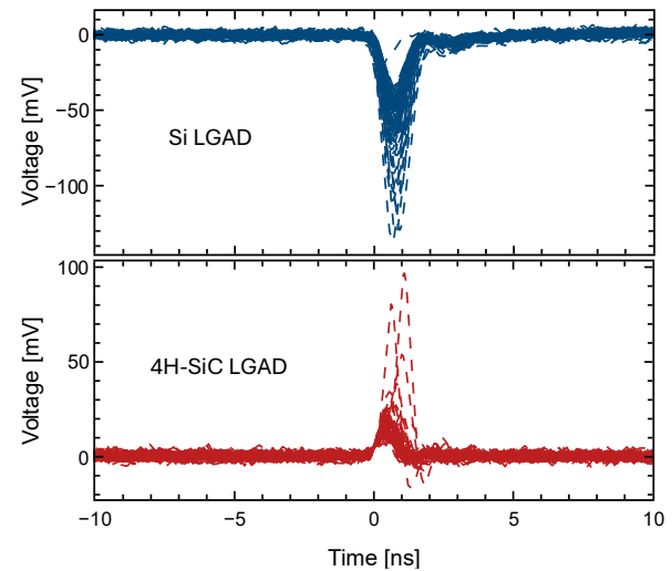
Fig. 5. Sampled waveforms with the ^{90}\text{Sr} source: (a) pulse signal detected by the Si LGAD; (b) pulse signal detected by the 4H-SiC LGAD.
