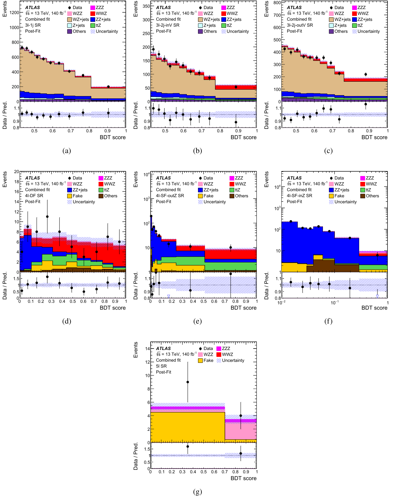
Fig. 3. Comparison of the BDT distribution between data and predictions for the (a) 3 \ell -1j, (b) 3 \ell -2j-inV, (c) 3 \ell -2j-outV, (d) 4 \ell -DF, (e) 4 \ell -SF-outZ, (f) 4 \ell -SF-inZ, and (g) 5 \ell SRs. The bottom panel shows the ratio of the data and SM predictions. The uncertainty band includes both statistical and systematic uncertainties obtained by the fit.
