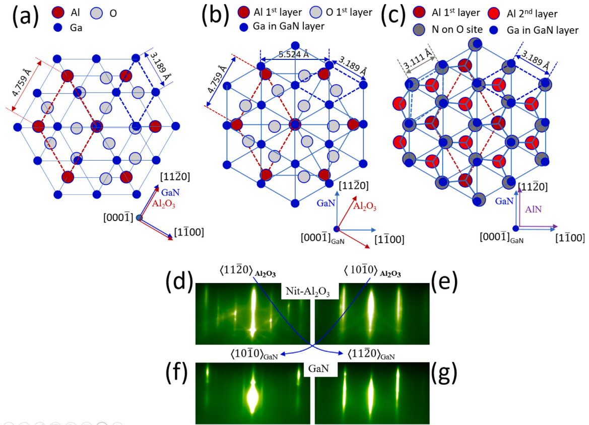
Fig. 1. Modeling GaN growth on sapphire with and without lattice rotation and plasma nitridation: (a) GaN lattice ( a_{\text{GaN}(0001)} = 3.189 \text{ \AA} ) on sapphire lattice ( a_{\text{Al}_2\text{O}_3(0001)} = 4.759 \text{ \AA} ), illustrating a lattice mismatch of -33.0\% ; sapphire and GaN surface unit cells are shown by dashed lines. Only 1st layer Al sites are shown to indicate the surface unit cell lattice of \text{Al}_2\text{O}_3 ; the O sublattice is 30^\circ misaligned to the Al sublattice as well as with the Ga (of GaN) sublattice overlaid; (b) GaN(000 \bar{1} ) lattice rotated 30^\circ on \text{Al}_2\text{O}_3 (0001) reduces the lattice mismatch to +16.0\% with a_{\text{Al}_2\text{O}_3(0001)} = 4.759 \text{ \AA} and \sqrt{3} a_{\text{GaN}(0001)} = 5.524 \text{ \AA} ; sapphire and GaN surface unit cells are shown by dashed lines; (c) after rf plasma nitridation of the \text{Al}_2\text{O}_3 substrate surface, illustrating the formation of an AlN-like surface and subsequent reduction of lattice mismatch to +2.49\% with a_{\text{AlN}(0001)} = 3.111 \text{ \AA} ; both 1st and 2nd layer Al atom are shown as well as N atoms on O sites; sapphire, AlN, and GaN surface unit cells are shown by dashed lines; (d,e) RHEED patterns of nitridated \text{Al}_2\text{O}_3 surface before GaN growth; and (f,g) RHEED patterns along the same beam directions after GaN growth.
