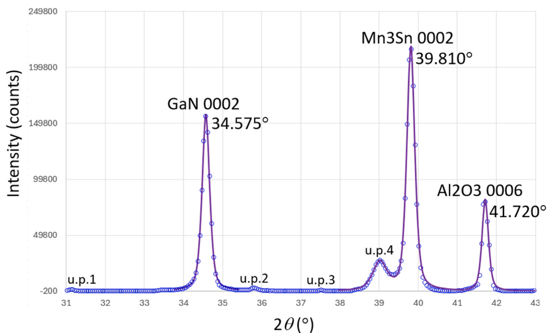
Fig. 7. X-ray diffraction pattern of \text{Mn}_3\text{Sn}/c\text{-plane GaN}/\text{Al}_2\text{O}_3 . The primary peaks seen are the 0002 for \text{Mn}_3\text{Sn} , the 0002 for GaN, and the 0006 for \text{Al}_2\text{O}_3 . Other minor unknown peaks (u.p.'s) are seen and described in the text.
