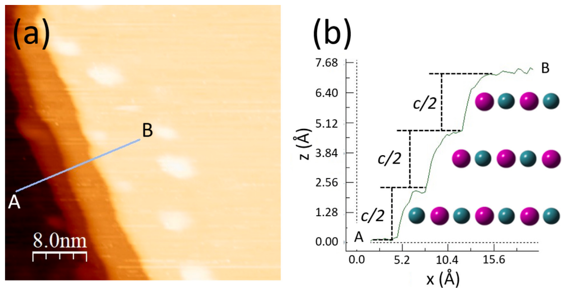
Fig. 10. (a) In-situ UHV-STM image of \text{Mn}_2\text{Sn}/\text{GaN}/\text{Al}_2\text{O}_3 showing atomically smooth terraces and atomic layer height steps. The cross-section line profile A-B at the gray line is displayed in (b); model atoms are not to scale.
