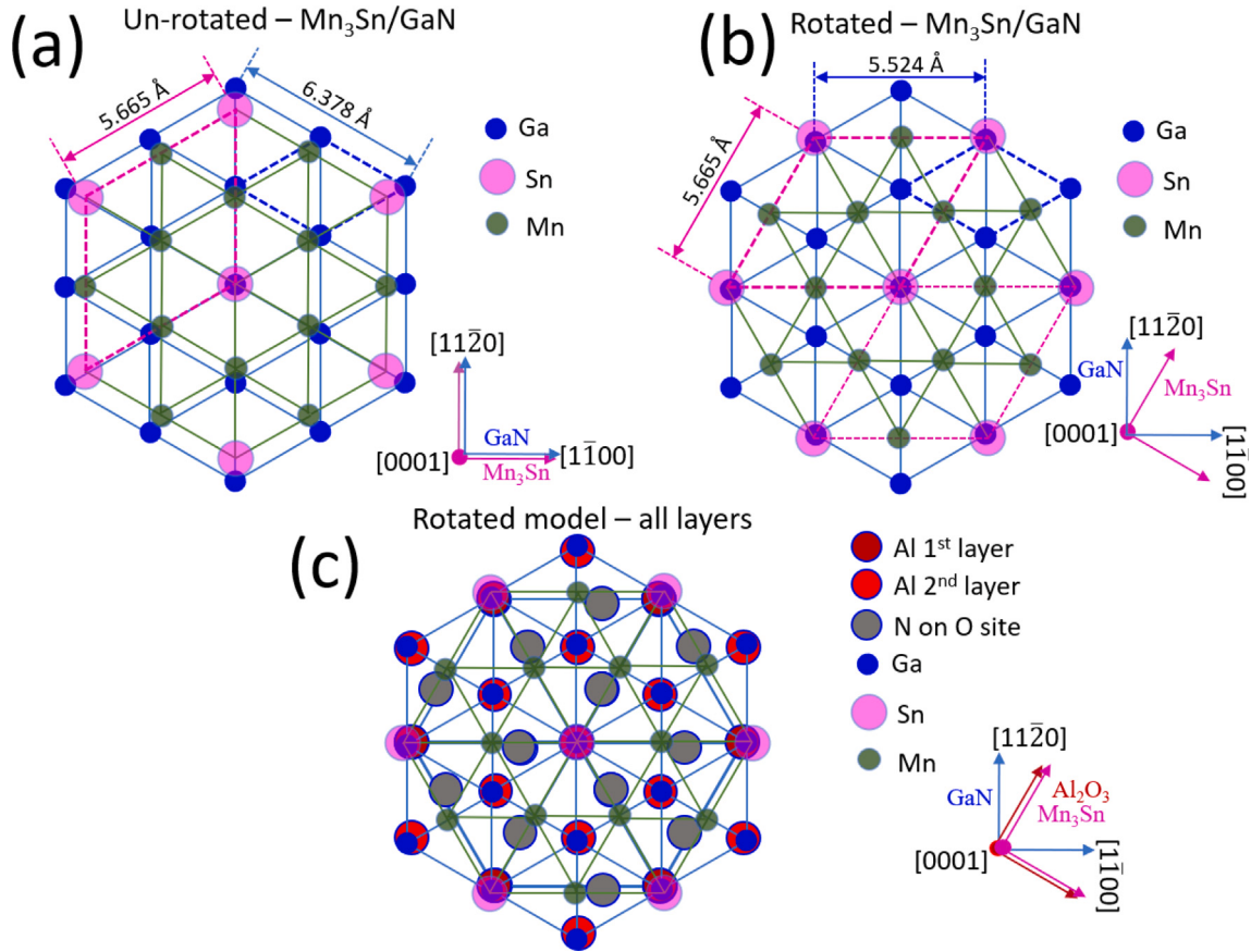
Fig. 3. Growth schematic of Mn 3 Sn (0001) on c -plane GaN with (a) in-plane axes aligned resulting in -11.2\% lattice mismatch with a_{\text{Mn}_3\text{Sn}(0001)} = 5.665 \text{ \AA} and 2 \times a_{\text{GaN}(0001)} = 2 \times 3.189 \text{ \AA} = 6.378 \text{ \AA} ; GaN and Mn 3 Sn surface unit cells are shown by dashed lines; (b) With in-plane 30^\circ rotation on c -plane GaN, reducing the lattice mismatch to +2.63\% ; GaN and Mn 3 Sn surface unit cells are shown by dashed lines; (c) combined schematic lattice overlay of c -plane Mn 3 Sn on GaN on nitridated sapphire.
