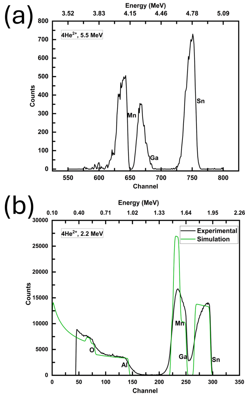
Fig. 8. (a) RBS data at 5.5 MeV showing the separated peaks for Mn, Ga, and Sn; (b) RBS data at 2.2 MeV together with a RUMP simulation.
