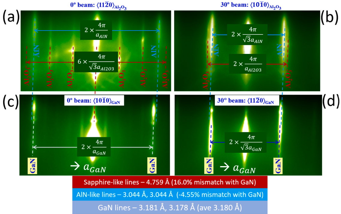
Fig. 2. RHEED patterns before (a,b) and after (c,d) GaN growth on nitridated \text{Al}_2\text{O}_3 (0001). (a,b) RHEED shows 1st-order primary streaks corresponding to original \text{Al}_2\text{O}_3 (0001) (red dashed lines) lattice but also 1st-order AlN-like streaks (cyan dashed lines) indicating a 30° lattice rotation; (c,d) overgrown GaN RHEED streaks slightly closer together compared to the AlN streaks. Reciprocal lattice streak spacings given in terms of inverse lattice constants. (For interpretation of the references to colour in this figure legend, the reader is referred to the web version of this article.)
