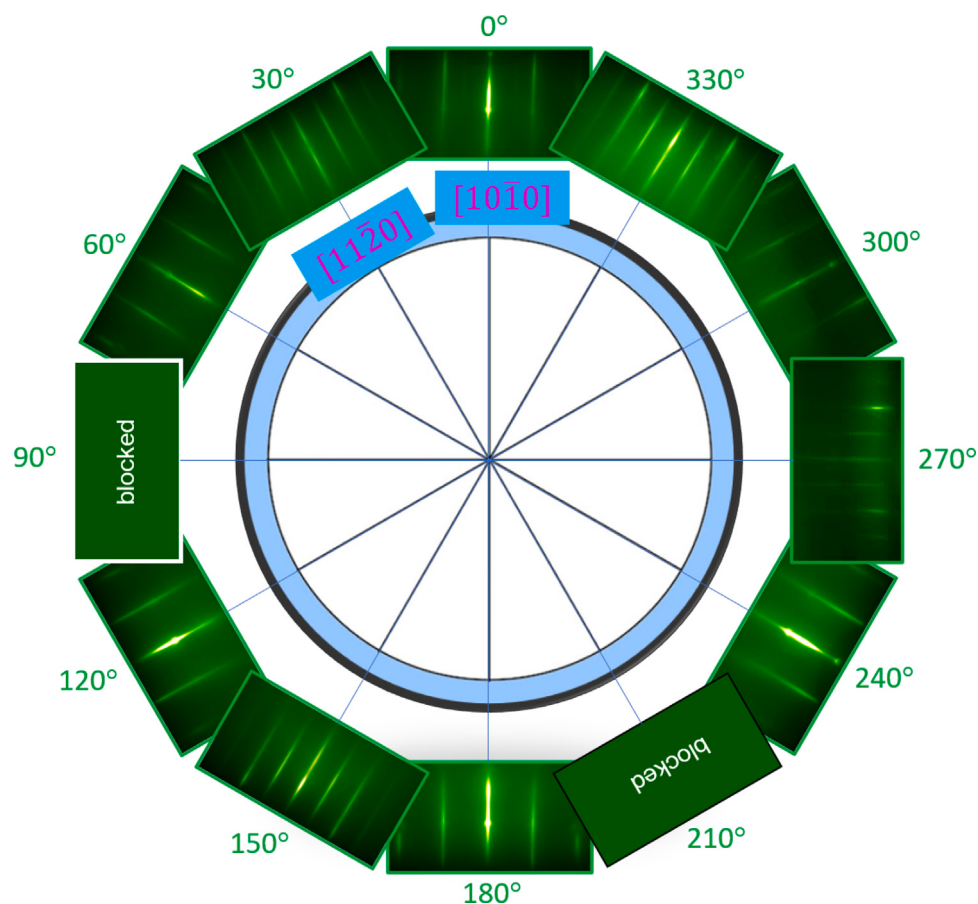
Fig. 6. 360° RHEED azimuth map for \text{Mn}_3\text{Sn} (0001). The patterns exhibit well-defined streaks, indicative of a well-ordered crystalline surface. A clear six-fold rotational symmetry is observed, consistent with the hexagonal crystal structure of \text{Mn}_3\text{Sn} . The primary crystallographic orientations, [11\bar{2}0] and [10\bar{1}0] , are marked for reference. The 90° and 210° azimuths are blocked by the sample holder clips.
