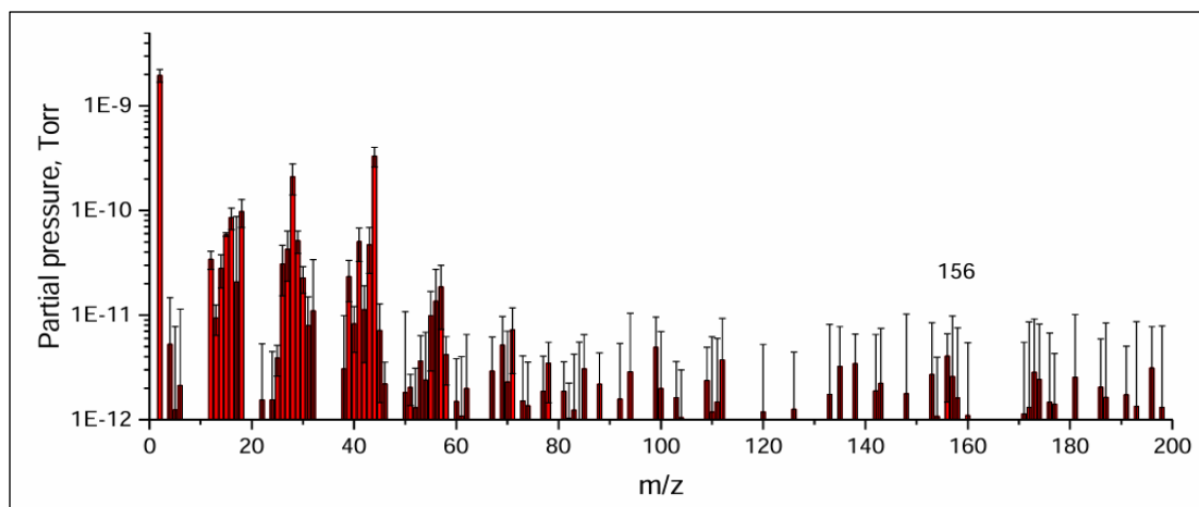
Figure S15. RGA outgassing from aZnMIm films from m/z = 1 - 200 . 156 is the only significant outgassing peak greater than m/z = 100 .
