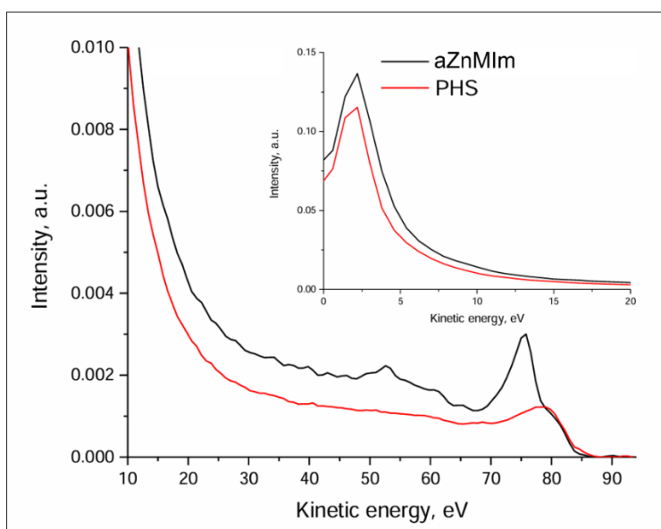
Figure S13. EUV photoelectron spectra comparing aZnMIm to poly(4-hydroxystyrene) (PHS).
