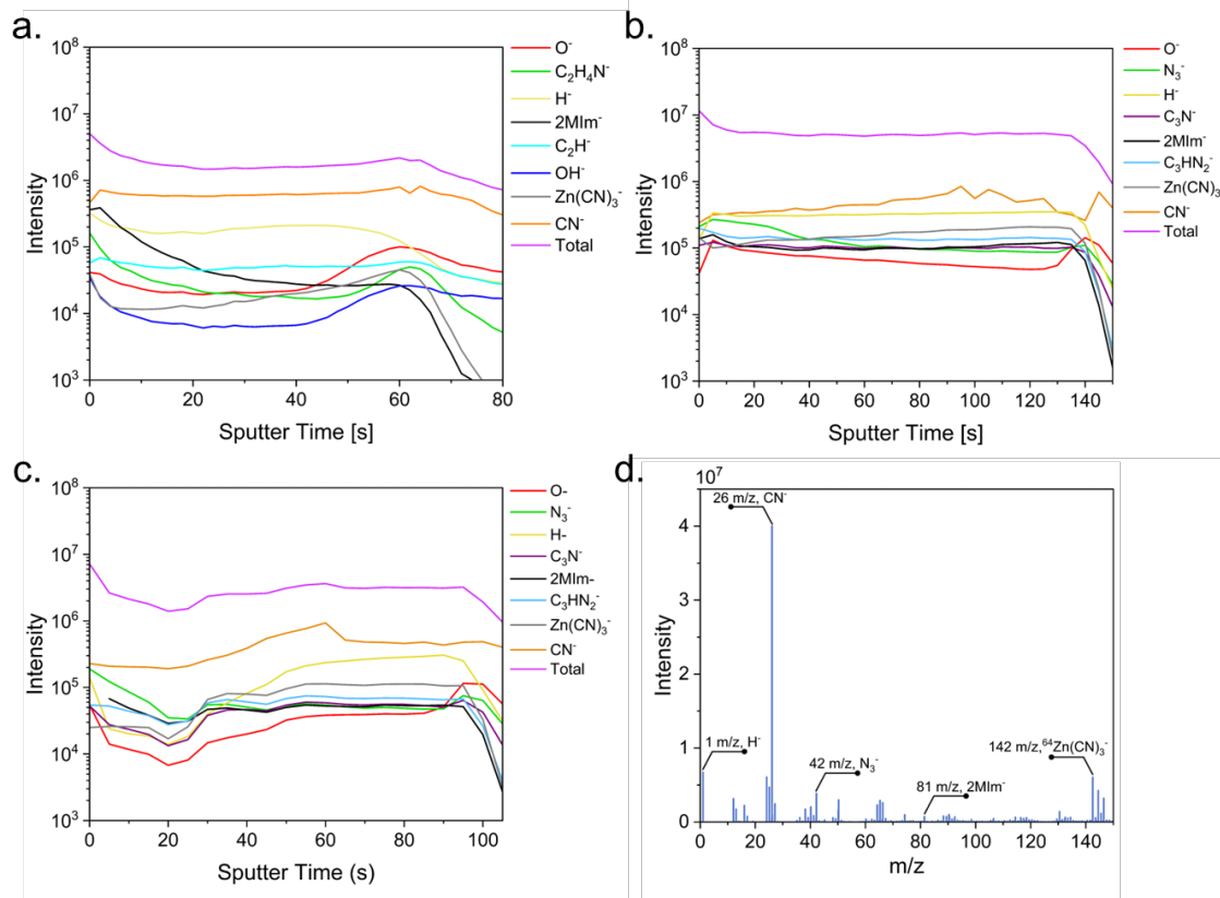
Figure S17. TOF-SIMS depth profiling and sum spectrum. (a) TOF-SIMS depth profile for an as-deposited aZnMIm film. (b) TOF-SIMS depth profile for aZnMIm exposed to an EUV dose of 4036 mJ/cm 2 . (c) TOF-SIMS depth profile for aZnMIm exposed to an EUV dose of 4036 mJ/cm 2 and subsequently developed in water for 15 minutes. (d) TOF-SIMS total-film-depth sum spectrum for the sample in (c).
