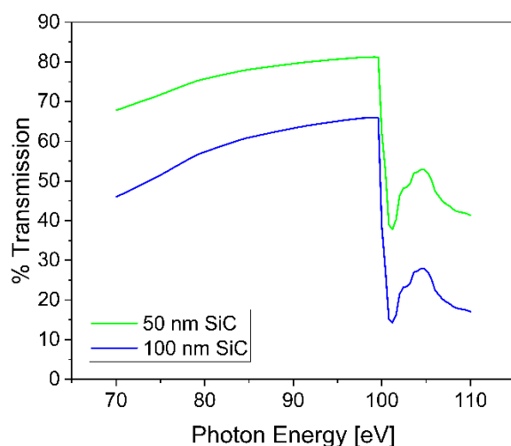
Figure S3. Transmission of SiC membranes. There is ~64% transmission of 92 eV photons through a 100 nm thick SiC membrane. Data was extracted from the CXRO X-ray Database on the X-ray transmission of solids page. 6
