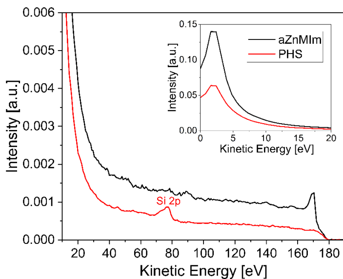
Figure S19. BEUV (6.7 nm) photoelectron spectra comparing aZnMIm to poly(4-hydroxystyrene) (PHS).
