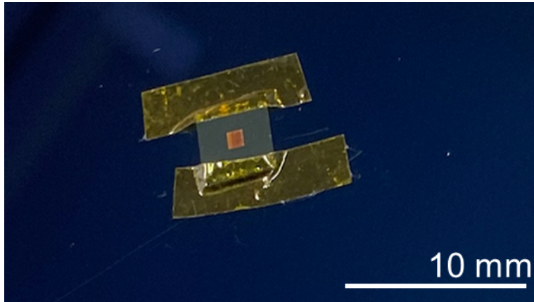
Figure S2. Photomask fabricated by Applied Nanotools Inc. (ANT) taped with Kapton tape to the surface of an aZnM1m photoresist before EUV exposure.
