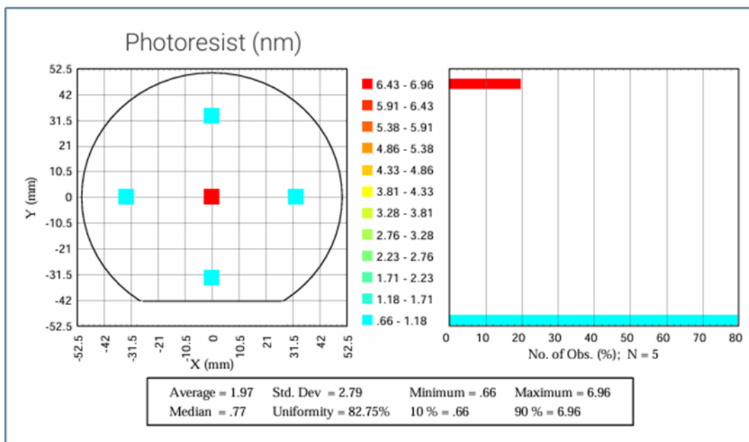
Figure S11. Ellipsometry data taken at Bruker Inc. of an aZnMIm photoresist after development in water for five minutes and 655 \mu\text{M} acetic acid for 1 minute (spot is the one with an exposure dose of 460 \text{mJ}/\text{cm}^2 in Figure 2c). The top panel gives measurements around an EUV exposure spot showing a steep height drop off to the native oxide thickness next to the spot. The bottom panel gives remaining material thickness around the outside edges of the 100 mm wafer in addition to a height measurement at the very center of the wafer. The edges show very clean development with remaining thickness attributed to the native oxide. The center of the wafer indicates some undeveloped photoresist material (thickness of ca. 6 nm) remaining after immersion in DI water and acetic acid.
