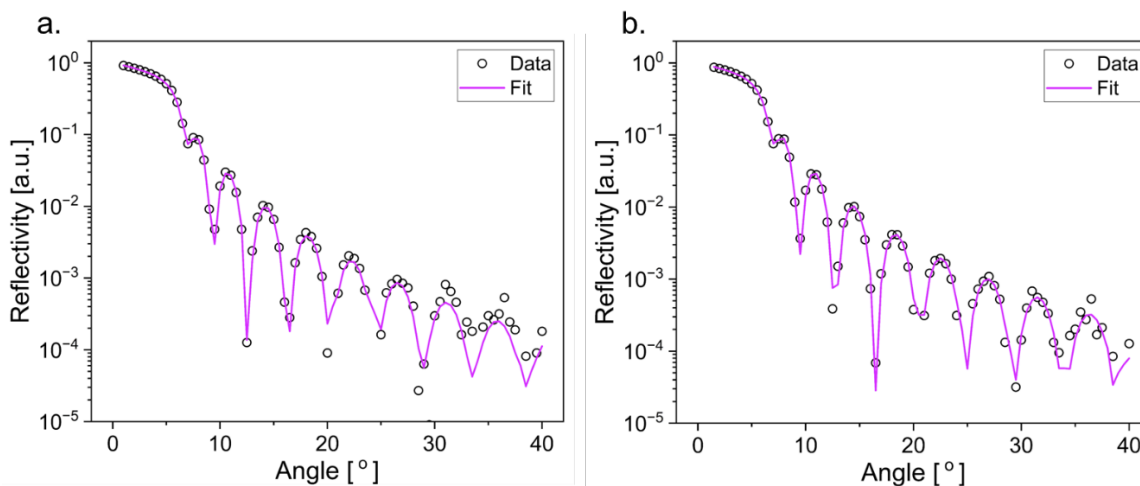
Figure S18. BEUVL reflectometry data obtained experimentally and calculated for a 45 nm thick aZnMIm film to determine BEUV absorption. (a) Reflectometry results at a wavelength of 6.60 nm. (b) Reflectometry results at a wavelength of 6.65 nm.
