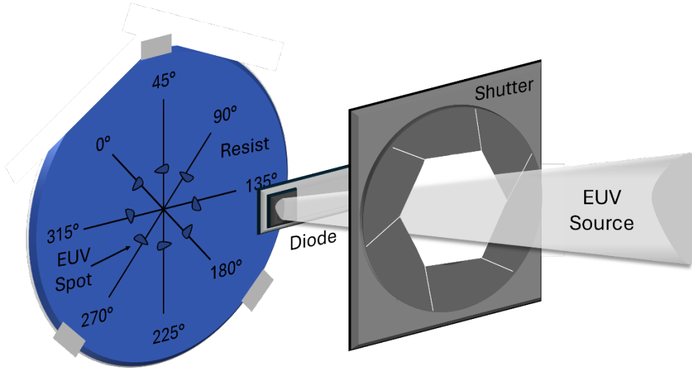
Figure S1. EUV Exposure Schematic showing the shutter open and the diode rotated into measurement position to measure the beam current. This is done both before and after EUV exposure. The current is then averaged before being used to calculate the EUV dose.
