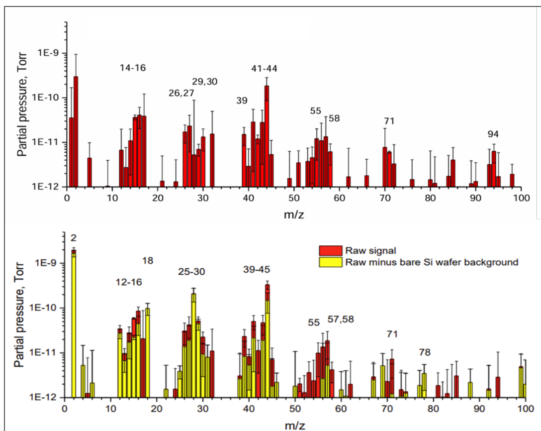
Figure S14. RGA outgassing from a Si wafer (top) and aZnMIm (bottom) before and after subtracting the Si wafer background.
