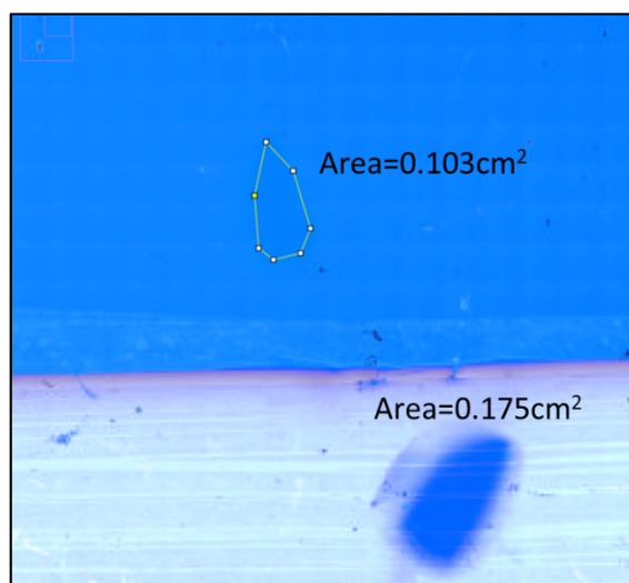
Figure S21. EUV spot area measured and used to calculate EUV dose. The area of the latent image was measured in ImageJ and was used for all EUV dose calculations. The dose in \text{mJ}/\text{cm}^2 is calculated by multiplying the averaged beam current in mA before and after exposure by the exposure time in s and dividing by the area in \text{cm}^2 and a source conversion factor ( 0.09 \text{ mA}/\text{mW} ).
