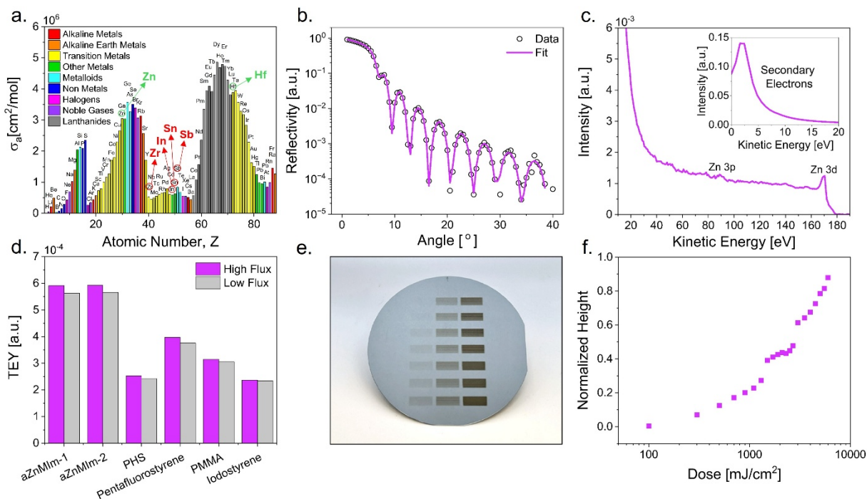
Figure 4. aZnMIm Response to a BEUV wavelength of 6.7 nm. (a) Atomic absorption cross sections at a wavelength of 6.7 nm (185.05 eV). Elements with atomic number from 1 to 88 were plotted using atomic scattering factors from CXRO X-ray database. 106 (b) Reflectometry data obtained experimentally and model fit for a 45 nm thick aZnMIm film to determine BEUV absorption. (c) BEUV photoelectron spectrum of an aZnMIm film showing the distribution of primary and secondary electrons. The inset shows a zoomed in view of the low energy secondary electrons (< 20 eV). (d) TEY for many model photoresist materials at a wavelength of 6.7 nm. Two aZnMIm locations were tested along with PHS, poly(pentafluorostyrene), PMMA, and poly(iodostyrene). (e) BEUV exposure of a 45 nm thick aZnMIm film at doses between 100 – 6000 mJ/cm 2 . Following BEUV, the aZnMIm film was exposed to hfach vapor at 120 °C for 60 seconds and then rinsed with methanol. (f) A contrast curve corresponding to the film in (e) with BEUV exposure spots measured via spectroscopic ellipsometry and then normalized with respect to the original film thickness after MLD.
