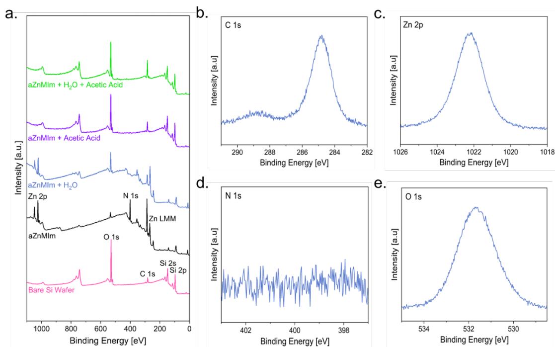
Figure S7. XPS of developed aZnMIm films. (a) Survey scans showing (from bottom to top) a bare Si wafer reference, a 60 nm thick as-deposited aZnMIm film, aZnMIm after development in DI water for 8 minutes, aZnMIm after development in 655 μM acetic acid for 3 minutes, and aZnMIm after development in DI water for 5 minutes and then 655 μM acetic acid for 1 minute. (b-e) High-resolution (b) C 1s (c) Zn 2p (d) N 1s (e) O 1s scans of an aZnMIm film after development in water for 8 minutes.
