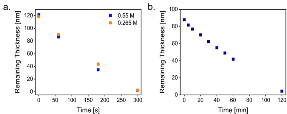
Figure S12. Dissolution of aZnMIm in TMAH and methanol. (a) Dissolution of a ~120 nm thick aZnMIm film in two different concentrations of tetramethylammonium hydroxide (TMAH). (b) Dissolution of a 90 nm thick aZnMIm film in methanol.
