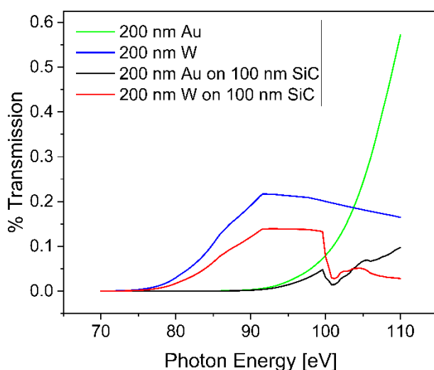
Figure S4. Transmission of metal gratings. Based on the transmission values above, Au was selected for the grating material. There is less than 0.005% transmission of 92 eV photons through the Au gratings on top of the 100 nm thick SiC membrane. Data was extracted from the CXRO X-ray Database on the X-ray transmission of solids page. 6
