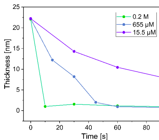
Figure S8. Dissolution of 23 nm thick aZnMIm films in three acetic acid solutions: 0.2M (pH ~2.7), 655 \mu M (pH ~4), and 15.5 \mu M (pH ~5).
