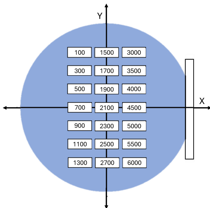
Figure S20. BEUV (6.7 nm) exposure doses in \text{mJ}/\text{cm}^2 for the aZnMIm film shown in Figure 4e.
