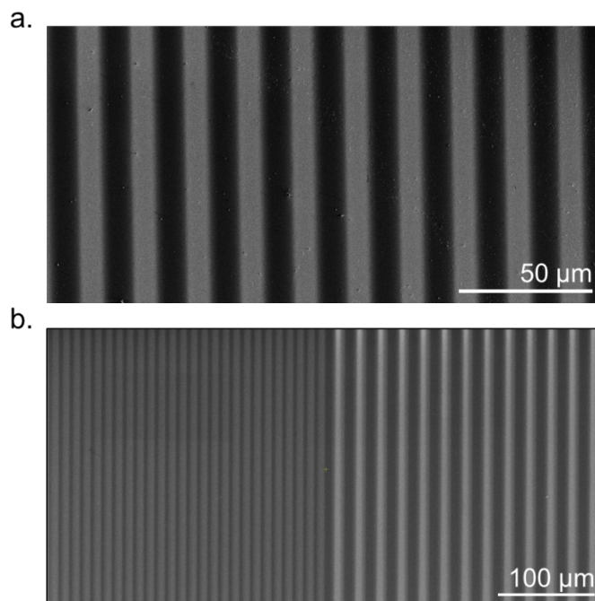
Figure S5. Line patterns fabricated with the EUV Tech Inc. EUV Flood source using a coarse grating photomask fabricated by Applied Nanotools Inc. (ANT). (a) 1:1 10 \mu\text{m} line spacing patterns exposed to an EUV dose of \sim 216 \text{ mJ/cm}^2 and developed in DI water for 5 minutes followed by 2 minutes in 655 \mu\text{M} acetic acid and a methanol rinse. (b) 1:1 5 (left) and 10 (right) \mu\text{m} line spacing patterns exposed to an EUV dose of \sim 120 \text{ mJ/cm}^2 and developed in DI water for 10 minutes. The patterns in (b) are not completely developed and have \sim 30 \text{ nm} of residual material between the lined areas.
