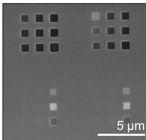
Figure S9. Electron beam patterning of 22 nm thick aZnMIm with development in 655 \mu M acetic acid for 60 seconds followed by a methanol rinse. The bottom two 3 x 3 dose matrices range from 50 to 1000 \mu C/cm 2 while the top left is 1 to 20 mC/cm 2 and the top right is 0.5 to 10 mC/cm 2 .
