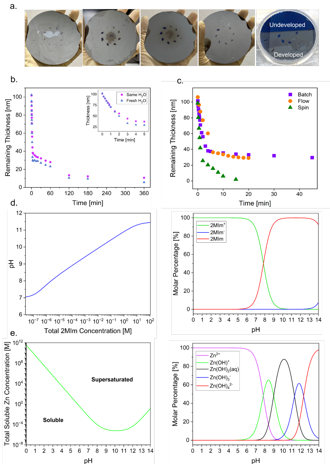
Figure S6. Dissolution of as-deposited aZnMIm films in water. (a) Development of aZnMIm films in water showing uneven development, variation from sample to sample, delamination, and peeling of remaining material. (b) Dissolution of ~100 nm thick aZnMIm in water revealing two stage dissolution
