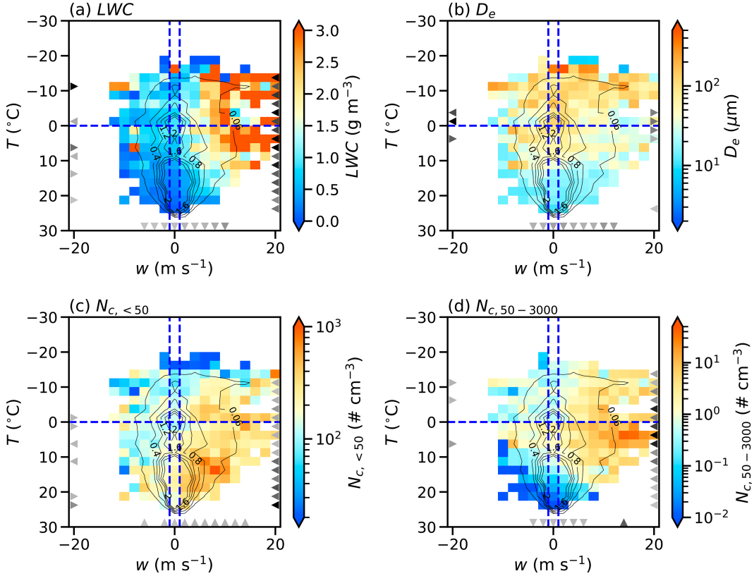
FIG. 5. Variation in cloud properties (a) LWC, (b) D_e , (c) N_{c, <50} , and (d) N_{c, 50-3000} in the w - T parameter space for 16853 samples where N_{c, <50} \geq 10 \text{ cm}^{-3} . The bin sizes for computing the variations for w and T are 2 \text{ m s}^{-1} and 2.5^\circ\text{C} , respectively. Colored shading areas represent the mean value of each cloud property within each bin. Contours indicate the sample percentage distribution at levels of 0.06%, 0.4%, 0.8%, 1.2%, 1.6%, and 2%. The triangles along the x axis represent the sign of regression coefficients (slopes) between cloud properties and T in each w bin: upward-pointing triangles ( \blacktriangle ) indicate the positive slopes (cloud properties increase as T increases) and downward-pointing triangles ( \blacktriangledown ) indicate the negative slopes (cloud properties decrease as T increases). The triangles along the left y axis represent the sign of regression coefficients between cloud properties and negative w in each T bin, and the triangles along the right y axis correspond to the regression coefficients between cloud properties and positive w : rightward-pointing triangles ( \blacktriangleright ) indicate the negative slopes (cloud properties decrease as w increases) and leftward-pointing triangles ( \blacktriangleleft ) indicate the positive slopes (cloud properties increase as w increases). Shading of every triangle indicates the magnitude of the slope (darker = larger |slope|). Only regression coefficients with sample sizes greater than 30 and a statistical significance level of 0.05 are shown. The horizontal blue dashed line indicates 0^\circ\text{C} , and the vertical blue dashed lines denote -1 and 1 \text{ m s}^{-1} in each panel.
