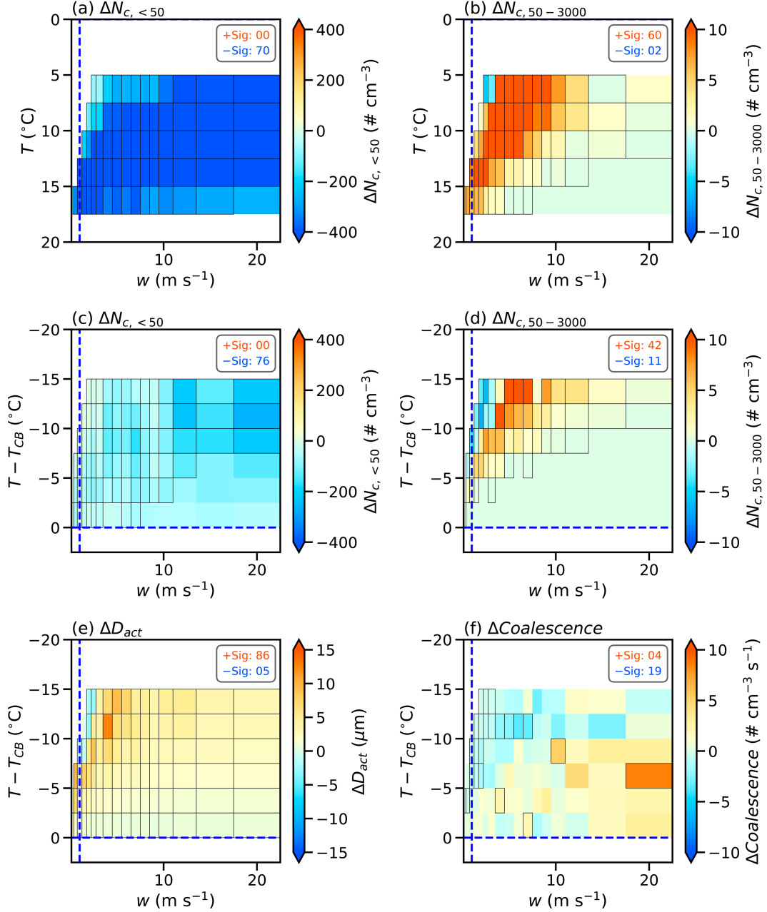
FIG. 9. Differences (shaded pixels) in mean cloud properties or process rates between warmer ( 21^{\circ}\text{C} \leq T_{CB} \leq 23^{\circ}\text{C} ) and colder ( 15^{\circ}\text{C} \leq T_{CB} \leq 17^{\circ}\text{C} ) cloud-base sample groups in the (a),(b) w - T and (c)-(f) w -( T - T_{CB} ) parameter spaces for (a),(c) N_{c, < 50} , (b),(d) N_{c, 50 - 3000} , (e) diameter of activated droplets D_{act} , and (f) droplet collision-coalescence rate. Pixels outlined with black boxes represent the bins where the sample size is at least 10 in both groups and the mean differences are statistically significant at the 0.05 level based on a t test. The total number of significant positive (orange) and negative (blue) differences is displayed in the top-right corner of each panel. The bin size for T or T - T_{CB} is 2.5^{\circ}\text{C} . The bin center for w corresponds to the prescribed vertical velocities in the parcel model. The horizontal blue dashed line indicates 0^{\circ}\text{C} , and the vertical blue dashed line denotes 1 \text{ m s}^{-1} in each panel.
