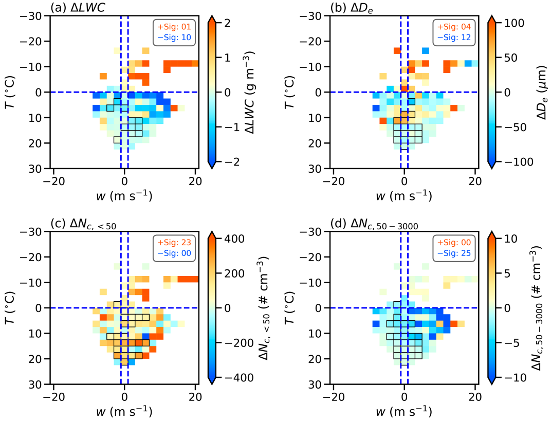
FIG. 8. Differences (shaded pixels) in mean cloud properties between the groups of the highest and lowest 20th percentile of entire M_{\text{aer}} samples in the w - T parameter space for (a) LWC, (b) D_e , (c) N_{c, <50} , and (d) N_{c, 50-3000} . The highest 20th percentile group of M_{\text{aer}} has a mean of 6.80 \mu\text{g m}^{-3} with a standard deviation of 3.10 \mu\text{g m}^{-3} , and the lowest 20th percentile group has a mean of 1.95 \mu\text{g m}^{-3} with a standard deviation of 0.23 \mu\text{g m}^{-3} . Pixels outlined with black boxes represent the bins where the sample size is at least 10 in both groups, and the mean differences are statistically significant at the 0.05 level based on a t test. The total number of significant positive (orange) and negative (blue) differences is displayed in the top-right corner of each panel. The bin sizes for w and T are 2 \text{ m s}^{-1} and 2.5^\circ\text{C} , respectively. The horizontal blue dashed line indicates 0^\circ\text{C} , and the vertical blue dashed lines denote -1 and 1 \text{ m s}^{-1} in each panel.
