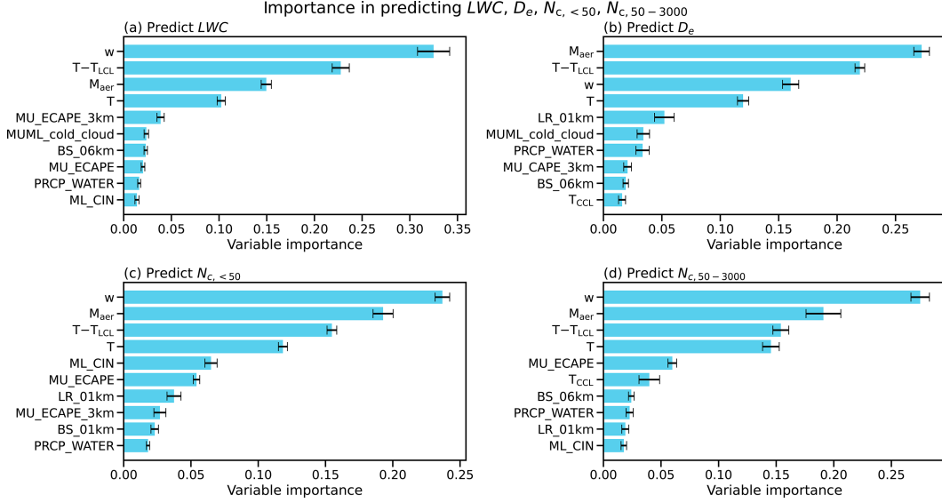
FIG. 6. As in Fig. 4, but for random forest models trained with an additional environmental parameter T - T_{LCL} .
