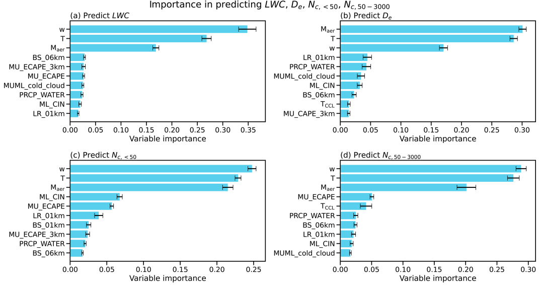
FIG. 4. Importance of top-10 environmental parameters in predicting (a) LWC , (b) D_e , (c) cloud droplet number concentration for D_{\text{max}} < 50 \mu\text{m} ( N_{c, < 50} ), and (d) cloud droplet number concentration for 50 \mu\text{m} \leq D_{\text{max}} \leq 3000 \mu\text{m} ( N_{c, 50-3000} ) using a random forest model. The horizontal bars represent the mean relative importance of various environmental variables for each cloud property, with error bars showing the standard deviation of the importance scores over 100 iterations of Monte Carlo cross validation.
