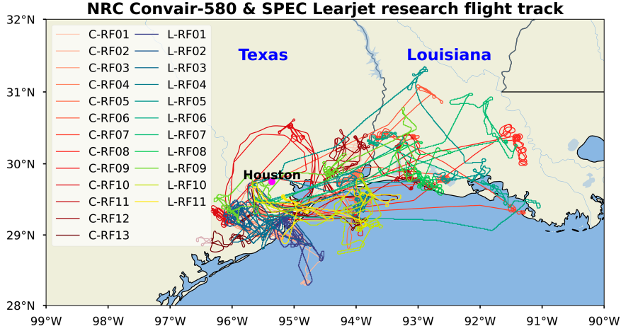
FIG. 1. Research flight tracks of NRC Convair-580 (C-RF01–C-RF13) and SPEC Learjet (L-RF01–L-RF11) during the ESCAPE field campaign.
