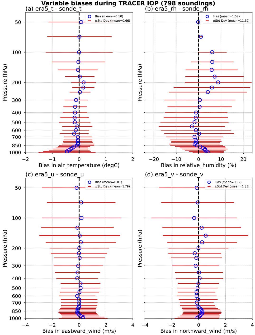
FIG. 2. Differences in (a) air temperature ( ^{\circ}\text{C} ), (b) relative humidity (%), (c) eastward wind ( u ; \text{m s}^{-1} ), and (d) northward wind ( v ; \text{m s}^{-1} ) between the ERA5 and balloon-borne soundings during the TRACER IOP. Blue circles indicate the mean bias at each level, and red bars represent the \pm 1 standard deviation.
