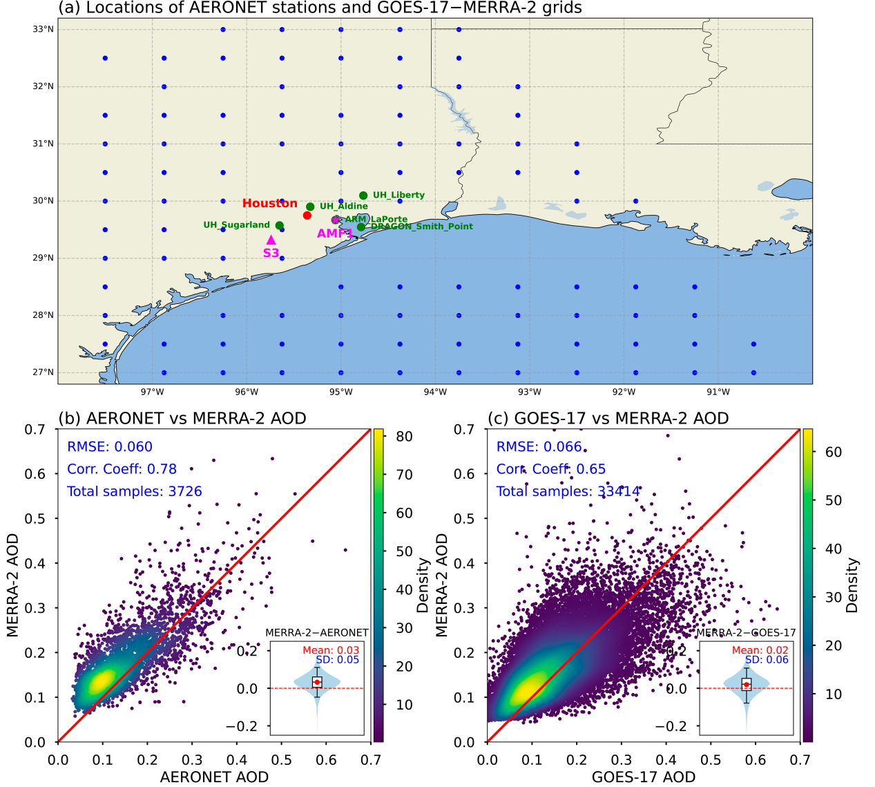
FIG. 3. Comparison of AOD at 550 nm between MERRA-2, AERONET, and GOES-17 datasets during the TRACER IOP. (a) Locations of AERONET stations (green dots) and grid cells for the comparison between GOES-17 and MERRA-2 (blue dots). Scatterplot of (b) AERONET AOD ( x axis) vs MERRA-2 AOD ( y axis) and (c) GOES-17 AOD ( x axis) vs MERRA-2 AOD ( y axis) with density coloring. In (b) and (c), the color intensity of the scatter points indicates the data point density as estimated by a Gaussian kernel density estimate. The red line represents the 1:1 line. Key statistical metrics including RMSE, correlation coefficient, and total number of samples are annotated on each plot. The inset plot shows the distribution of difference [MERRA-2 minus AERONET in (a) and MERRA-2 minus GOES-17 in (b)] with a violin plot and box plot. The box plot indicates the 5th, 25th, 50th (median), 75th, and 95th percentiles. The mean difference (red dot and annotation) and standard deviation (blue annotation) are also highlighted.
