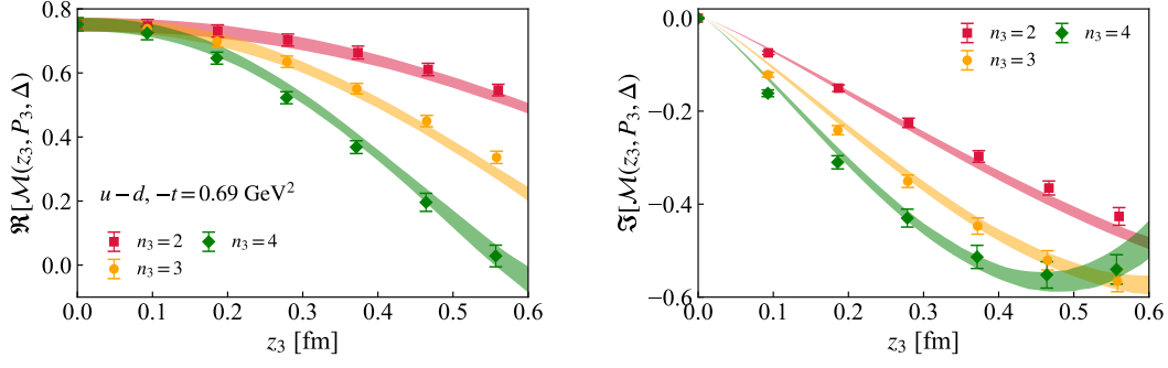
Figure 6. The ratio scheme renormalized iso-vector matrix elements for the case with momentum transfer -t = 0.69 \text{ GeV}^2 are shown as a function of z_3 for three different values of P_3 . The real part (left panel) and imaginary part (right panel) are both shown. The bands are reconstructed from the fit with z_3 \in [2a, 6a] including the NLO matching kernels.
